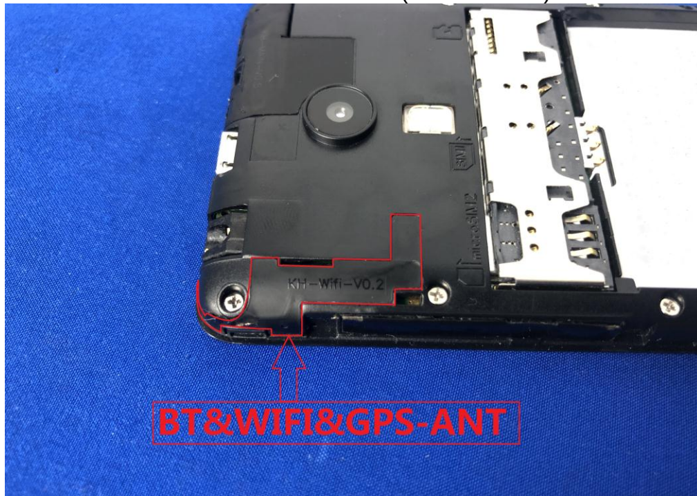
Bluetooth and WIFI ant 1(KH-WiFi-V0.2)
