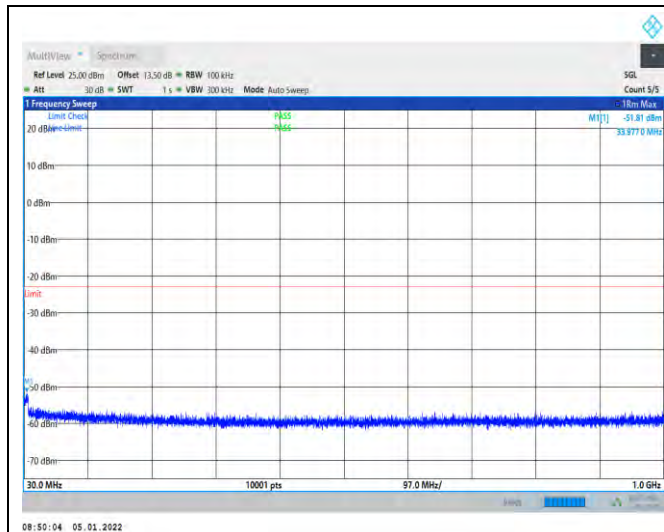
1-N66-PC3-15-40-M-4-DFT-QPSK-Edge_1RB_Left-1 @0-30-1000--51.81--23-PASS
