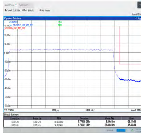
1-N66-PC3-15-5-H-6-CP-QPSK-Outer_Full-2 5@0-Ant1-seegraph-PASS-see graph
