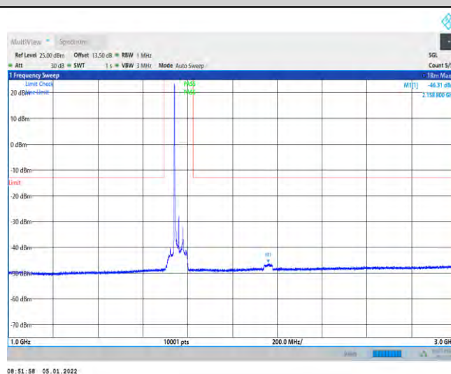
1-N66-PC3-15-40-H-4-DFT-QPSK-Edge_1RB_Left-1@ -1000-3000--46.31--13-PASS
