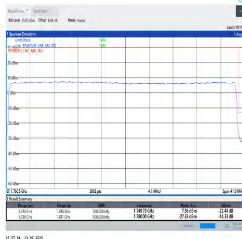
1-N66-PC3-15-40-H-3-DFT-PI2BPSK-Outer_Full-216@0-Ant1-seegraph-PASS-see graph
