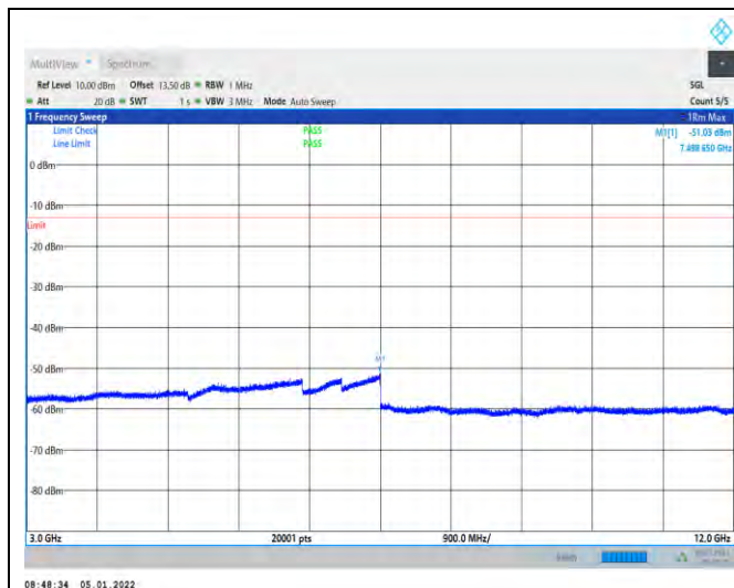
1-N66-PC3-15-40-L-4-DFT-QPSK-Edge_1RB_Left-1 @0-3000-12000--51.03--13-PASS
