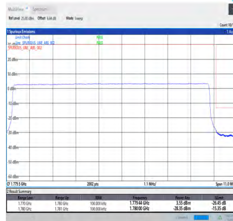
1-N66-PC3-15-10-H-6-CP-QPSK-Outer_Full-52@0-Ant1-seegraph-PASS-see graph
