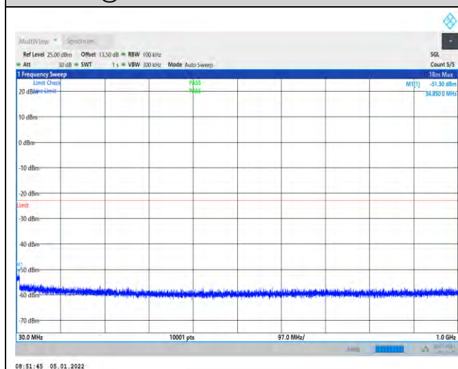
1-N66-PC3-15-40-H-4-DFT-QPSK-Edge_1RB_Left-1 @0-30-1000--51.30--23-PASS
