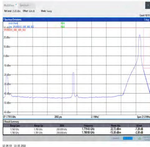
1-N66-PC3-15-20-H-5-CP-QPSK-Edge_1RB_Right-1@105-Ant1-seegraph-PASS-see graph
