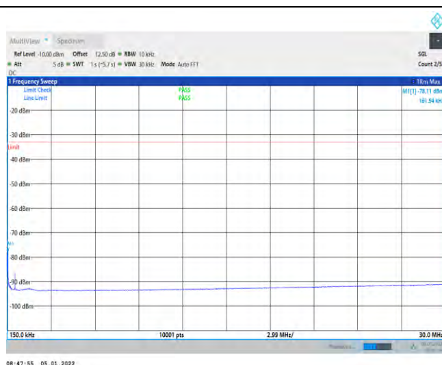
1-N66-PC3-15-40-L-4-DFT-QPSK-Edge_1RB_Left-1@0 -0.15-30--78.11--33-PASS
