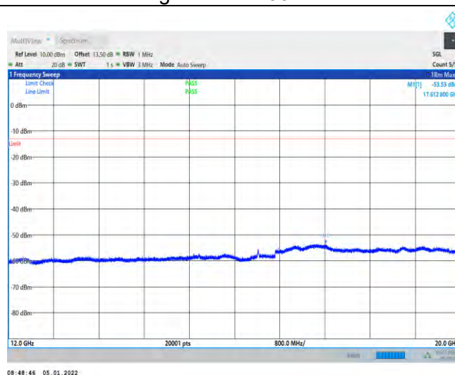
1-N66-PC3-15-40-L-4-DFT-QPSK-Edge_1RB_Left-1@0 -12000-20000--53.53--13-PASS
