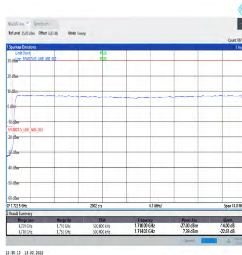
1-N66-PC3-15-40-L-3-DFT-PI2BPSK-Outer_Full-216@0-Ant1-seegraph-PASS-see graph
