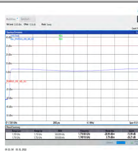
1-N66-PC3-15-40-L-6-CP-QPSK-Outer_Full-216@0-Ant1-seegraph-PASS-see graph
