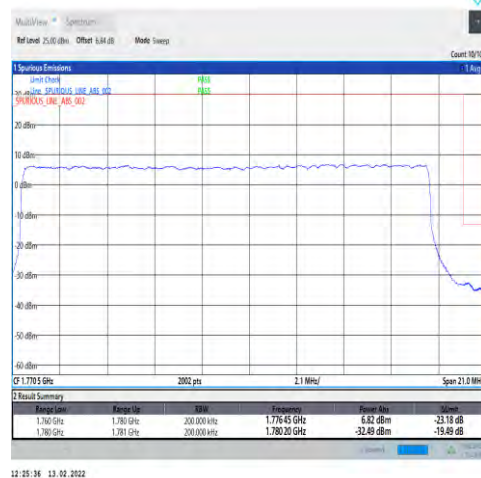
1-N66-PC3-15-20-H-3-DFT-PI2BPSK-Outer_Full-100@0-Ant1-seegraph-PASS-see graph
