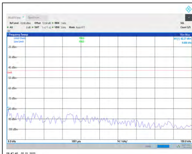
1-N66-PC3-15-40-L-4-DFT-QPSK-Edge_1RB_Left-1 @0-0.009-0.15--82.27--43-PASS
