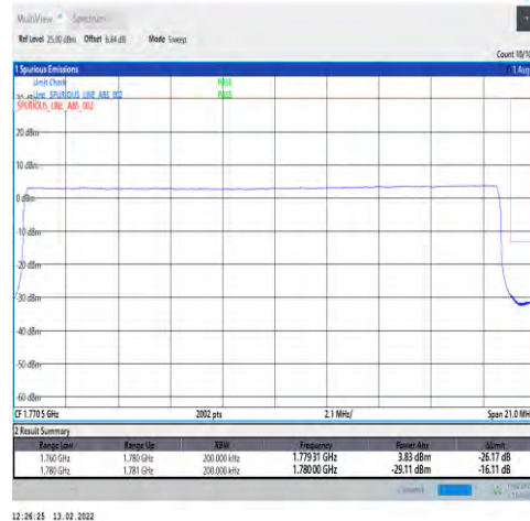
1-N66-PC3-15-20-H-6-CP-QPSK-Outer_Full-106@0-Ant1-seegraph-PASS-see graph
