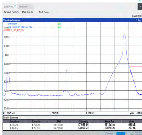
1-N66-PC3-15-10-H-2-DFT-PI2BPSK-Edge_1RB_Right-1@51-Ant1-seegraph-PASS-see graph
