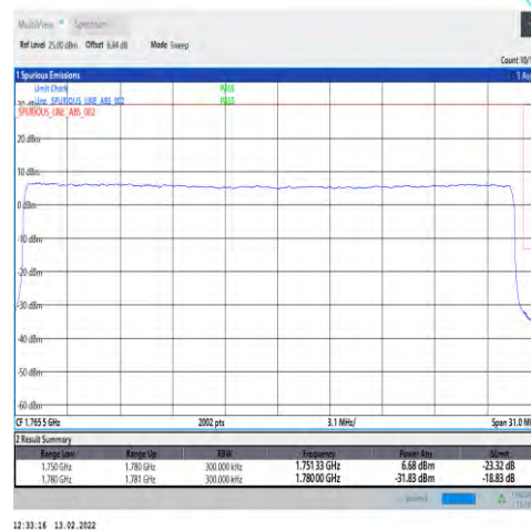
1-N66-PC3-15-30-H-3-DFT-PI2BPSK-Outer_Full-160@0-Ant1-seegraph-PASS-see graph
