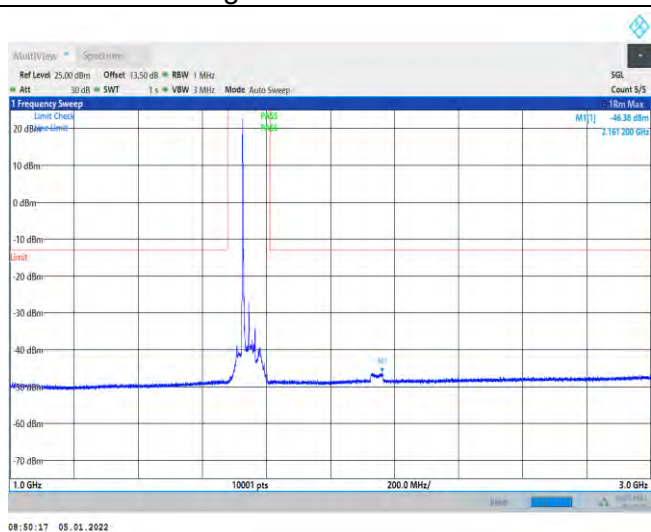
1-N66-PC3-15-40-M-4-DFT-QPSK-Edge_1RB_Left-1@ -1000-3000--46.38--13-PASS
