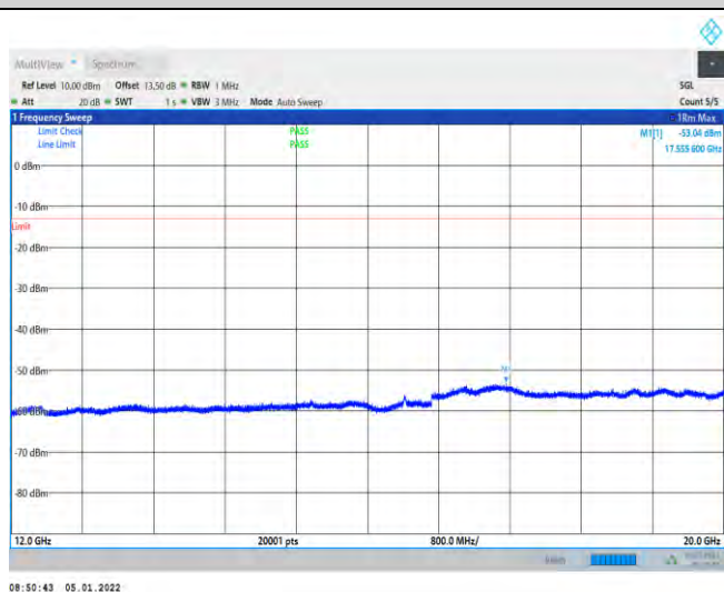
1-N66-PC3-15-40-M-4-DFT-QPSK-Edge_1RB_Left-1@ -12000-20000--53.04--13-PASS
