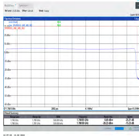
1-N66-PC3-15-40-H-6-CP-QPSK-Outer_Full-216@0-Ant1-seegraph-PASS-see graph
