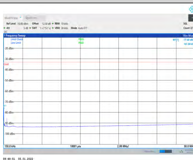
1-N66-PC3-15-40-M-4-DFT-QPSK-Edge_1RB_Left-1@0 -0.15-30--77.40--33-PASS
