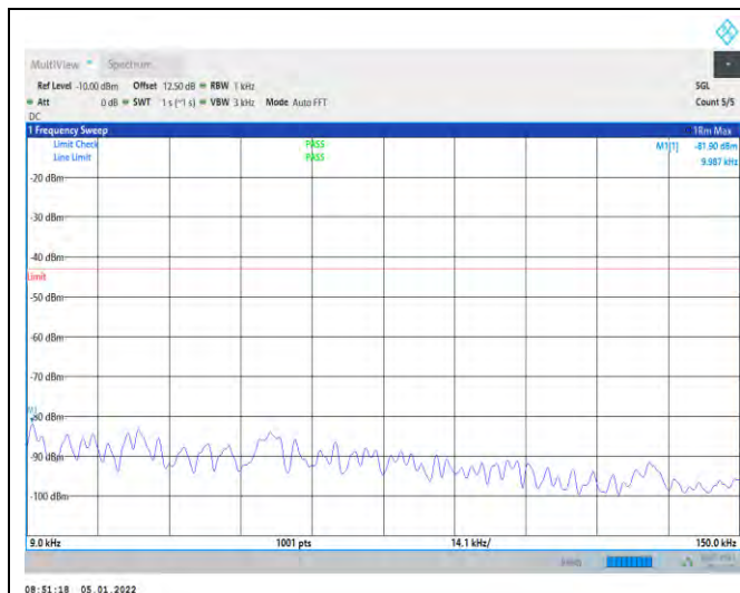
1-N66-PC3-15-40-H-4-DFT-QPSK-Edge_1RB_Left-1 @0-0.009-0.15--81.90--43-PASS
