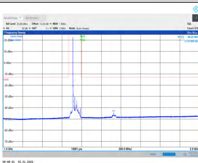
1-N66-PC3-15-40-L-4-DFT-QPSK-Edge_1RB_Left-1@0 -1000-3000--46.20--13-PASS
