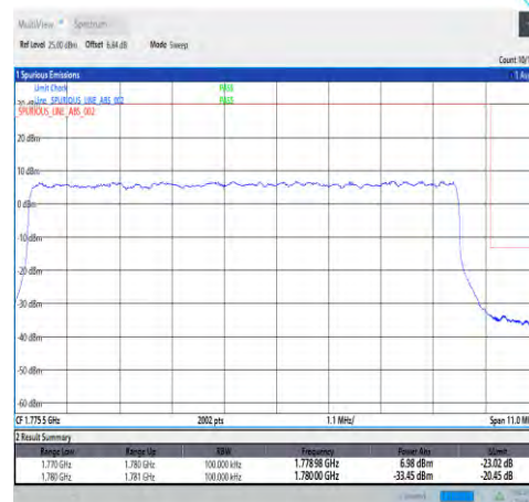
1-N66-PC3-15-10-H-3-DFT-PI2BPSK-Outer_Full-50@0-Ant1-seegraph-PASS-see graph
