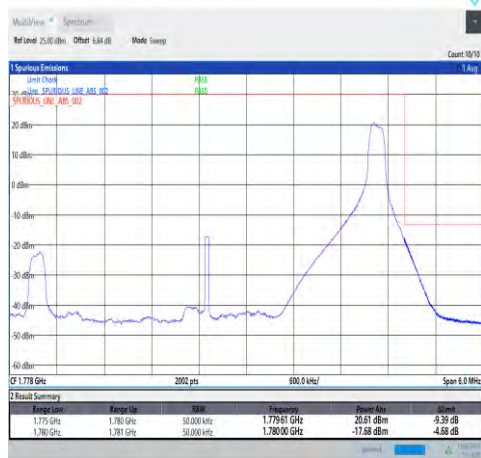
1-N66-PC3-15-5-H-2-DFT-PI2BPSK-Edge_1 RB_Right-1@24-Ant1-seegraph-PASS-see graph
