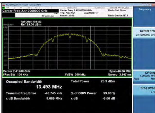
6 dB Bandwidth plot (802.11g-CH 1)
