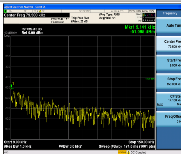
Band2_5MHz_QPSK_18625_1RB#0_0.009~0.15_0.009~0.15
