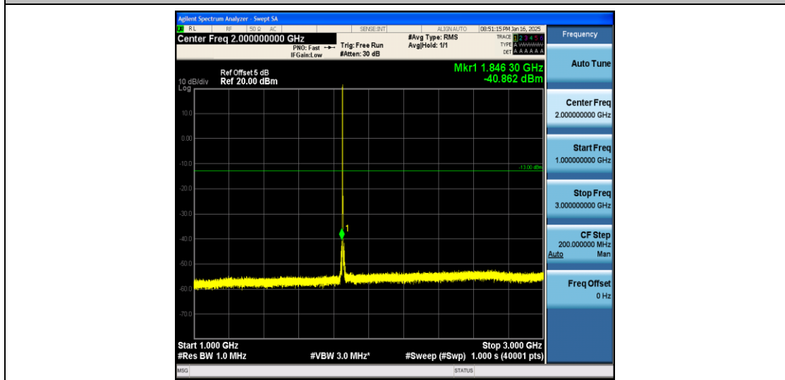
Band2_1.4MHz_16QAM_18607_1RB#0_1000~3000_1000~3000
