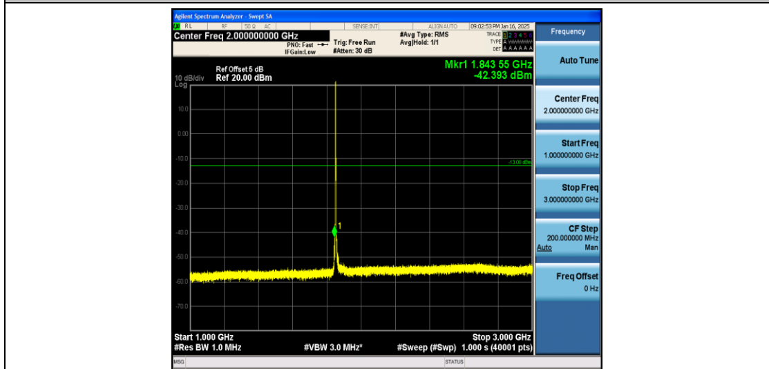
Band2_3MHz_QPSK_18615_1RB#0_1000~3000_1000~3000
