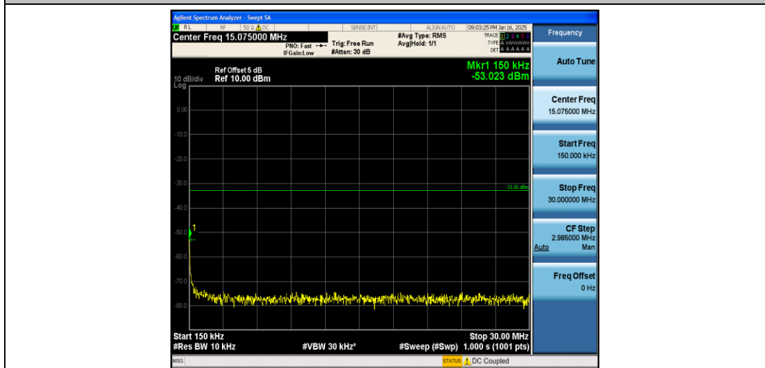
Band2_3MHz_16QAM_18615_1RB#0_0.15~30_0.15~30
