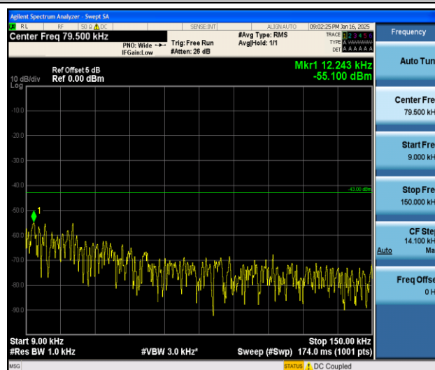
Band2_3MHz_QPSK_18615_1RB#0_0.009~0.15_0.009~0.15
