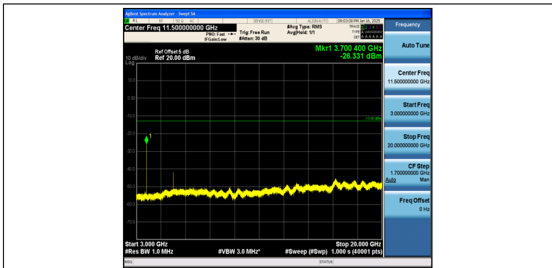
Band2_3MHz_QPSK_18615_1RB#0_3000~20000_3000~20000
