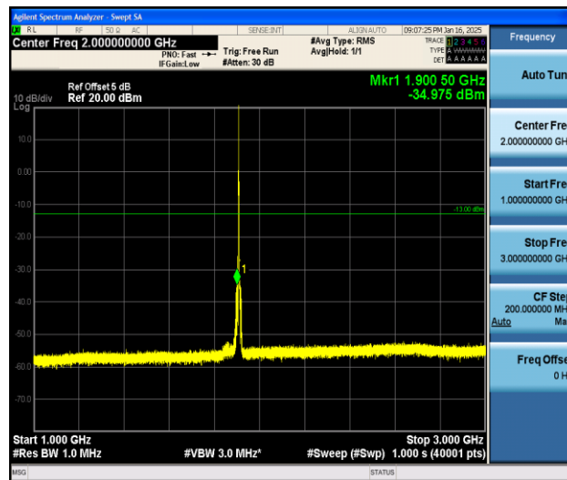
Band2_3MHz_16QAM_19185_1RB#0_1000~3000_1000~3000
