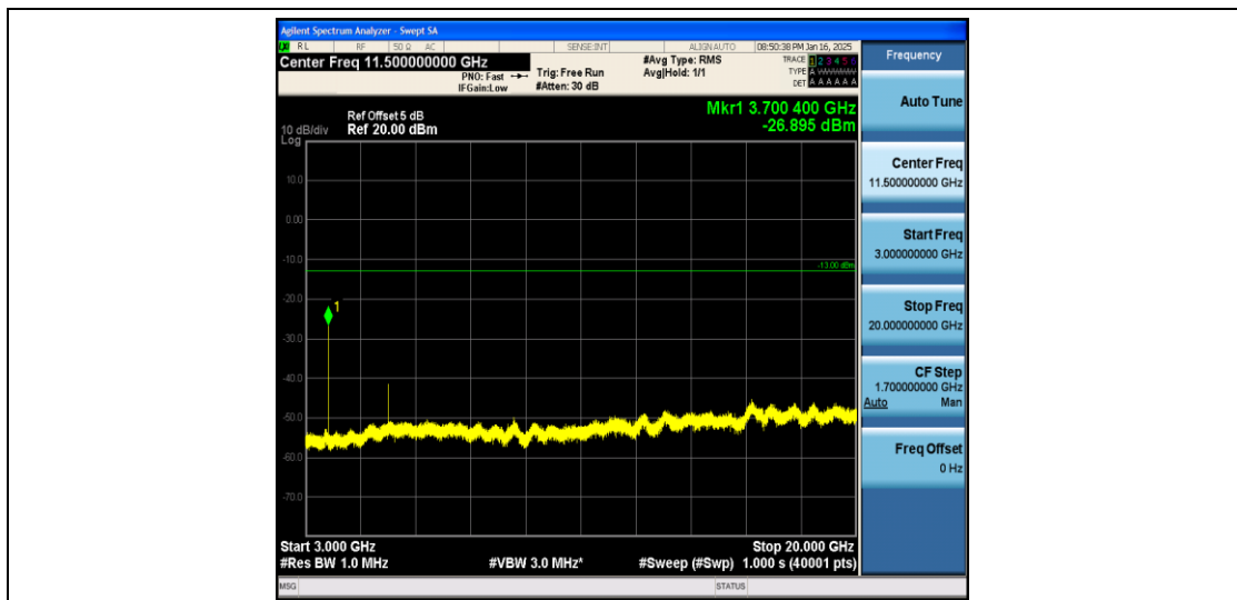
Band2_1.4MHz_QPSK_18607_1RB#0_3000~20000_3000~20000
