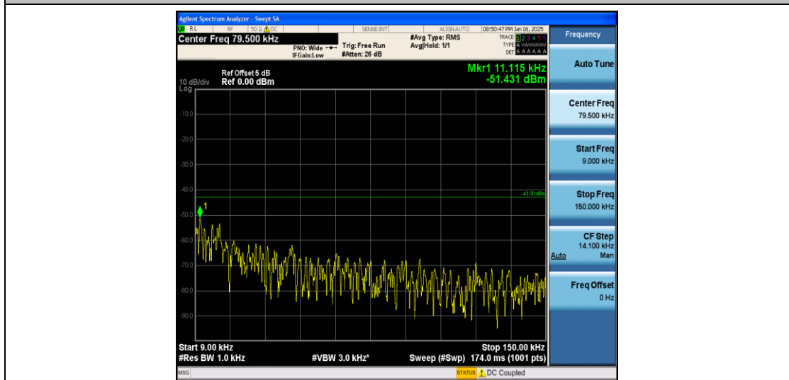
Band2_1.4MHz_16QAM_18607_1RB#0_0.009~0.15_0.009~0.15
