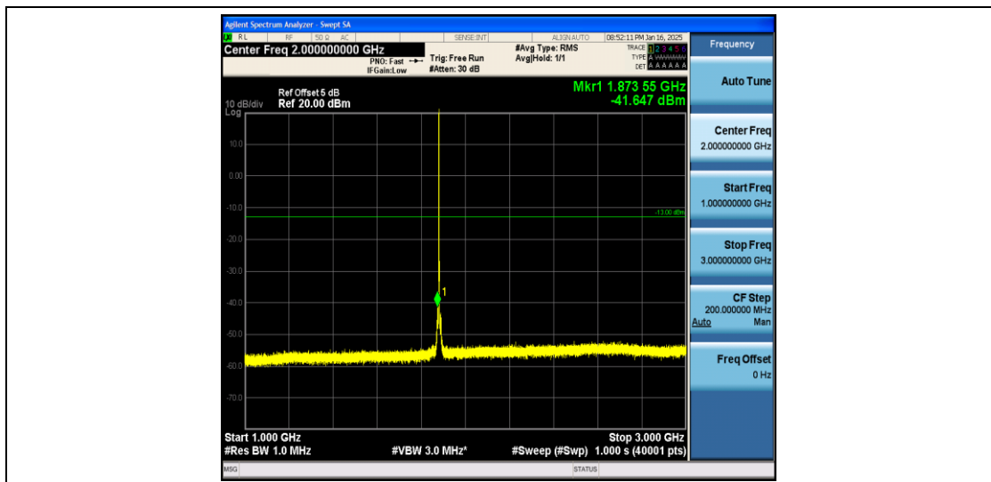
Band2_1.4MHz_QPSK_18900_1RB#0_1000~3000_1000~3000
