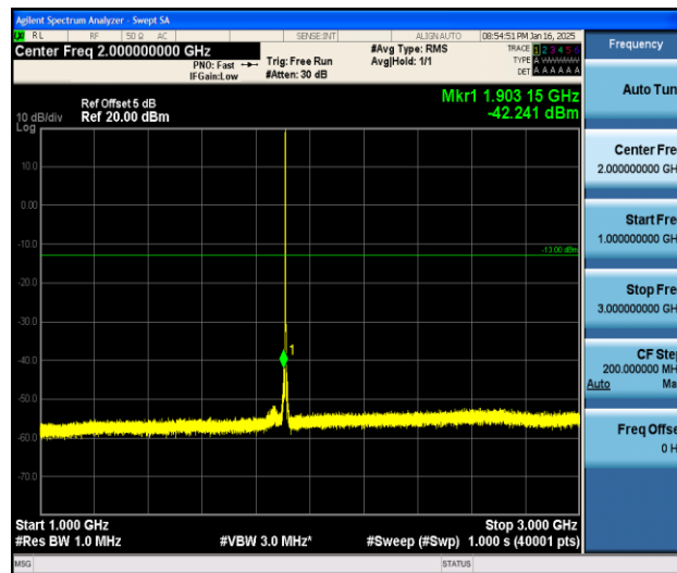
Band2_1.4MHz_16QAM_19193_1RB#0_1000~3000_1000~3000
