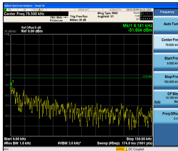
Band2_1.4MHz_QPSK_19193_1RB#0_0.009~0.15_0.009~0.15
