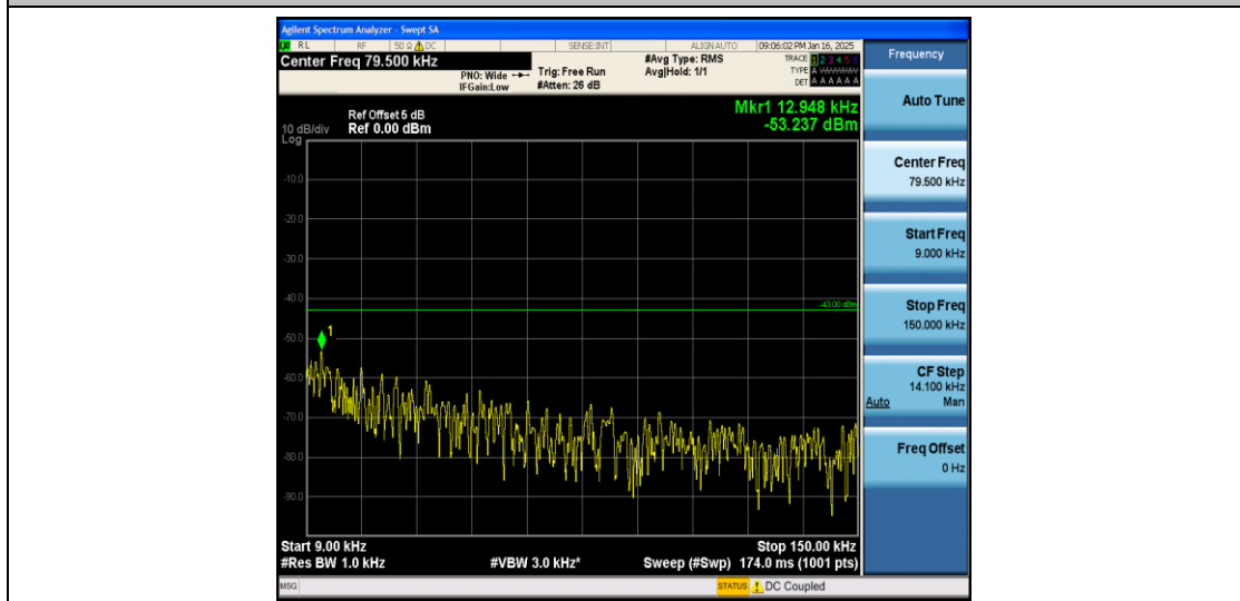
Band2_3MHz_QPSK_19185_1RB#0_0.009~0.15_0.009~0.15
