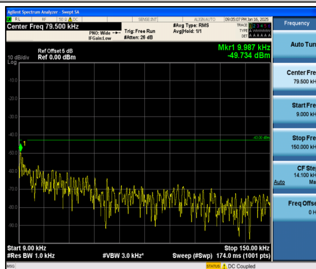
Band2_3MHz_16QAM_18900_1RB#0_0.009~0.15_0.009~0.15
