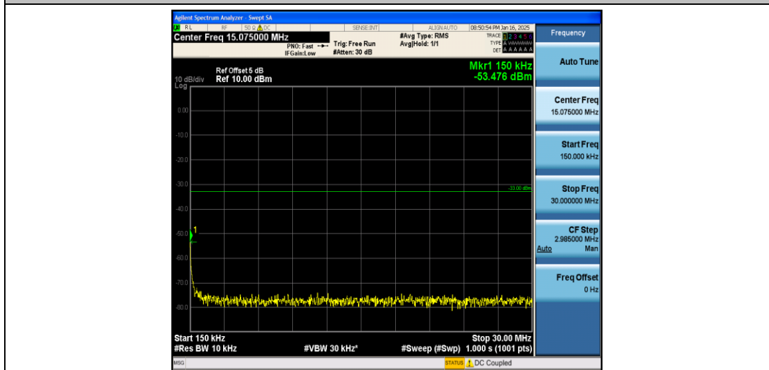
Band2_1.4MHz_16QAM_18607_1RB#0_0.15~30_0.15~30
