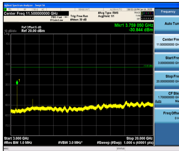
Band2_1.4MHz_16QAM_18900_1RB#0_3000~20000_3000~20000
