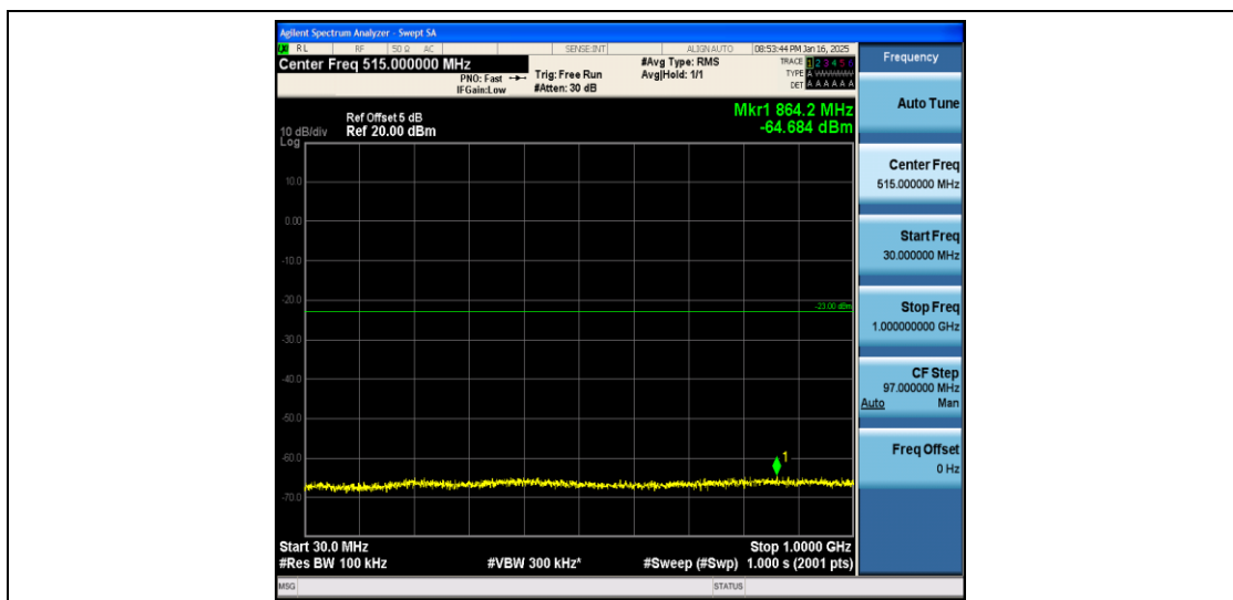
Band2_1.4MHz_QPSK_19193_1RB#0_30~1000_30~1000
