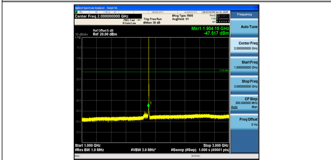
Band2_1.4MHz_QPSK_19193_1RB#0_1000~3000_1000~3000
