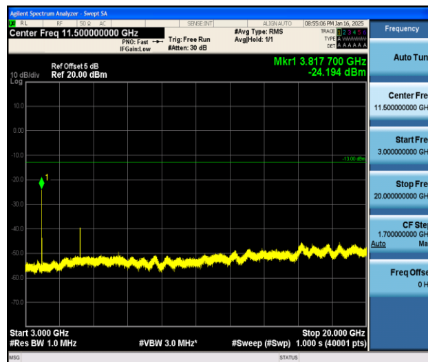
Band2_1.4MHz_16QAM_19193_1RB#0_3000~20000_3000~20000
