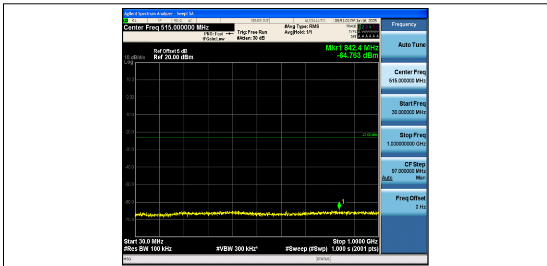
Band2_1.4MHz_16QAM_18607_1RB#0_30~1000_30~1000
