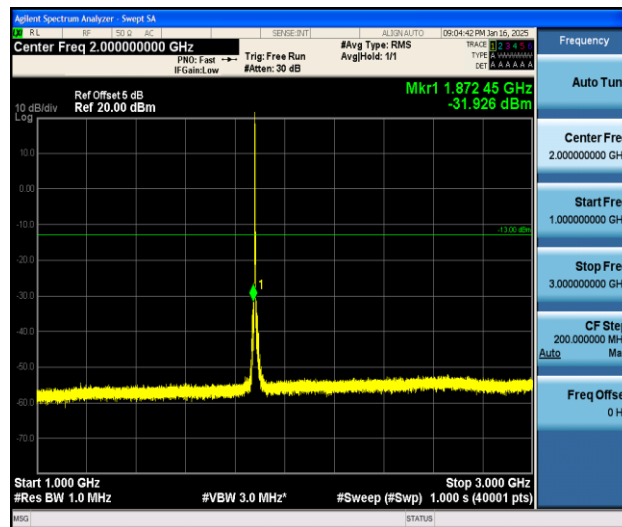
Band2_3MHz_QPSK_18900_1RB#0_1000~3000_1000~3000
