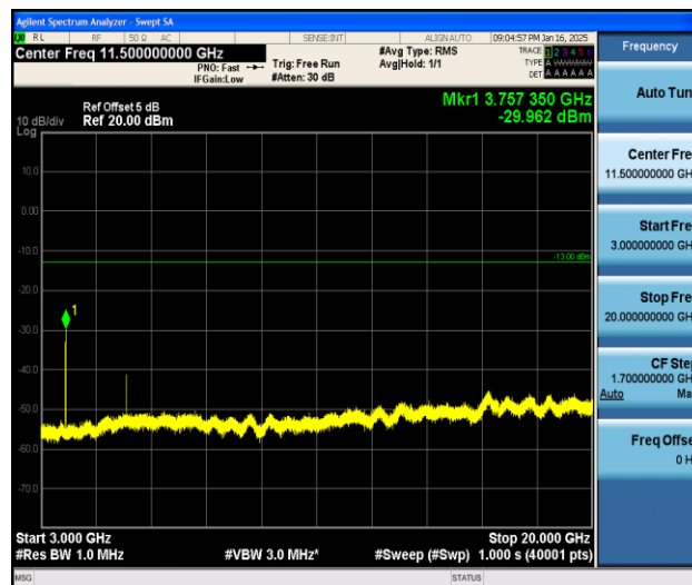
Band2_3MHz_QPSK_18900_1RB#0_3000~20000_3000~20000
