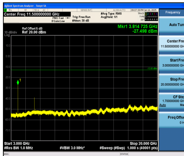
Band2_3MHz_16QAM_19185_1RB#0_3000~20000_3000~20000
