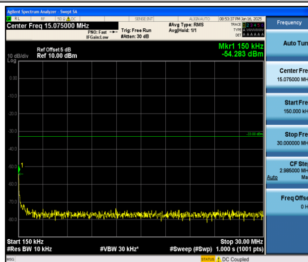
Band2_1.4MHz_QPSK_19193_1RB#0_0.15~30_0.15~30
