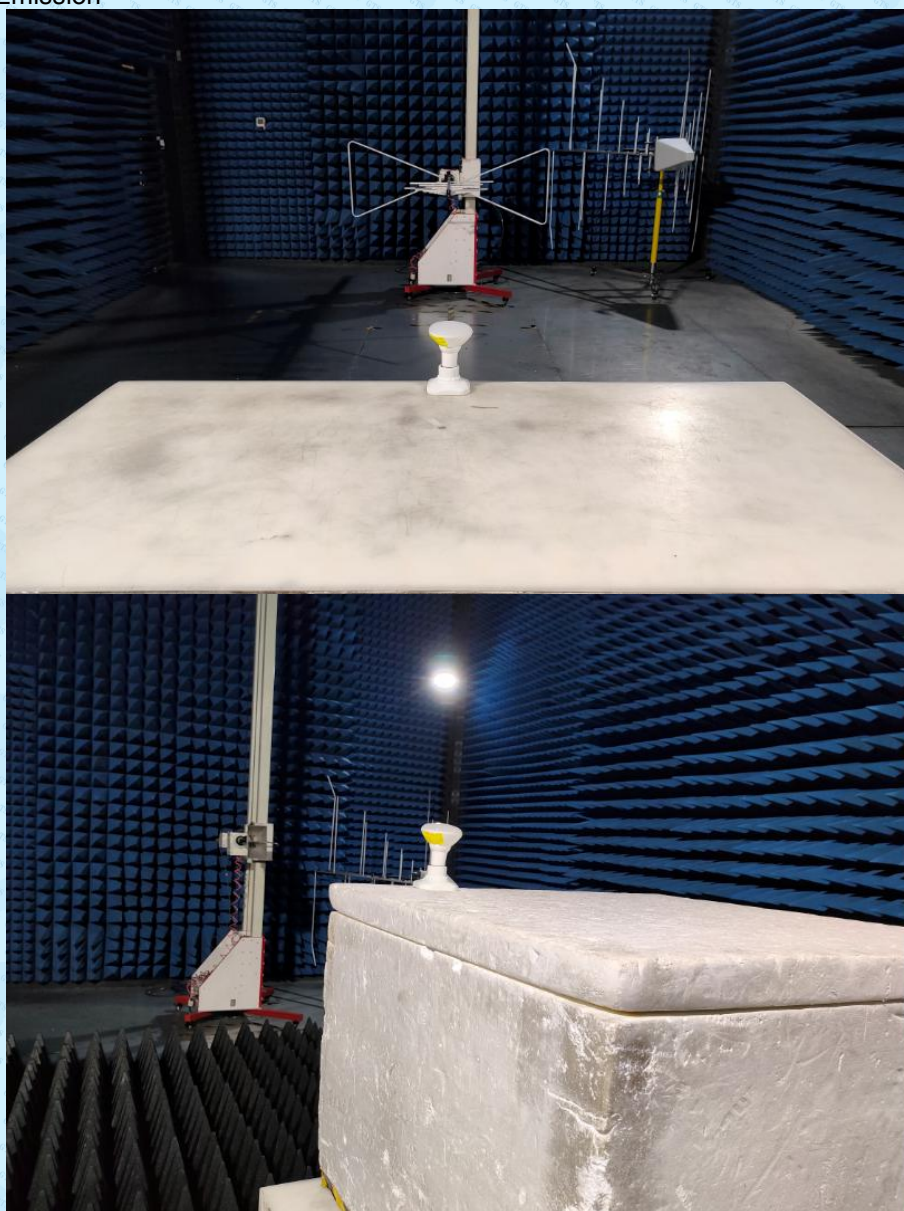
Radiated Emission
