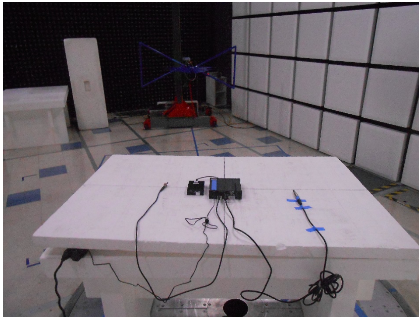
Radiated Emissions < 1 GHz
