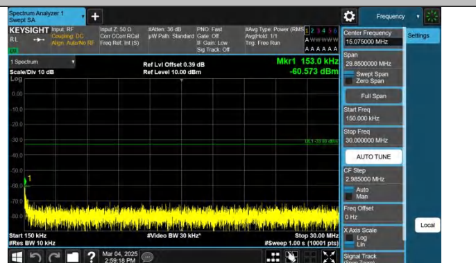
Band4-1513-4-0.15~30MHz-PASS
