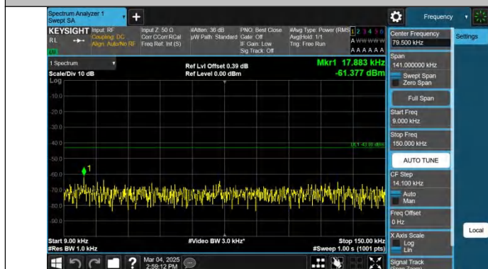
Band4-1513-4-0.009~0.15MHz-PASS
