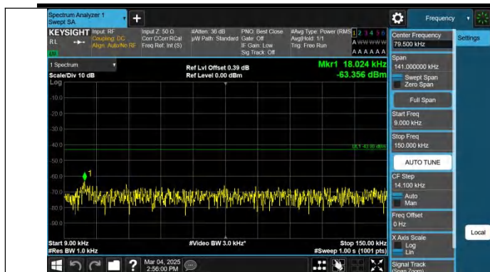
Band4-1513-3-0.009~0.15MHz-PASS
