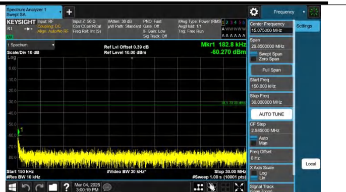
Band4-1312-5-0.15~30MHz-PASS
