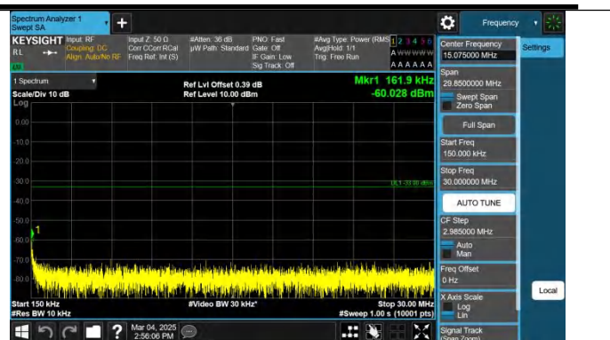
Band4-1513-3-0.15~30MHz-PASS
