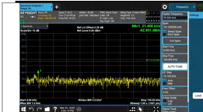
Band4-1312-5-0.009~0.15MHz-PASS
