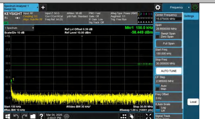
Band4-1413-1-0.15~30MHz-PASS
