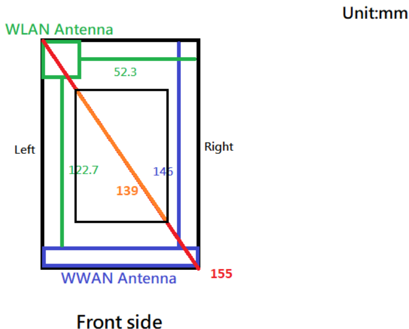
Fig.17 Antenna position of EUT
