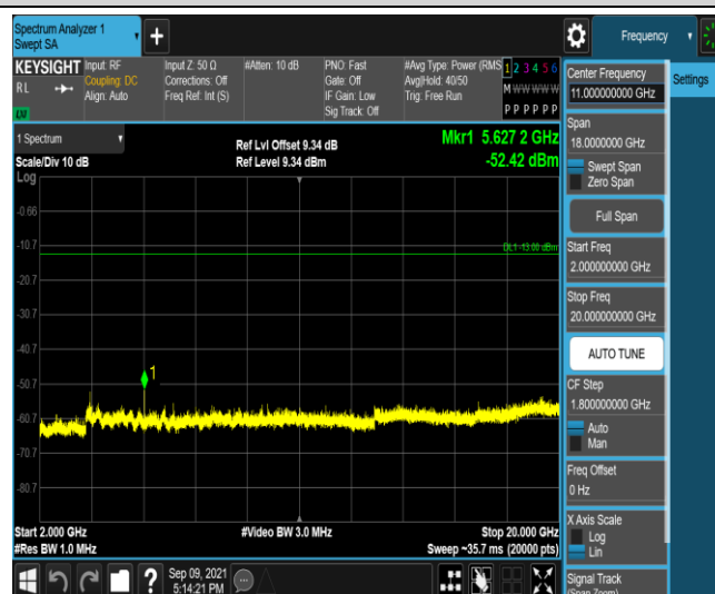
Band25-15MHz-QPSK-26365-1RB#0-Range5:2000~20000MHz
