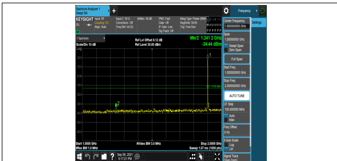
Band25-15MHz-16QAM-26615-1RB#0-Range4:1000~2000MHz
