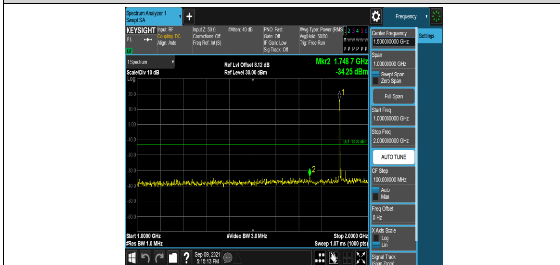
Band25-15MHz-16QAM-26365-1RB#0-Range4:1000~2000MHz
