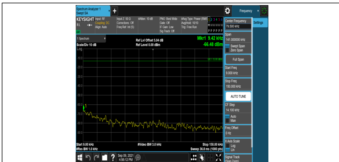
Band25-10MHz-16QAM-26640-1RB#0-Range1:0.009~0.15MHz
