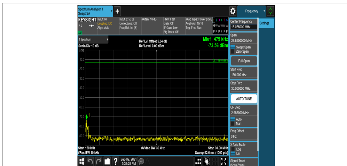
Band25-20MHz-16QAM-26140-1RB#0-Range2:0.15~30MHz
