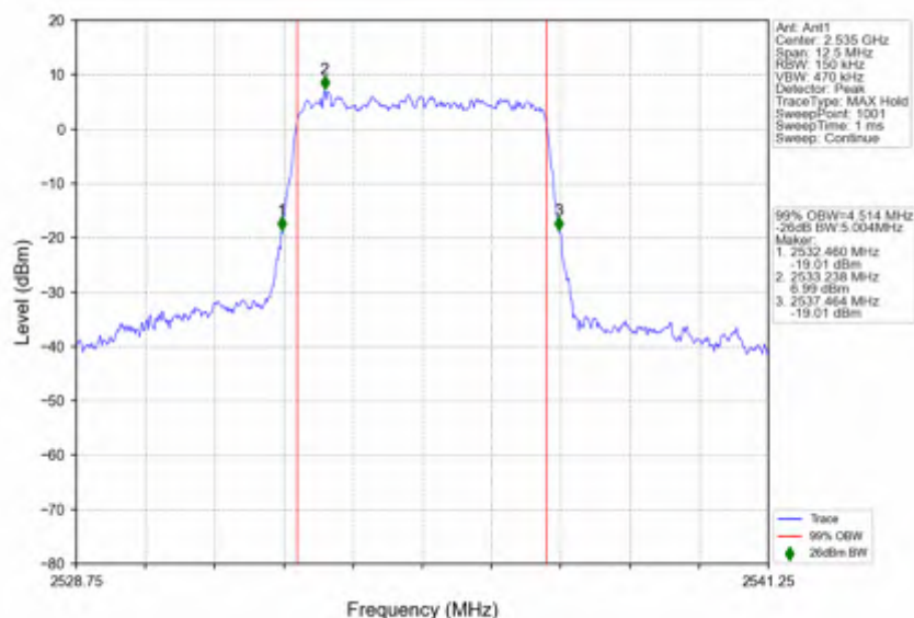
n7_15kHz_SISO_NTNV_5MHz_CP-OFDM 256 QAM 2535MHz_Outer_Full
