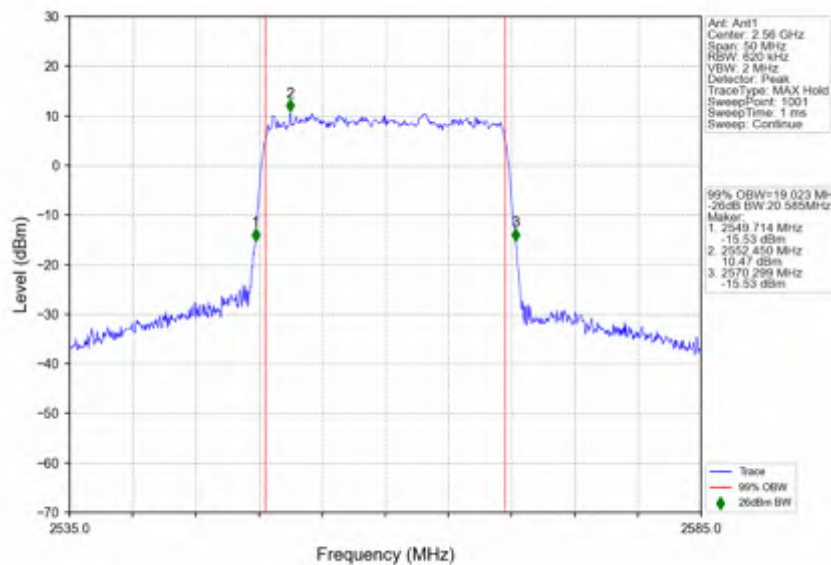
n7_15kHz_SISO_NTNV_20MHz_CP-OFDM_QPSK_2560MHz_Outer_Full
