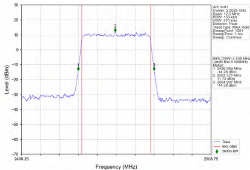
n7_15kHz_SISO_NTNV_5MHz_DFT-s-OFDM QPSK_2502.5MHz_Outer_Full
