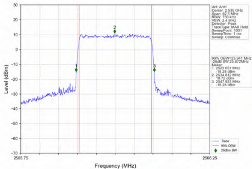
n7_15kHz_SISO_NTNV_25MHz_CP-OFDM_16_QAM_2535MHz_Outer_Full
