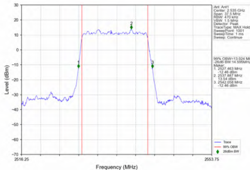
n7_30kHz_SISO_NTNV_15MHz_DFT-s-OFDM_PI/2_BPSK_2535MHz_Outer_Full
