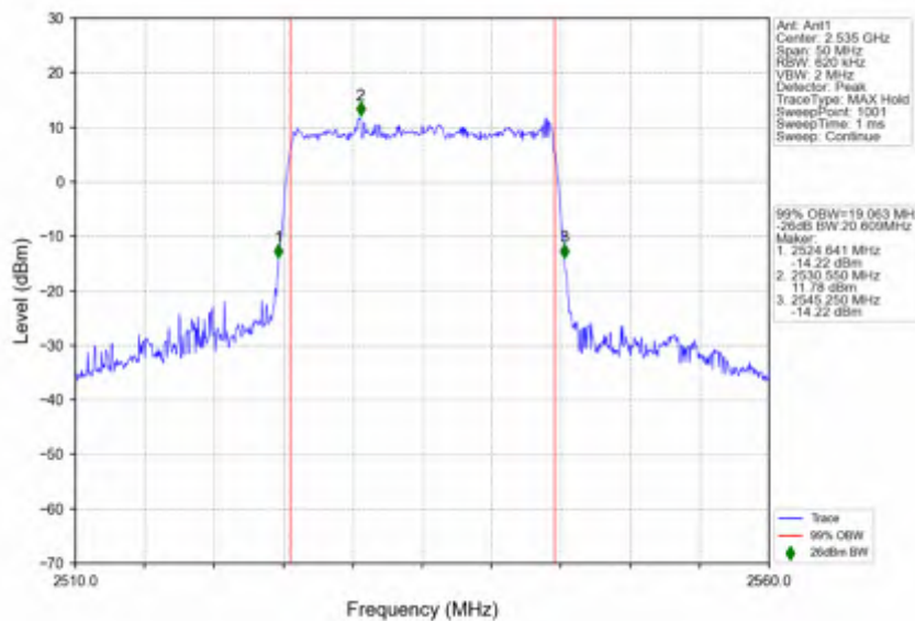
n7_15kHz_SISO_NTNV_20MHz_CP-OFDM_16_QAM_2535MHz_Outer_Full
