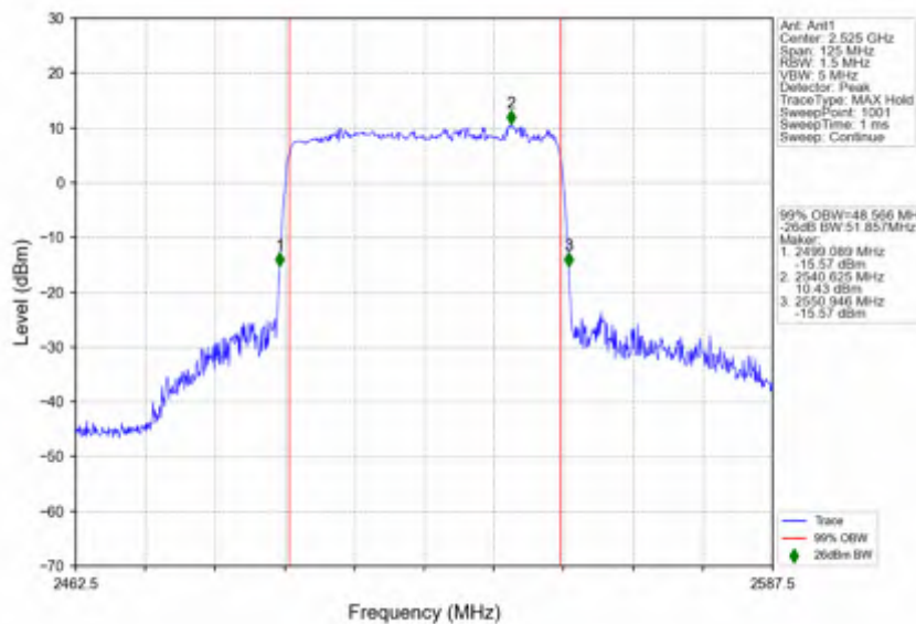
n7_15kHz_SISO_NTNV_50MHz_CP-OFDM 64 QAM_2525MHz_Outer_Full
