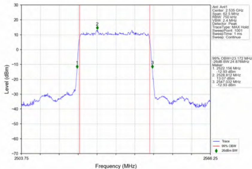
n7_15kHz_SISO_NTNV_25MHz_DFT-s-OFDM_PI/2_BPSK_2535MHz_Outer_Full
