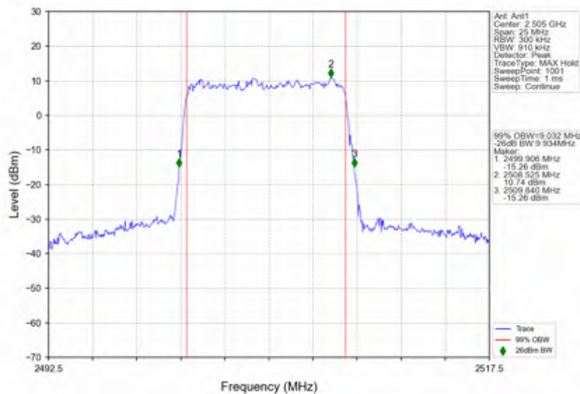
n7_15kHz_SISO_NTNV_10MHz_DFT-s-OFDM_64 QAM_2505MHz_Outer_Full
