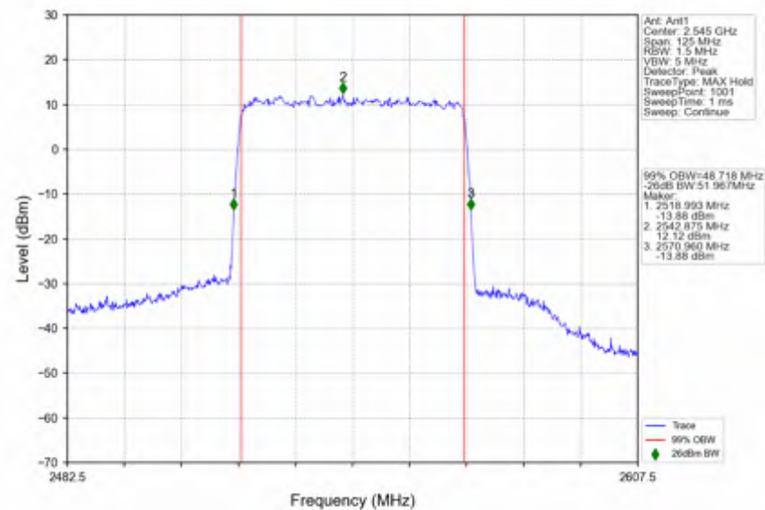
n7_15kHz_SISO_NTNV_50MHz_DFT-s-OFDM_QPSK_2545MHz_Outer_Full
