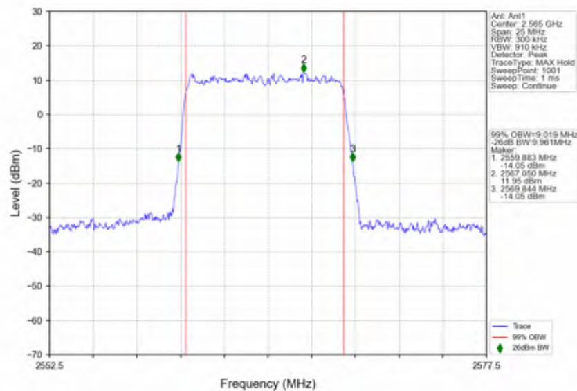
n7_15kHz_SISO_NTNV_10MHz_DFT-s-OFDM_QPSK_2565MHz_Outer_Full
