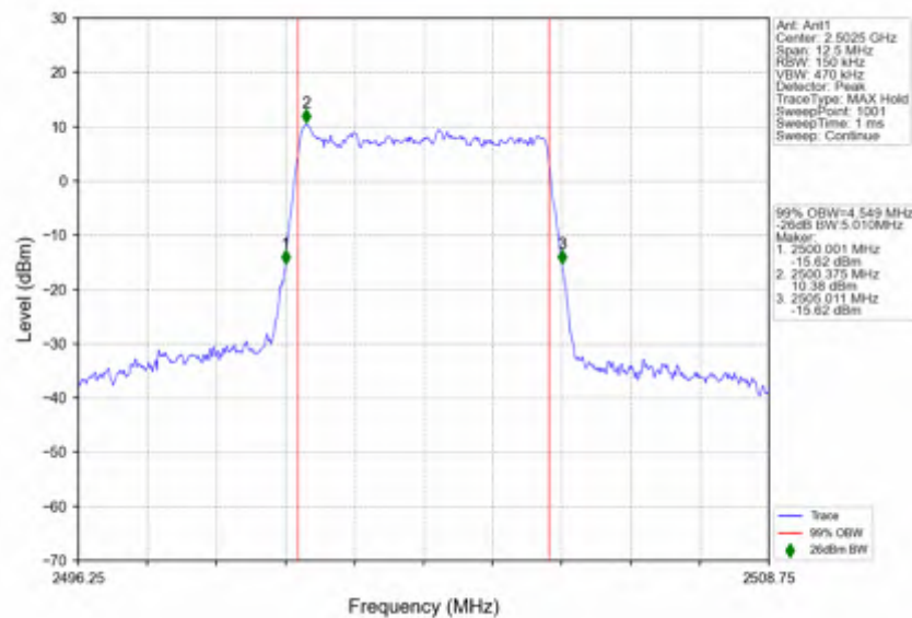
n7_15kHz_SISO_NTNV_5MHz_CP-OFDM_64_QAM_2502.5MHz_Outer_Full
