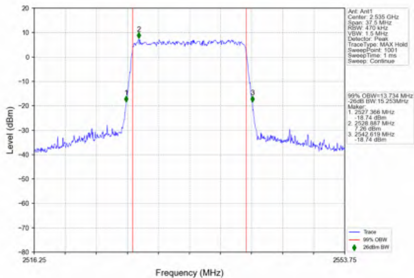
n7 30kHz SISO NTV 15MHz CP-OFDM 256 QAM 2535MHz Outer Full
