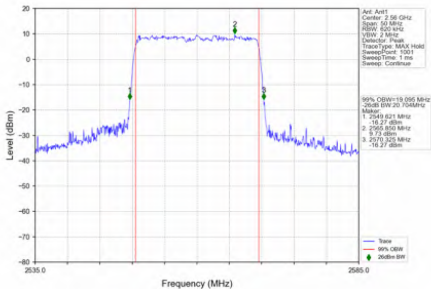
n7 15kHz SISO NTN 20MHz CP-OFDM 64 QAM 2560MHz Outer Full
