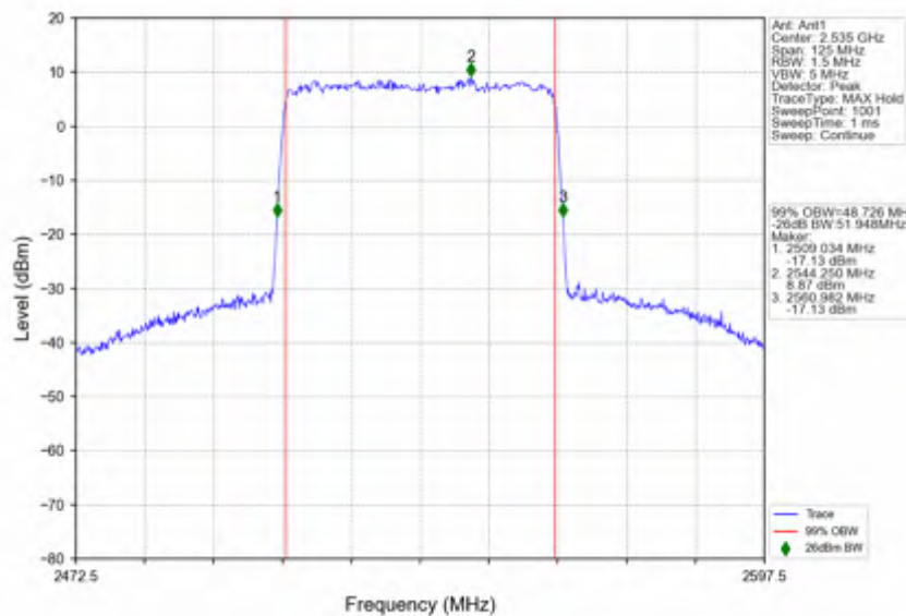
n7_15kHz_SISO_NTNV_50MHz_DFT-s-OFDM_256_QAM_2535MHz_Outer_Full
