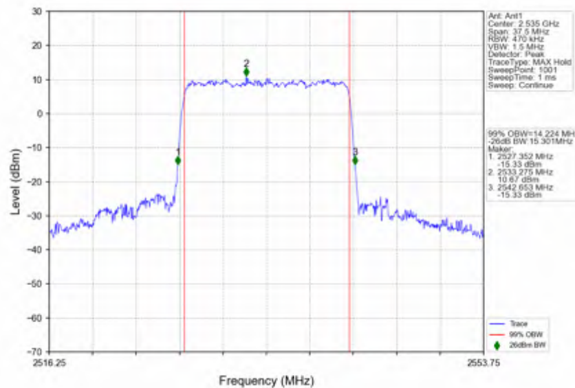
n7_15kHz_SISO_NTNV_15MHz_CP-OFDM_16_QAM_2535MHz_Outer_Full
