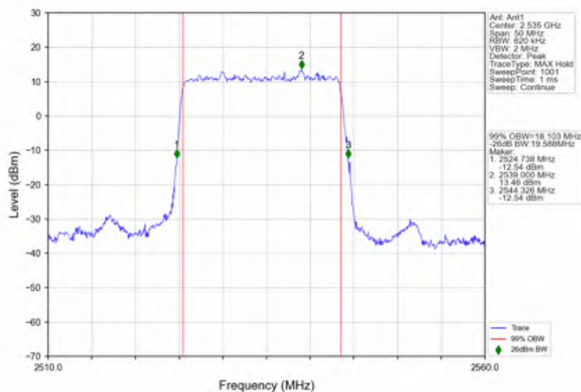
n7_15kHz_SISO_NTNV_20MHz_DFT-s-OFDM PI/2 BPSK_2535MHz_Outer_Full
