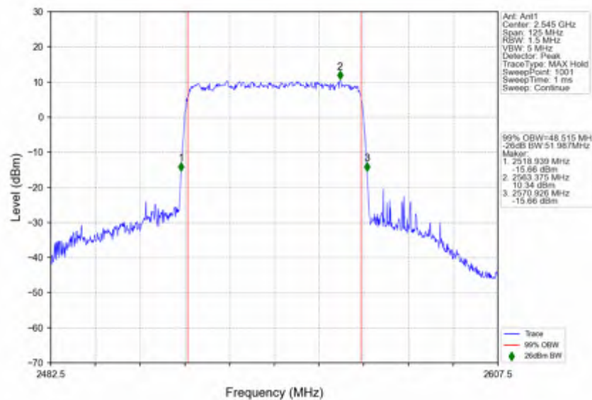
n7_15kHz_SISO_NTNV_50MHz_CP-OFDM_QPSK_2545MHz_Outer_Full
