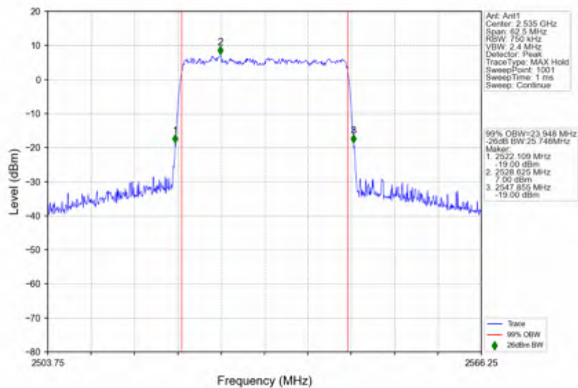
n7 15kHz SISO NTNV 25MHz CP-OFDM 256 QAM 2535MHz Outer Full
