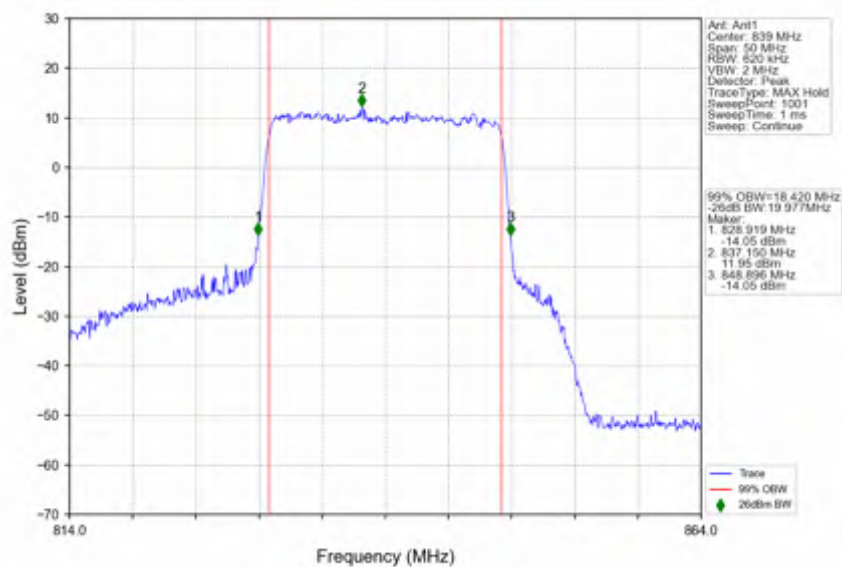
n5_30kHz_SISO_NTNV_20MHz_CP-OFDM_64_QAM_839MHz_Outer_Full
