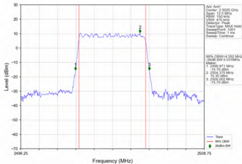
n7_15kHz_SISO_NTNV_5MHz_DFT-s-OFDM 64 QAM 2502.5MHz_Outer_Full
