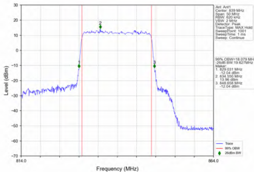
n5_30kHz_SISO_NTNV_20MHz_DFT-s-OFDM_QPSK_839MHz_Outer_Full
