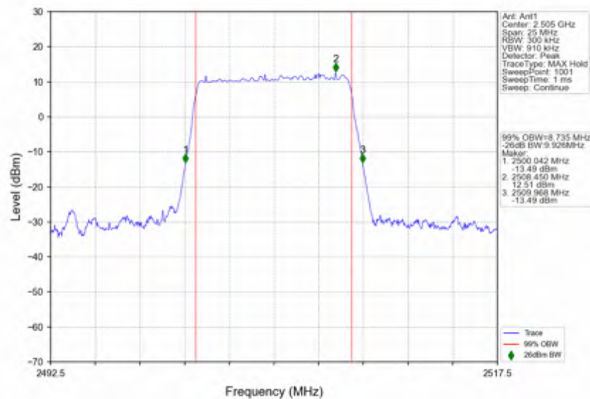
n7_30kHz_SISO_NTNV_10MHz_DFT-s-OFDM QPSK_2505MHz_Outer_Full
