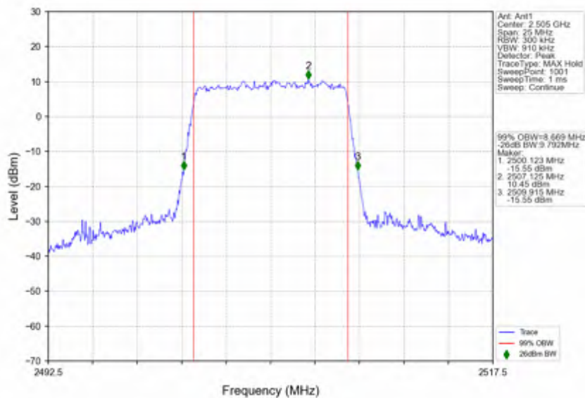
n7_30kHz_SISO_NTNV_10MHz_CP-OFDM 64 QAM_2505MHz_Outer_Full
