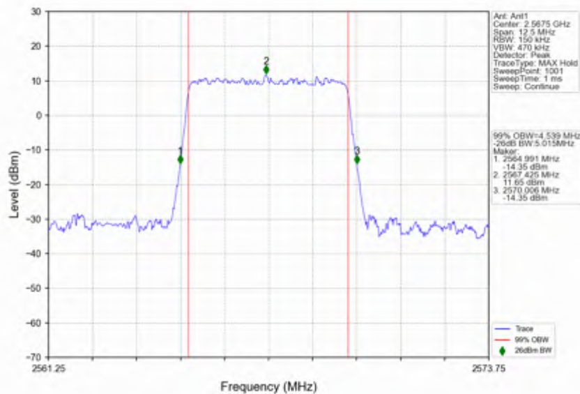
n7_15kHz_SISO_NTNV_5MHz_DFT-s-OFDM QPSK_2567.5MHz_Outer_Full
