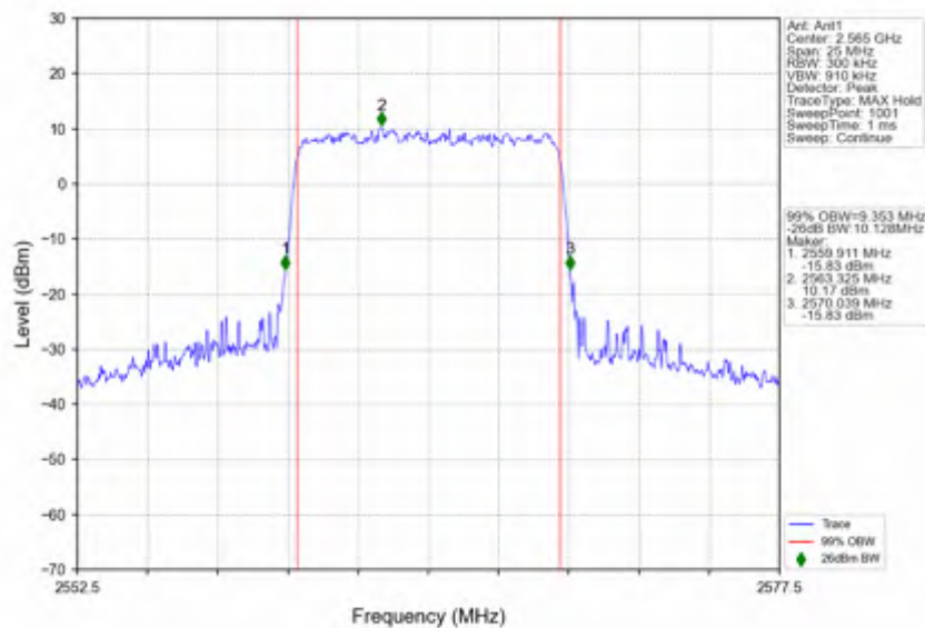
n7_15kHz_SISO_NTNV_10MHz_CP-OFDM_QPSK_2565MHz_Outer_Full
