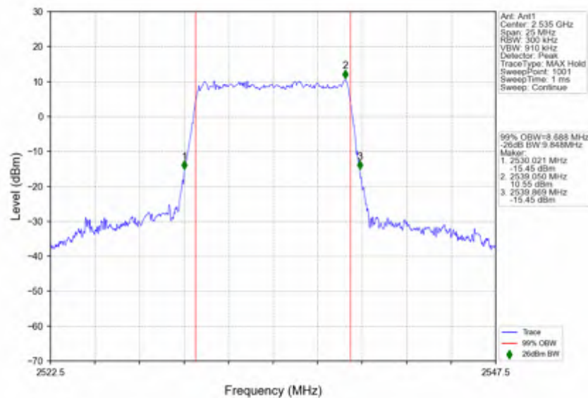
n7_30kHz_SISO_NTNV_10MHz_CP-OFDM_16_QAM_2535MHz_Outer_Full
