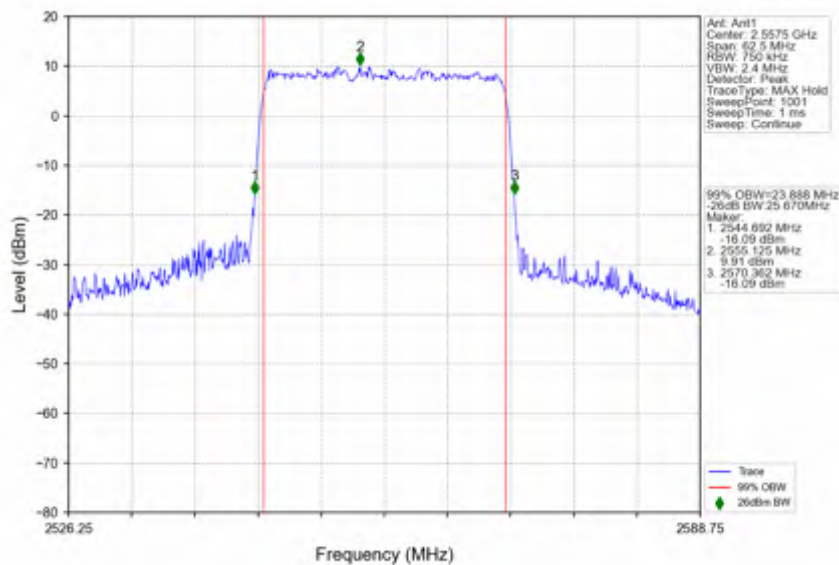
n7_15kHz_SISO_NTNV_25MHz_CP-OFDM 64 QAM_2557.5MHz_Outer_Full
