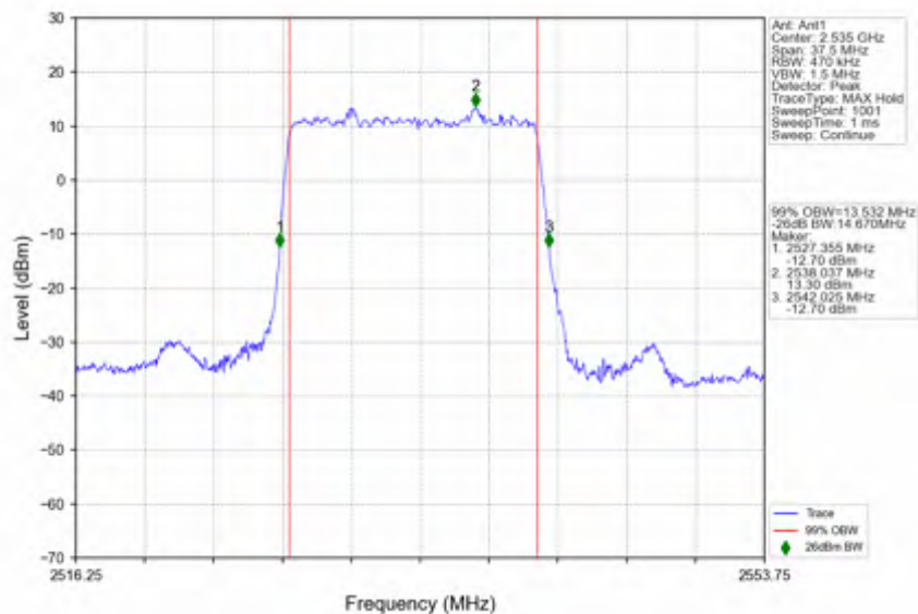
n7_15kHz_SISO_NTNV_15MHz_DFT-s-OFDM_PI/2_BPSK_2535MHz_Outer_Full
