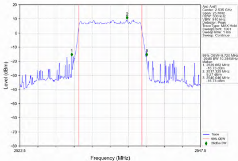
n7 30kHz SISO NTV 10MHz DFT-s-OFDM 256 QAM 2535MHz Outer Full
