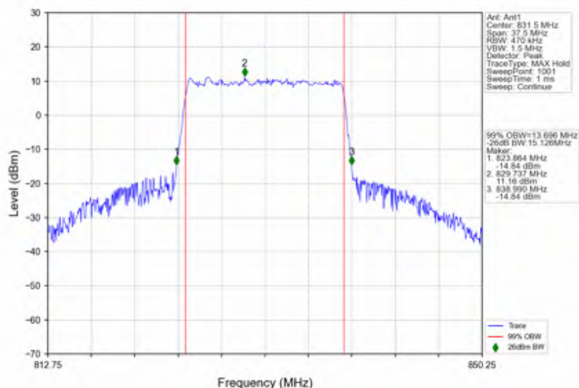
n5 30kHz SISO NTNV 15MHz CP-OFDM 64 QAM 831.5MHz Outer Full
