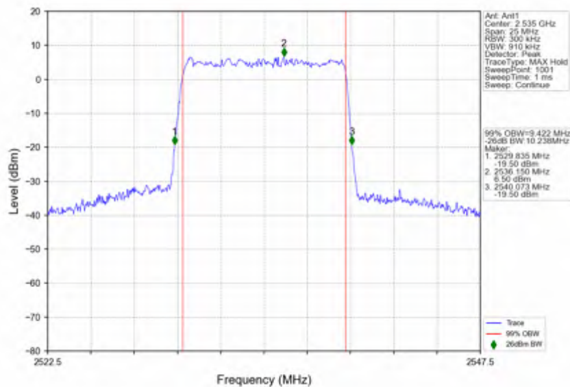
n7_15kHz_SISO_NTNV_10MHz_CP-OFDM_256_QAM_2535MHz_Outer_Full
