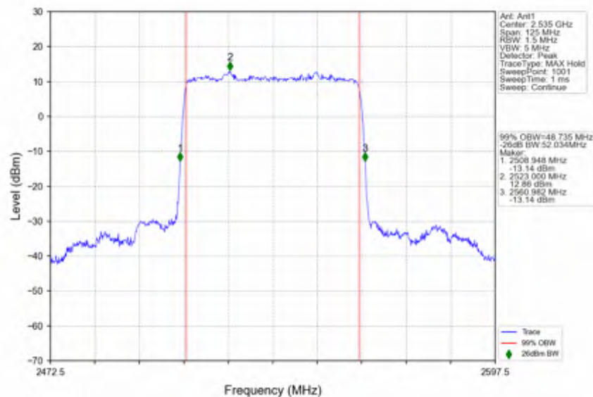
n7_15kHz_SISO_NTNV_50MHz_DFT-s-OFDM_PI/2_BPSK_2535MHz_Outer_Full
