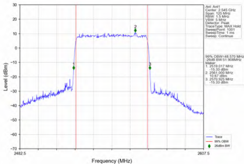
n7_15kHz_SISO_NTNV_50MHz_CP-OFDM 64 QAM_2545MHz_Outer_Full
