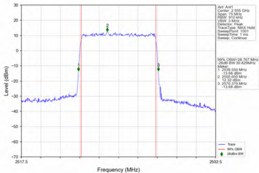
n7_15kHz_SISO_NTNV_30MHz_DFT-s-OFDM_QPSK_2555MHz_Outer_Full
