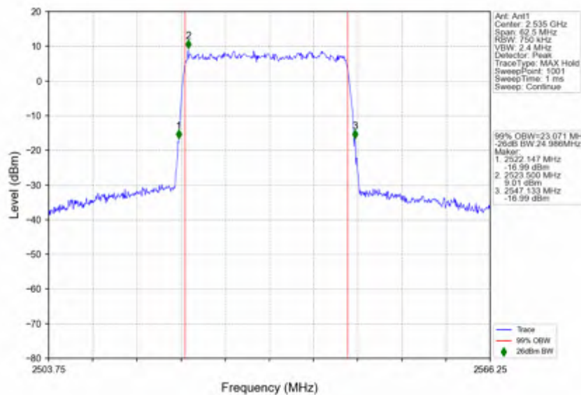
n7_15kHz_SISO_NTNV_25MHz_DFT-s-OFDM_256_QAM_2535MHz_Outer_Full
