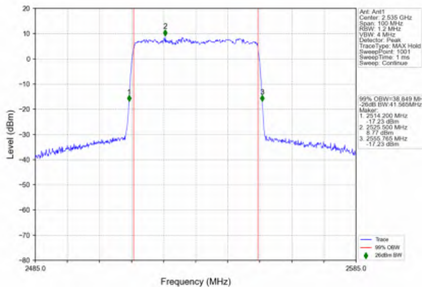
n7_15kHz_SISO_NTNV_40MHz_DFT-s-OFDM_256_QAM_2535MHz_Outer_Full
