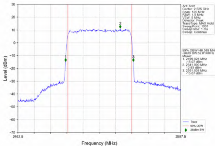
n7_15kHz_SISO_NTNV_50MHz_DFT-s-OFDM 64 QAM_2525MHz_Outer_Full
