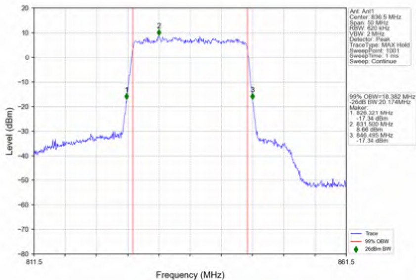
n5_30kHz_SISO_NTNV_20MHz_CP-OFDM 256 QAM_836.5MHz_Outer_Full
