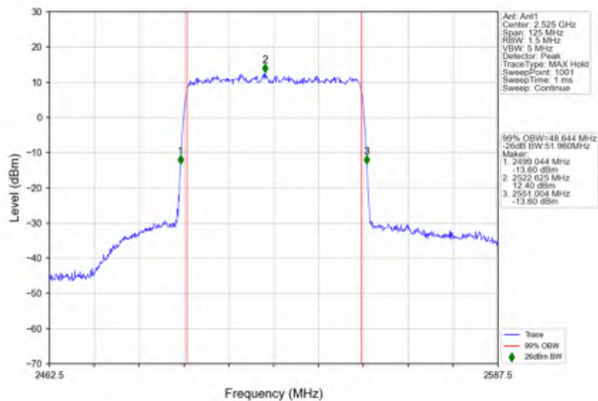
n7_15kHz_SISO_NTNV_50MHz_DFT-s-OFDM QPSK_2525MHz_Outer_Full
