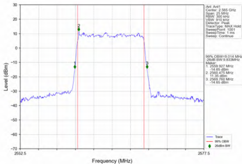
n7_15kHz_SISO_NTNV_10MHz_DFT-s-OFDM_64_QAM_2565MHz_Outer_Full
