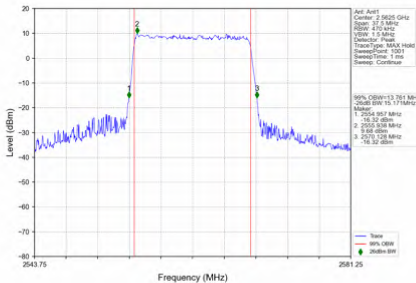
n7_30kHz_SISO_NTNV_15MHz_CP-OFDM 64 QAM_2562.5MHz_Outer_Full
