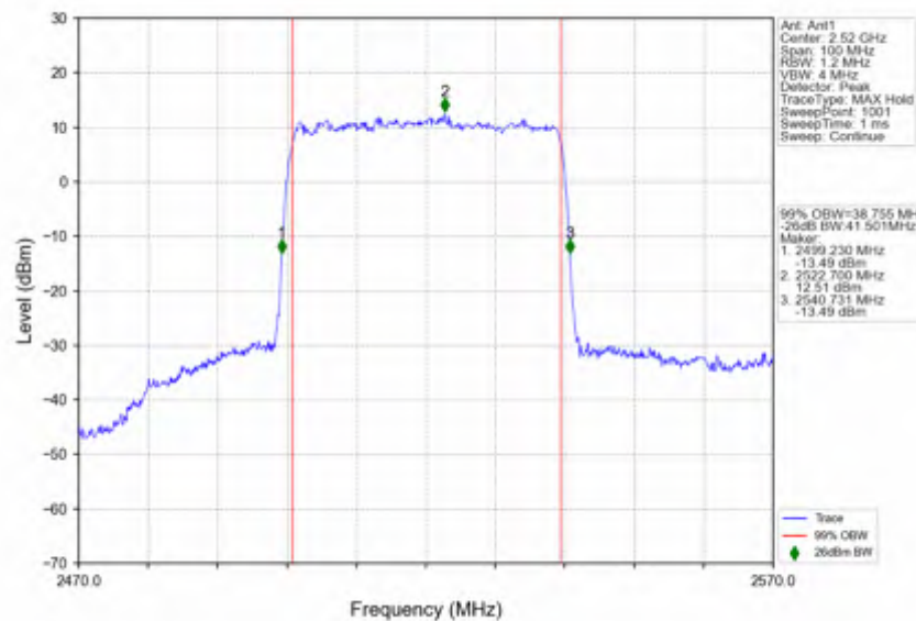
n7_15kHz_SISO_NTNV_40MHz_DFT-s-OFDM QPSK_2520MHz_Outer_Full
