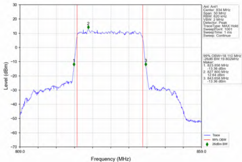
n5_30kHz_SISO_NTNV_20MHz_DFT-s-OFDM_64_QAM_834MHz_Outer_Full
