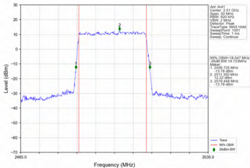
n7_15kHz_SISO_NTNV_20MHz_DFT-s-OFDM_QPSK_2510MHz_Outer_Full
