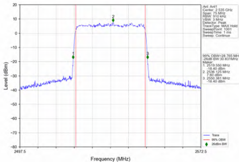
n7_15kHz_SISO_NTNV_30MHz_CP-OFDM_256_QAM_2535MHz_Outer_Full
