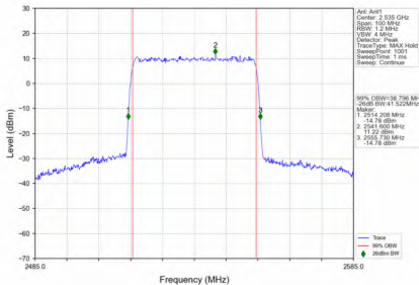
n7_15kHz_SISO_NTNV_40MHz_DFT-s-OFDM_16_QAM_2535MHz_Outer_Full
