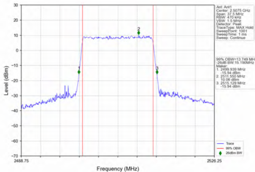
n7_30kHz_SISO_NTNV_15MHz_CP-OFDM_64 QAM_2507.5MHz_Outer_Full
