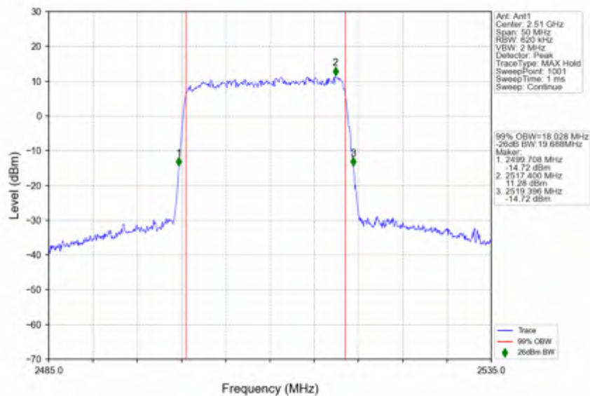
n7_15kHz_SISO_NTNV_20MHz_DFT-s-OFDM_64 QAM_2510MHz_Outer_Full
