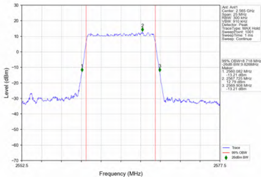
n7_30kHz_SISO_NTNV_10MHz_DFT-s-OFDM_QPSK_2565MHz_Outer_Full
