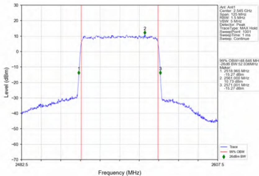
n7_15kHz_SISO_NTNV_50MHz_DFT-s-OFDM_64_QAM_2545MHz_Outer_Full
