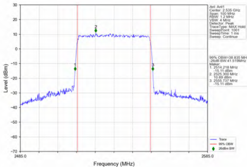
n7_15kHz_SISO_NTNV_40MHz_CP-OFDM_16_QAM_2535MHz_Outer_Full
