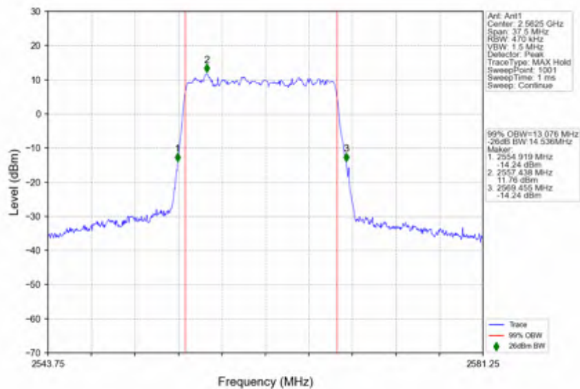
n7_30kHz_SISO_NTNV_15MHz_DFT-s-OFDM_64_QAM_2562.5MHz_Outer_Full
