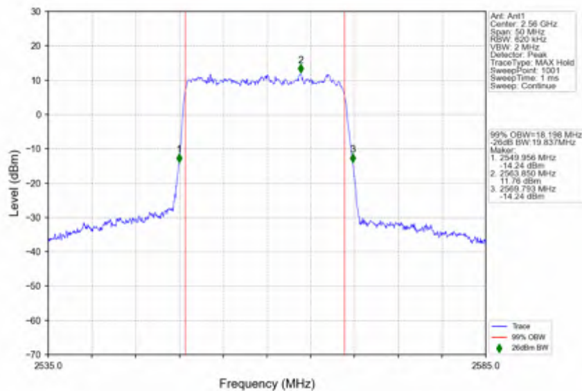
n7_30kHz_SISO_NTNV_20MHz_DFT-s-OFDM_64_QAM_2560MHz_Outer_Full
