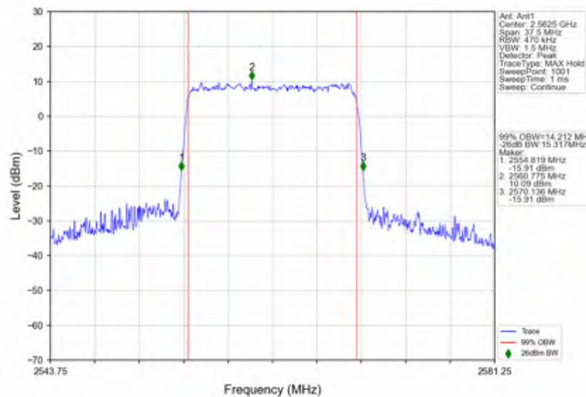
n7_15kHz_SISO_NTNV_15MHz_CP-OFDM 64 QAM_2562.5MHz_Outer_Full
