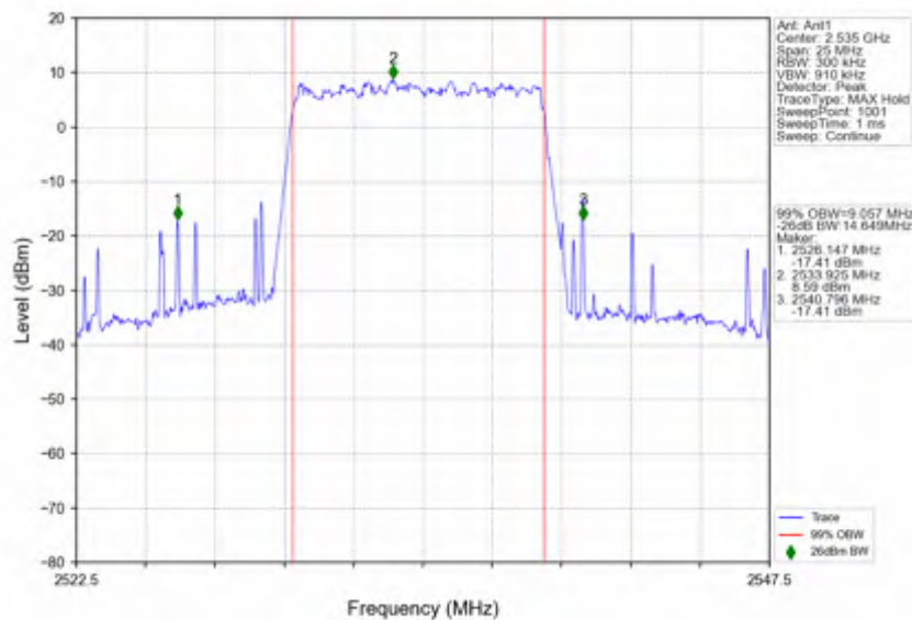
n7_15kHz_SISO_NTNV_10MHz_DFT-s-OFDM_256_QAM_2535MHz_Outer_Full
