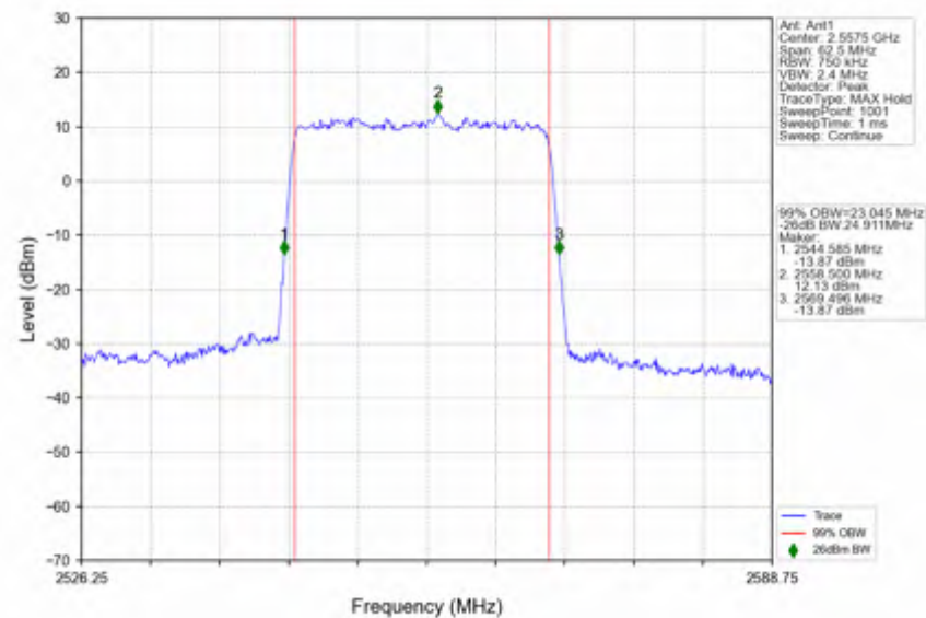
n7_15kHz_SISO_NTNV_25MHz_DFT-s-OFDM QPSK_2557.5MHz_Outer_Full
