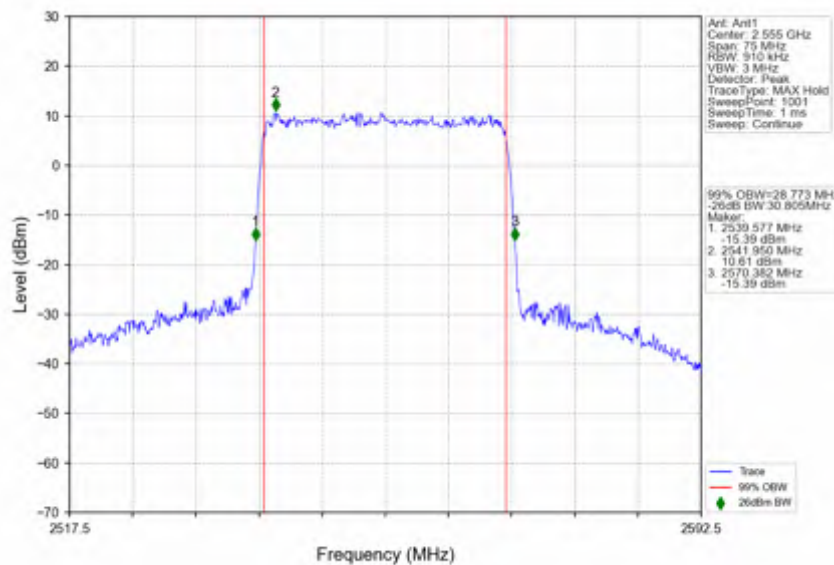
n7_15kHz_SISO_NTNV_30MHz_CP-OFDM_QPSK_2555MHz_Outer_Full
