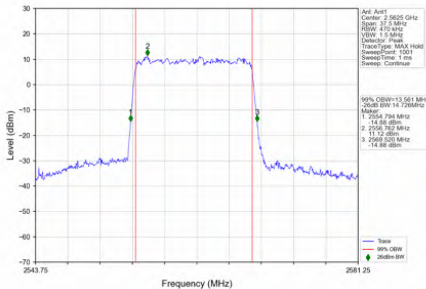
n7_15kHz_SISO_NTNV_15MHz_DFT-s-OFDM_64_QAM_2562.5MHz_Outer_Full
