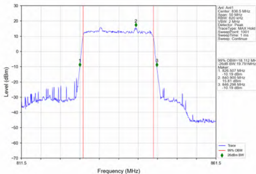
n5_30kHz_SISO_NTNV_20MHz_DFT-s-OFDM_PI/2_BPSK_836.5MHz_Outer_Full
