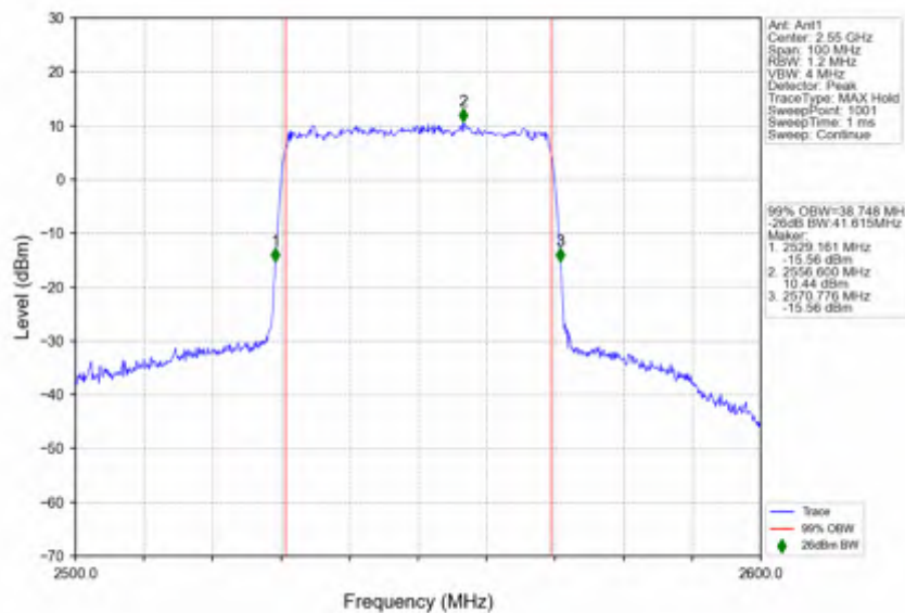
n7_15kHz_SISO_NTNV_40MHz_DFT-s-OFDM_64_QAM_2550MHz_Outer_Full
