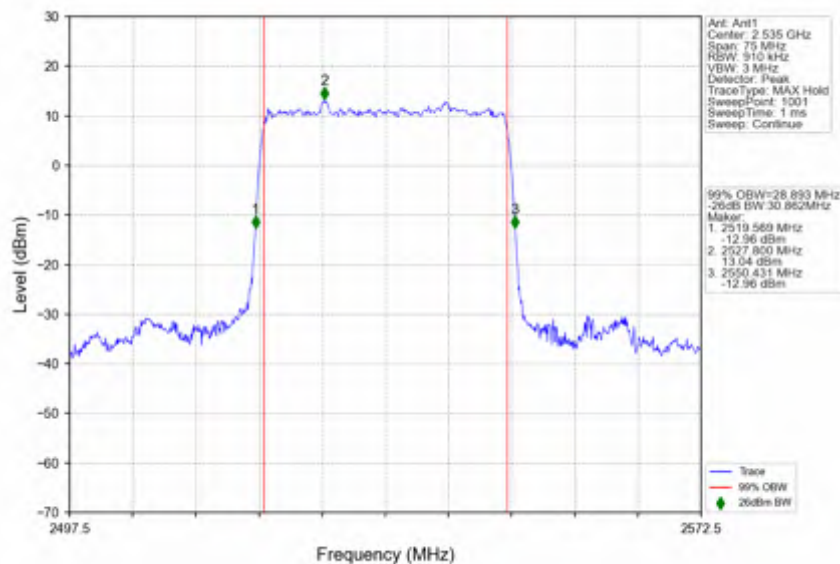
n7_15kHz_SISO_NTNV_30MHz_DFT-s-OFDM_PI/2_BPSK_2535MHz_Outer_Full
