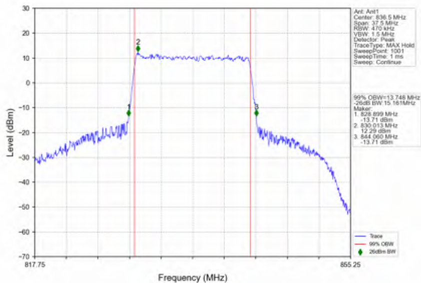
n5_30kHz_SISO_NTNV_15MHz_CP-OFDM_16_QAM_836.5MHz_Outer_Full
