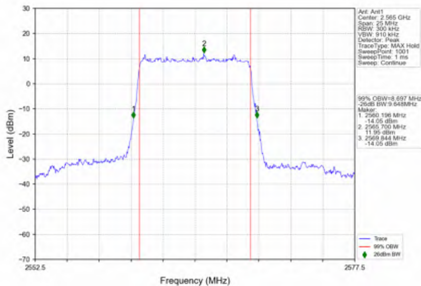
n7_30kHz_SISO_NTNV_10MHz_DFT-s-OFDM_64_QAM_2565MHz_Outer_Full
