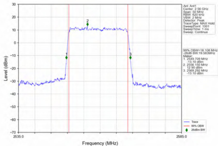
n7_15kHz_SISO_NTNV_20MHz_DFT-s-OFDM_QPSK_2560MHz_Outer_Full
