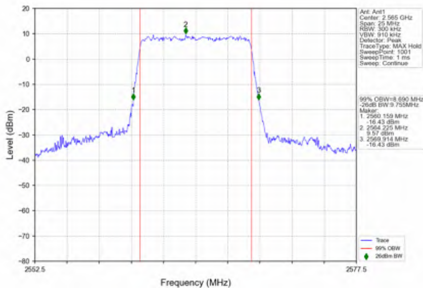
n7_30kHz_SISO_NTNV_10MHz_CP-OFDM 64 QAM_2565MHz_Outer_Full
