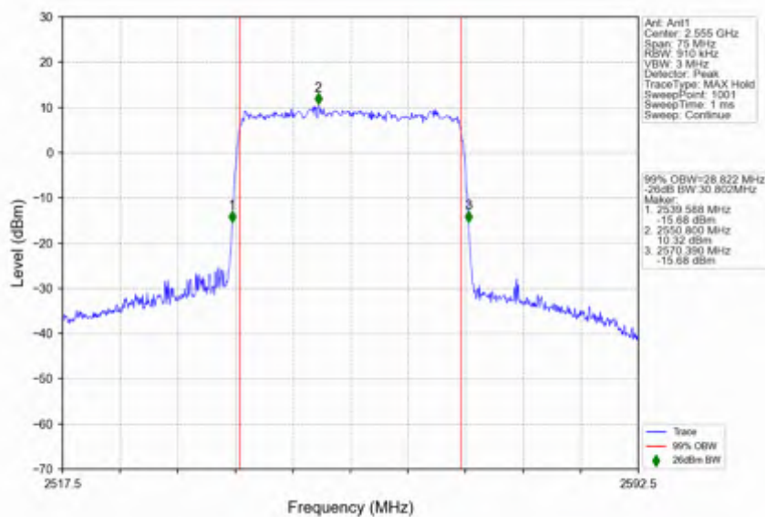
n7 15kHz SISO NTN 30MHz CP-OFDM 64 QAM 2555MHz Outer Full
