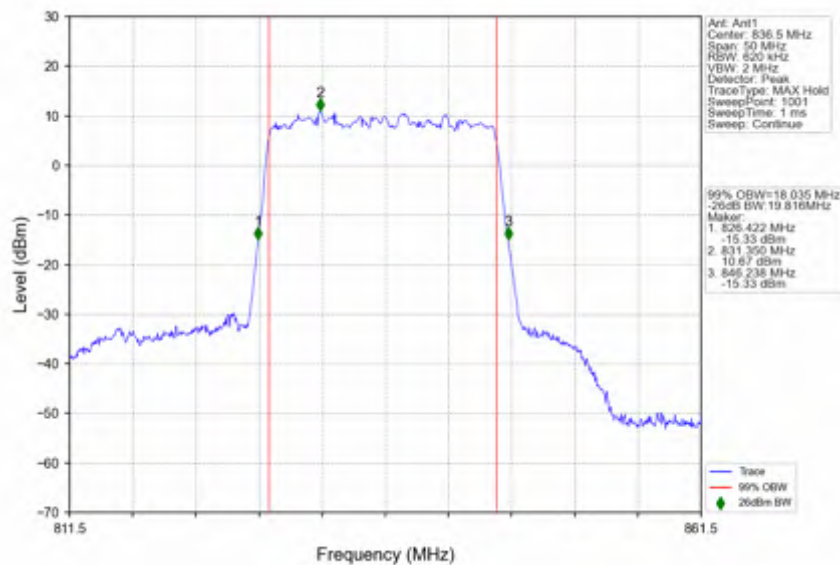
n5_30kHz_SISO_NTNV_20MHz_DFT-s-OFDM_256_QAM_836.5MHz_Outer_Full
