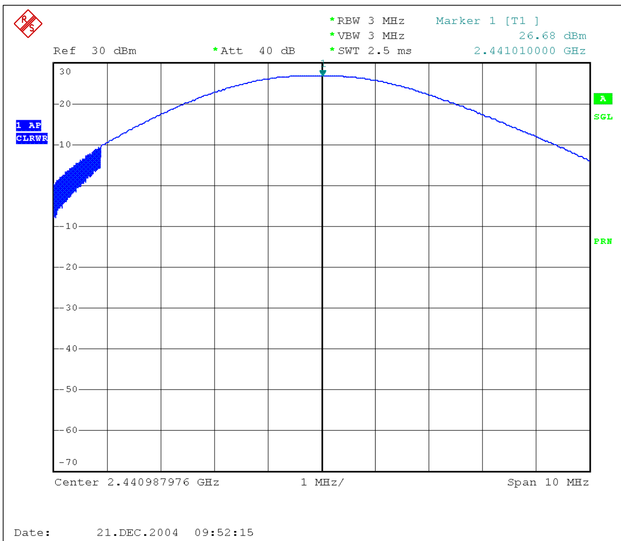
Graph # 3-1-1 Peak Output Power
