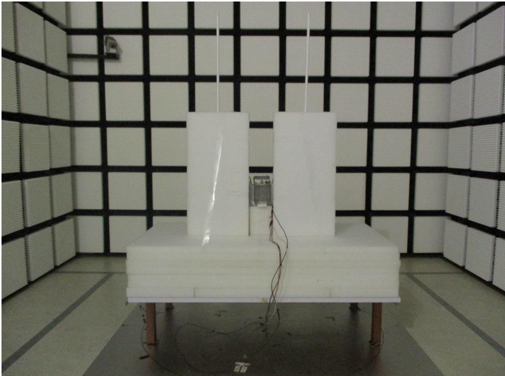
Radiated Emission Below 1GHz Test (DC mode)
