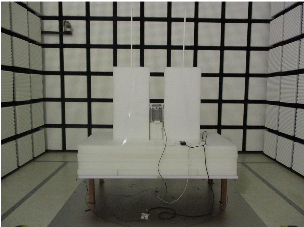
Radiated Emission Below 1GHz Test (POE mode)
