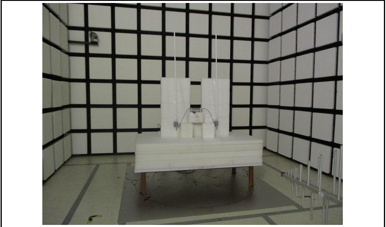
Radiated Emission Below 1GHz Test (DC mode)
