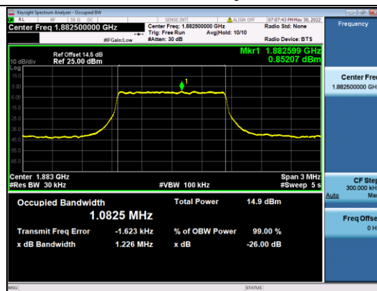
B25-1.4M-Mid CH-OBW-QPSK
