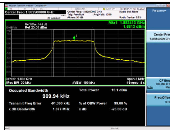
B25-1.4M-Mid CH-OBW-Q16
