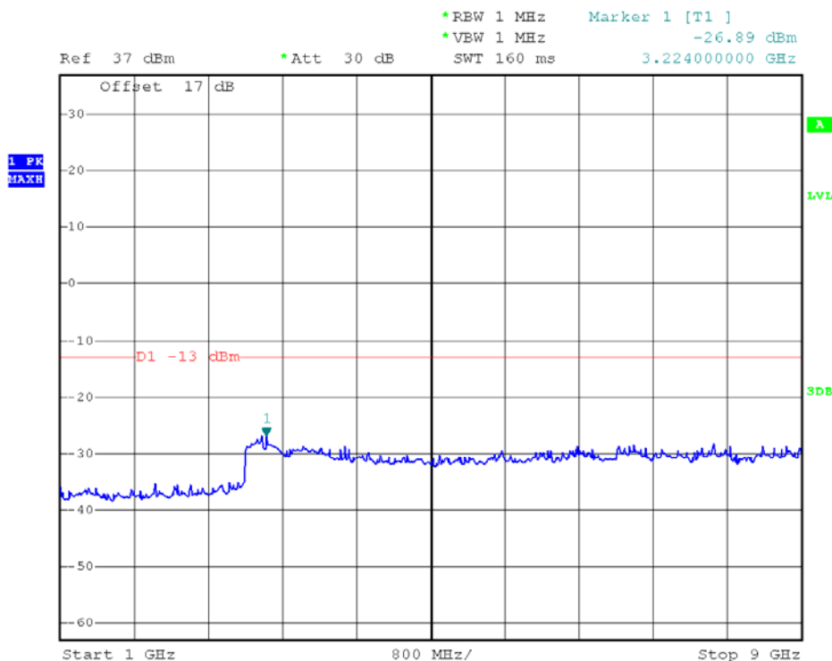
WCDMA850MHz Channel = 4233, 1GHz to 9GHz
