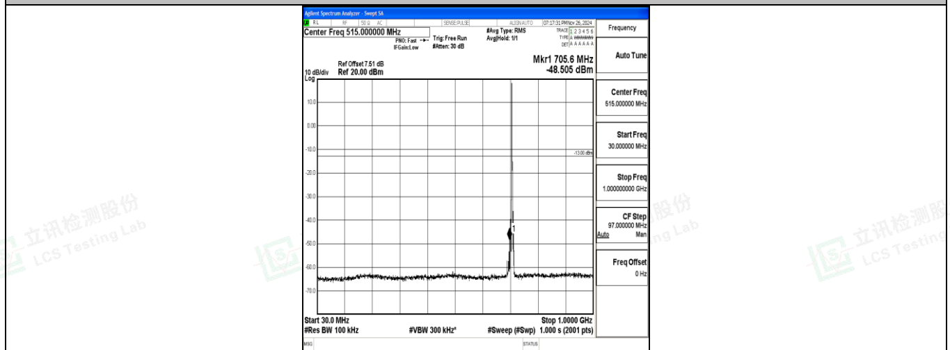
Band12_3MHz_16QAM_23165_1RB#0_30~1000_30~1000
