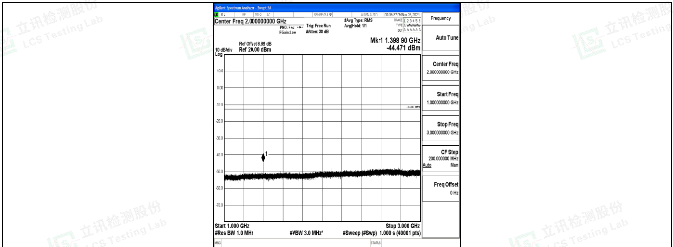
Band12_5MHz_16QAM_23035_1RB#0_1000~3000_1000~3000
