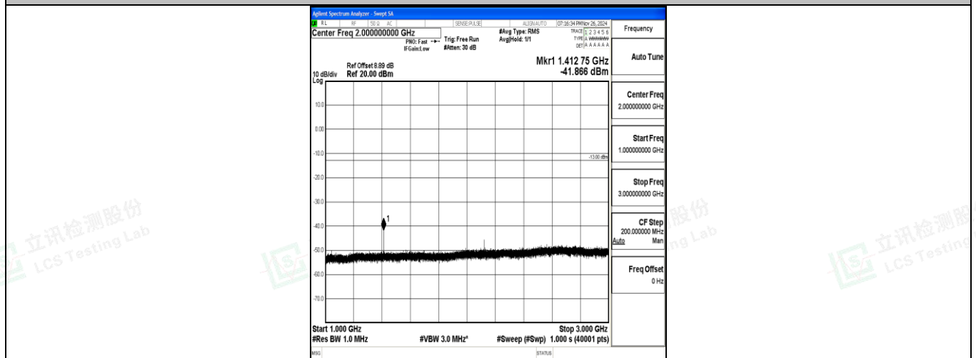
Band12_3MHz_16QAM_23095_1RB#0_1000~3000_1000~3000
