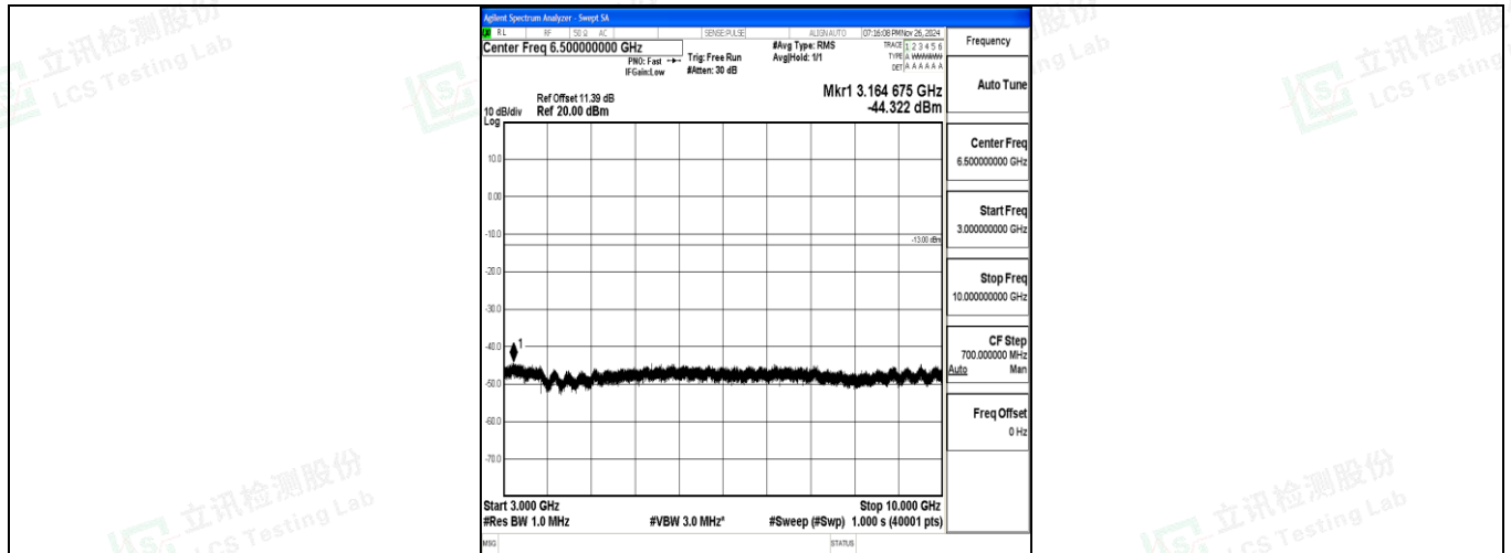
Band12_3MHz_QPSK_23095_1RB#0_3000~10000_3000~10000
