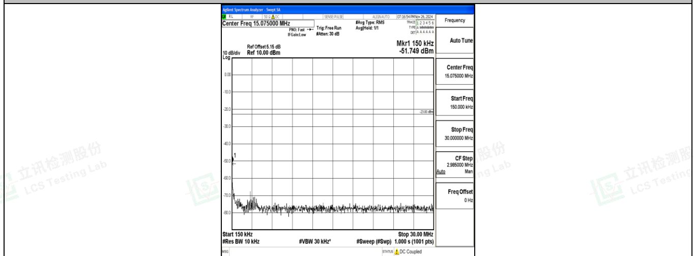
Band12_3MHz_QPSK_23165_1RB#0_0.15~30_0.15~30
