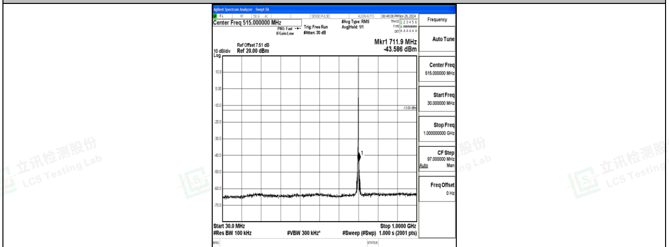
Band12_1.4MHz_QPSK_23095_1RB#0_30~1000_30~1000
