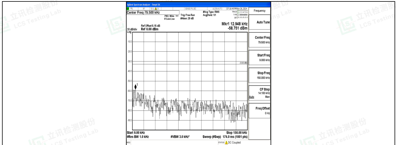
Band12_3MHz_QPSK_23165_1RB#0_0.009~0.15_0.009~0.15
