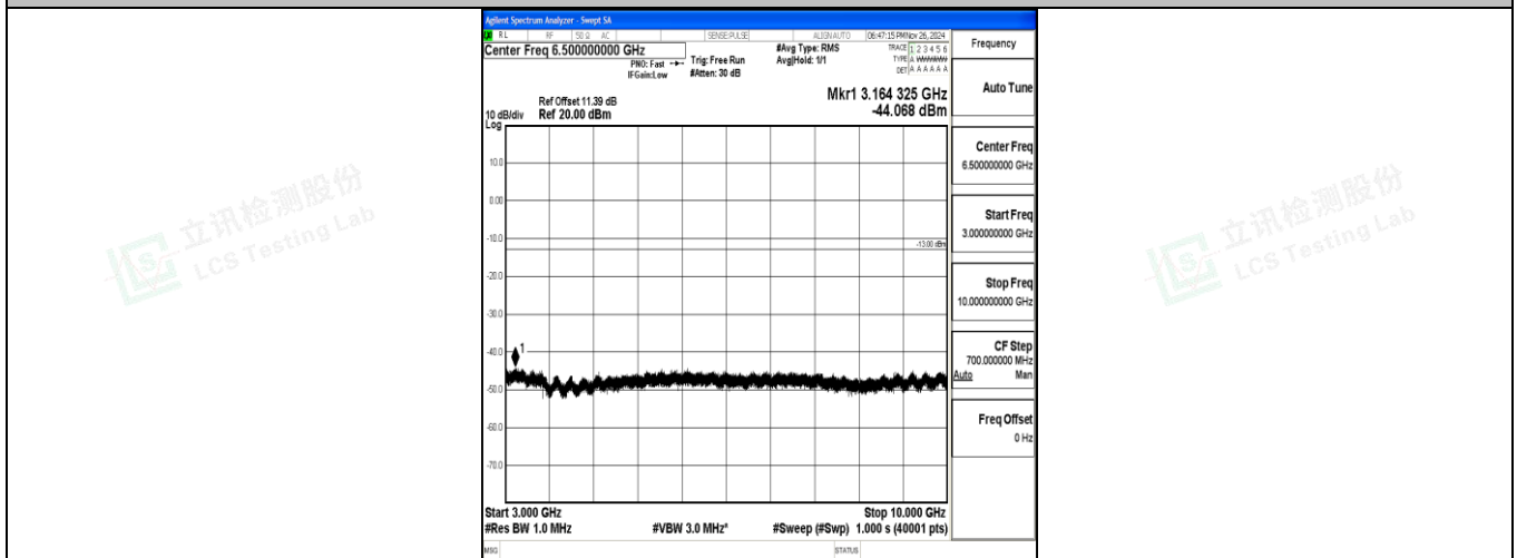
Band12_1.4MHz_QPSK_23017_1RB#0_3000~10000_3000~10000
