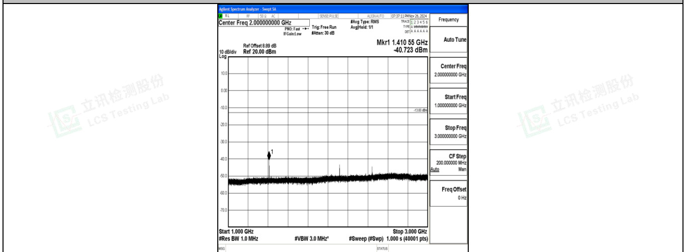
Band12_5MHz_QPSK_23095_1RB#0_1000~3000_1000~3000
