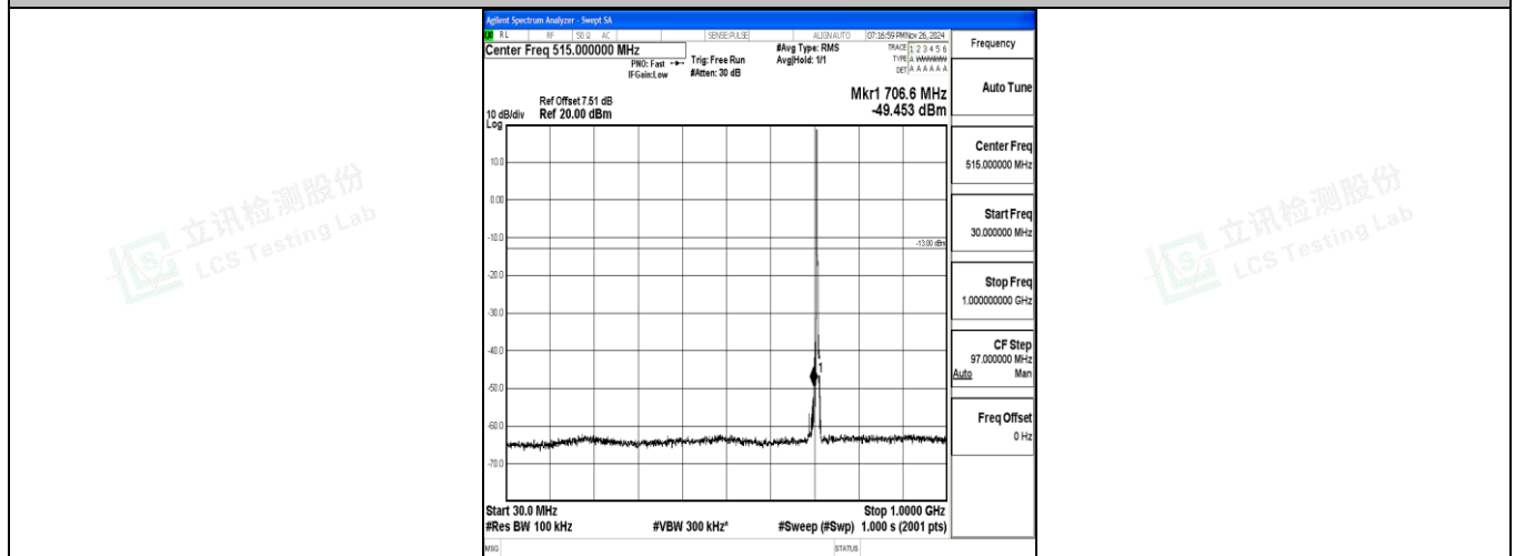
Band12_3MHz_QPSK_23165_1RB#0_30~1000_30~1000
