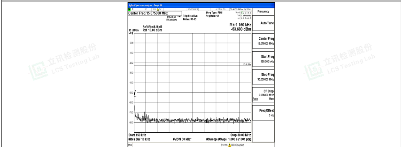
Band12_1.4MHz_16QAM_23095_1RB#0_0.15~30_0.15~30
