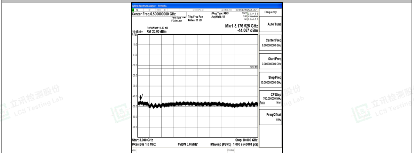
Band12_3MHz_16QAM_23025_1RB#0_3000~10000_3000~10000
