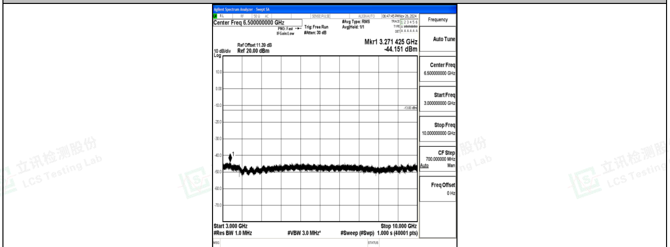
Band12_1.4MHz_16QAM_23017_1RB#0_3000~10000_3000~10000
