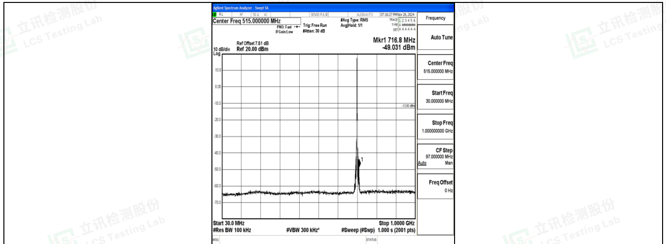
Band12_3MHz_16QAM_23095_1RB#0_30~1000_30~1000
