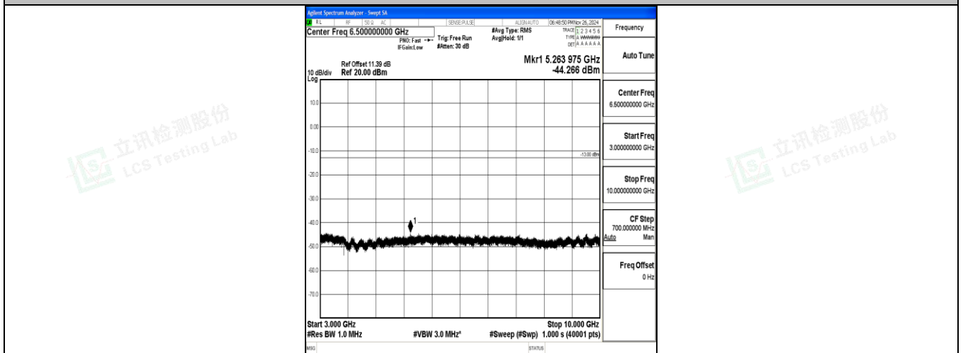
Band12_1.4MHz_16QAM_23095_1RB#0_3000~10000_3000~10000
