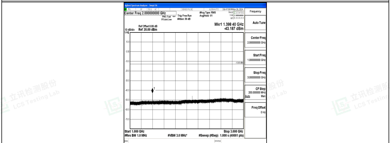
Band12_1.4MHz_QPSK_23017_1RB#0_1000~3000_1000~3000
