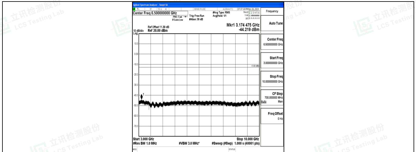
Band12_5MHz_QPSK_23095_1RB#0_3000~10000_3000~10000
