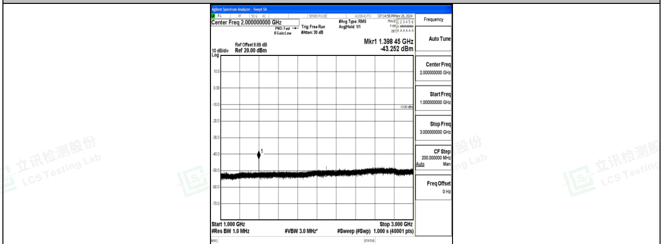
Band12_3MHz_QPSK_23025_1RB#0_1000~3000_1000~3000
