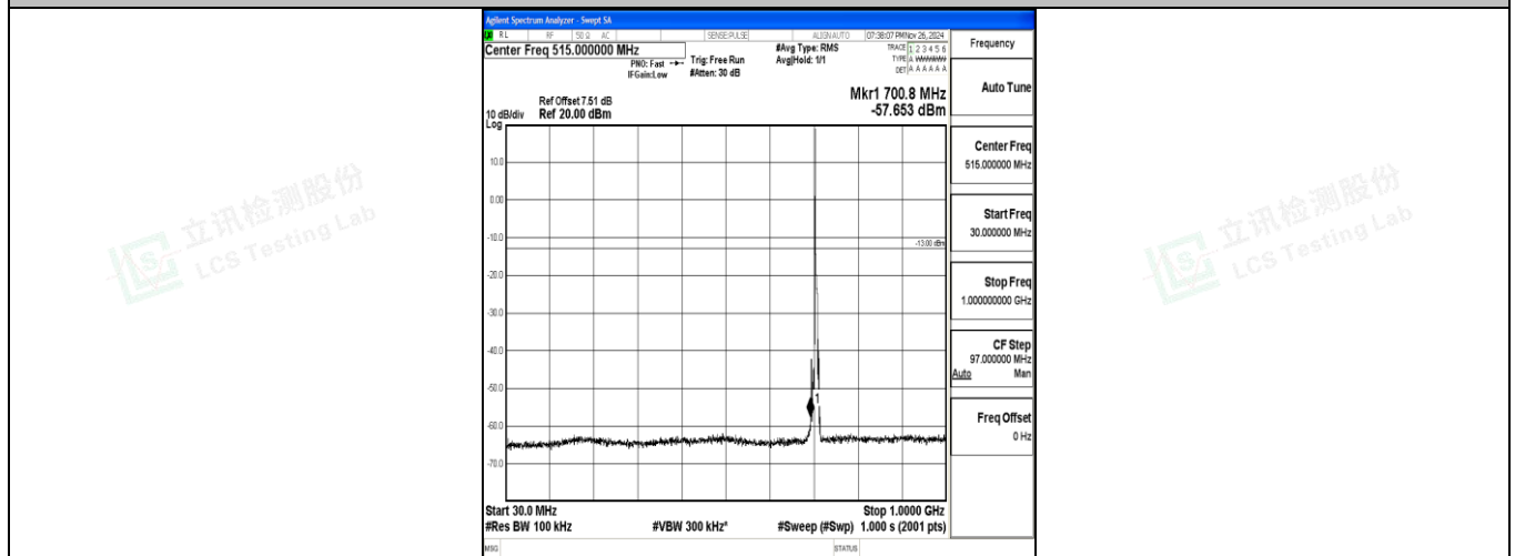
Band12_5MHz_QPSK_23155_1RB#0_30~1000_30~1000
