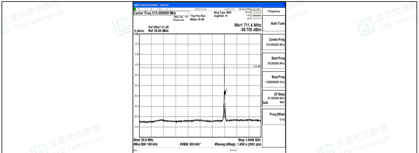
Band12_1.4MHz_16QAM_23095_1RB#0_30~1000_30~1000
