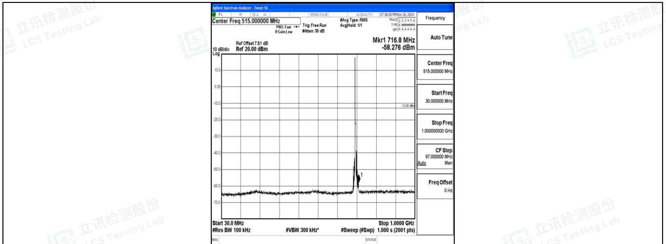
Band12_5MHz_QPSK_23035_1RB#0_30~1000_30~1000
