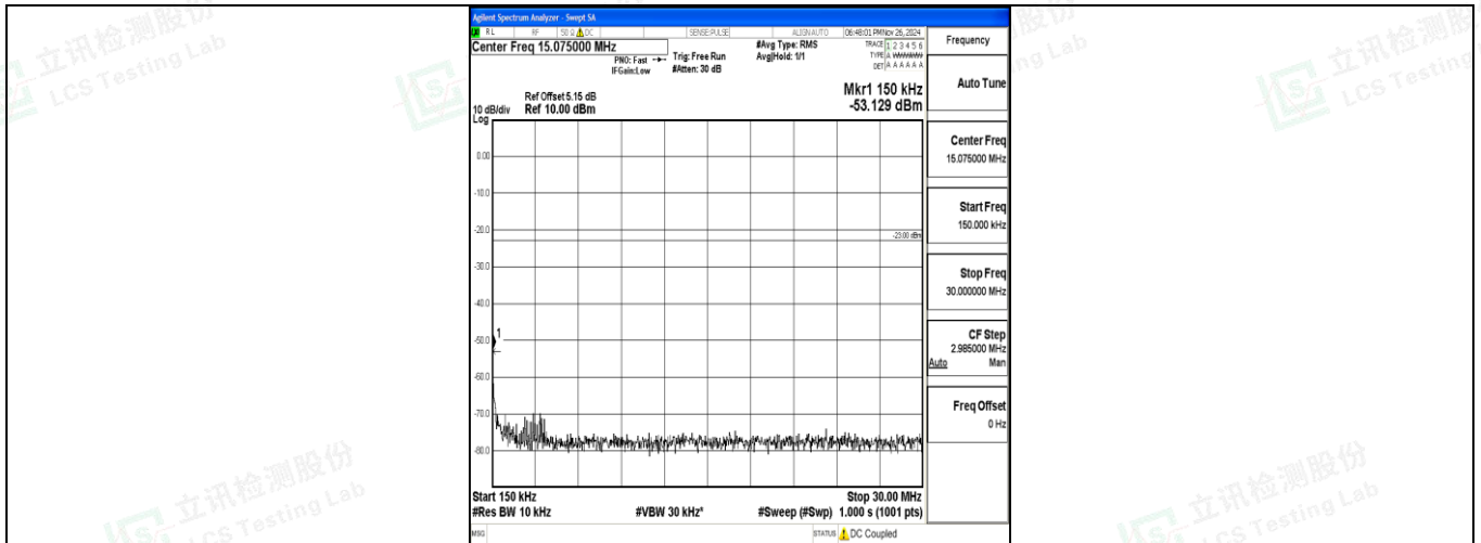
Band12_1.4MHz_QPSK_23095_1RB#0_0.15~30_0.15~30
