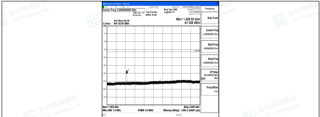
Band12_1.4MHz_QPSK_23173_1RB#0_1000~3000_1000~3000
