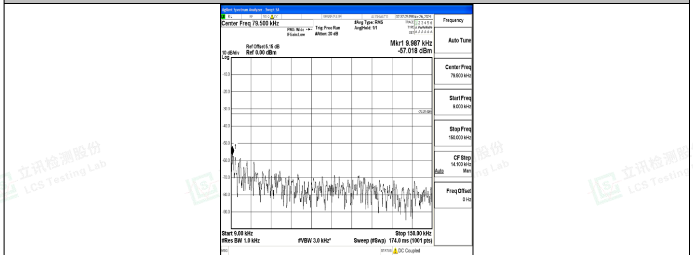
Band12_5MHz_16QAM_23095_1RB#0_0.009~0.15_0.009~0.15
