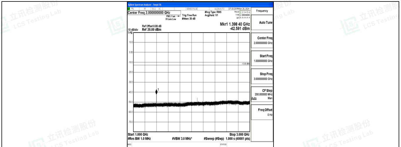
Band12_3MHz_16QAM_23025_1RB#0_1000~3000_1000~3000
