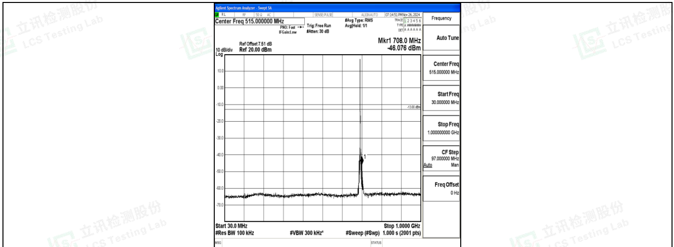
Band12_3MHz_QPSK_23025_1RB#0_30~1000_30~1000
