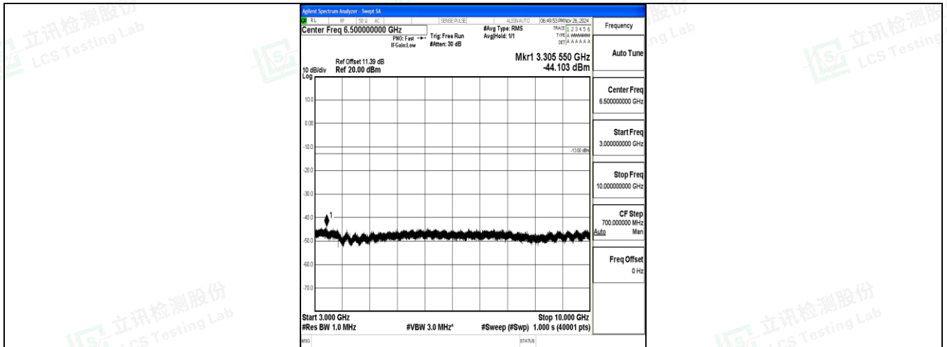
Band12_1.4MHz_16QAM_23173_1RB#0_3000~10000_3000~10000
