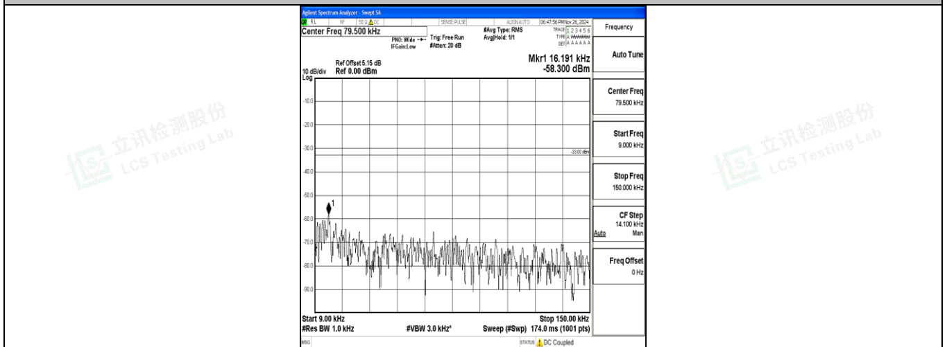
Band12_1.4MHz_QPSK_23095_1RB#0_0.009~0.15_0.009~0.15
