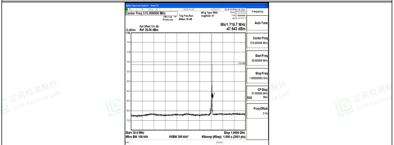
Band12_1.4MHz_16QAM_23173_1RB#0_30~1000_30~1000
