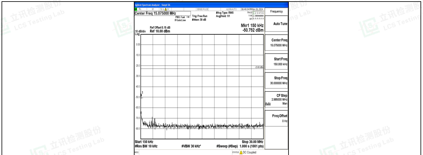
Band12_1.4MHz_16QAM_23173_1RB#0_0.15~30_0.15~30
