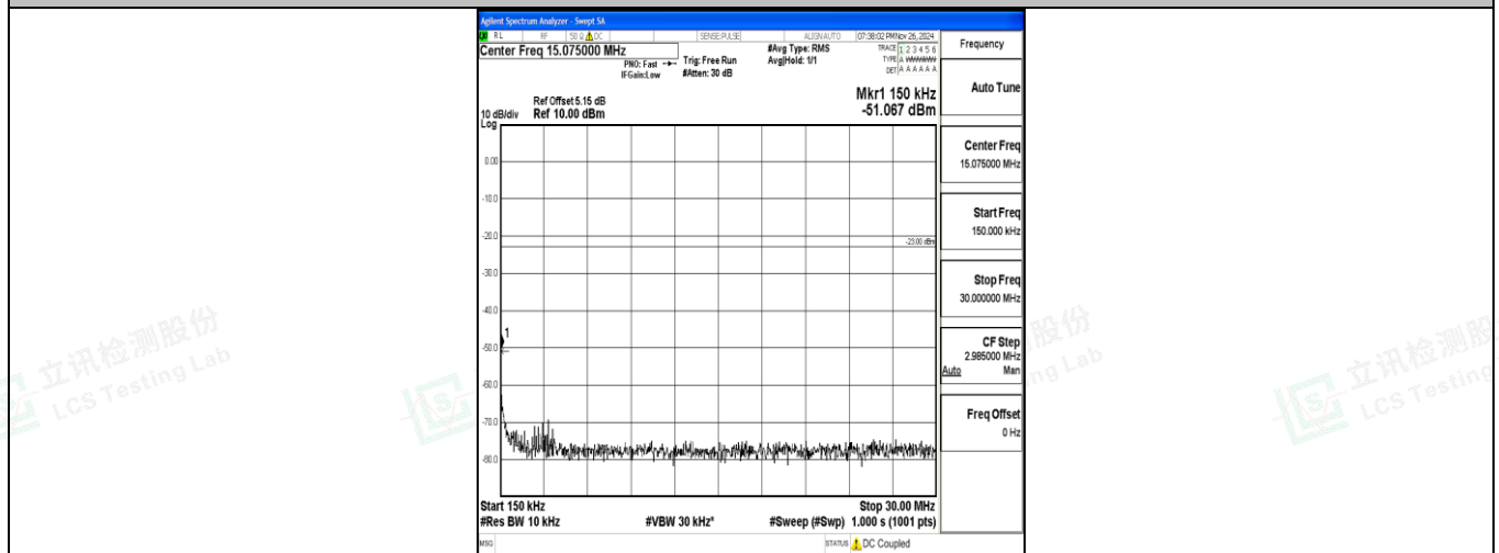
Band12_5MHz_QPSK_23155_1RB#0_0.15~30_0.15~30
