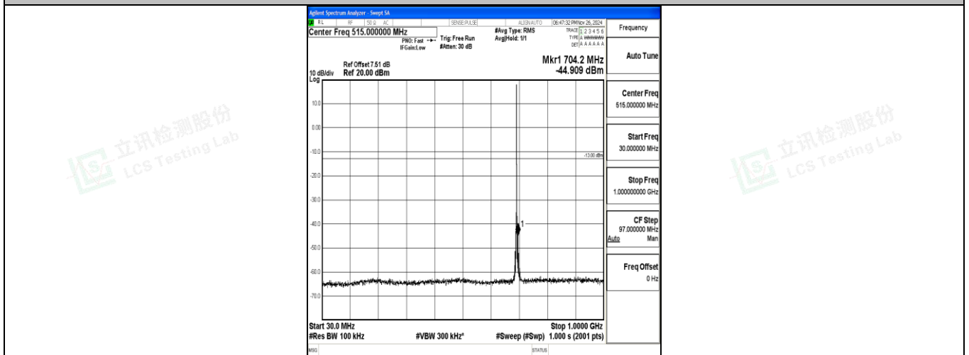
Band12_1.4MHz_16QAM_23017_1RB#0_30~1000_30~1000
