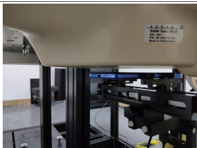
Body-worn Rear(10mm)
