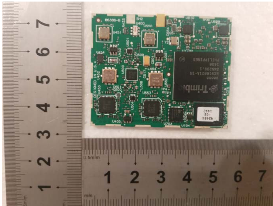
EUT – Cut Off View-5
