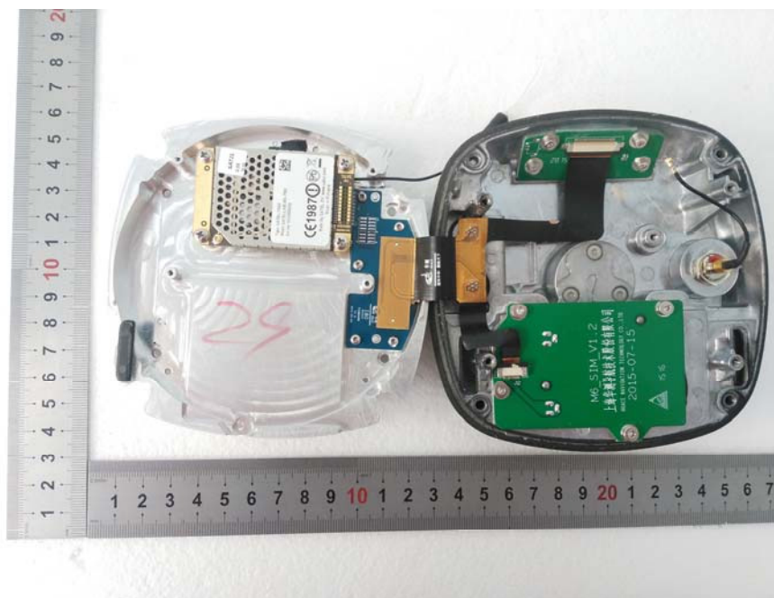
EUT – Cut Off View-5
