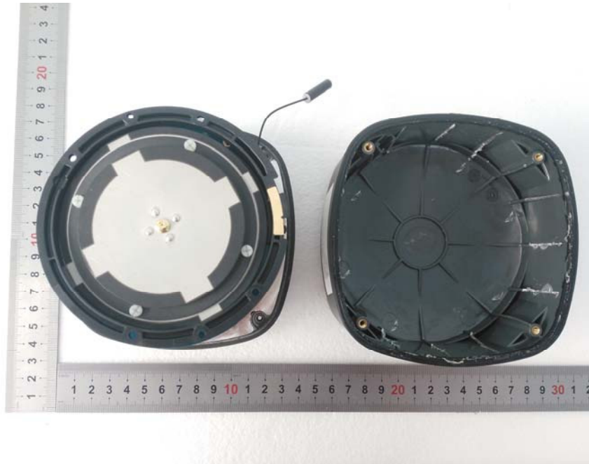
EUT – Cut Off View-2
