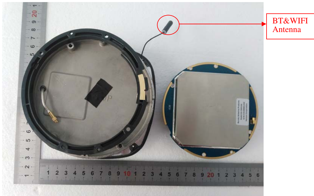
EUT – Cut Off View-2
