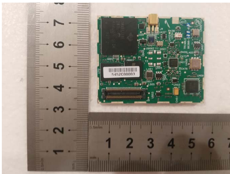
EUT – Main Board 3 Cut off View-1
