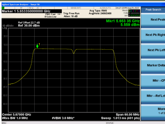
Channel 134 (5670MHz)
