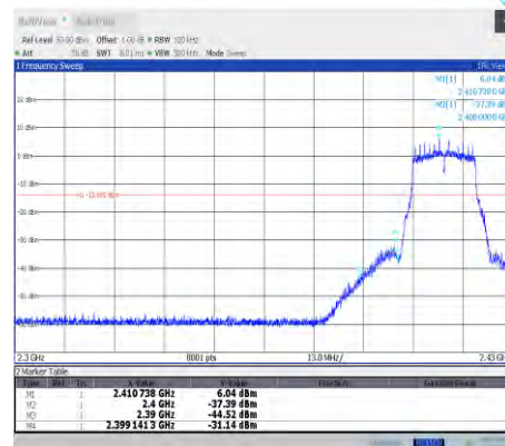
11g-CDD-Ant8-2412
