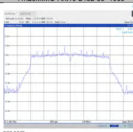
11n20MIMO-Ant8-2462-0~Reference
