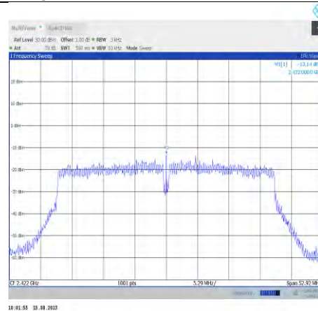
11n40MIMO-Ant8-2422
