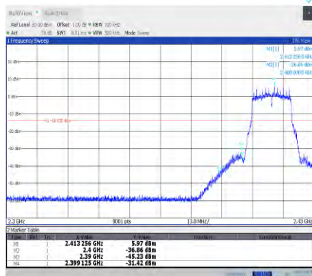
11g-CDD-Ant10-2412
