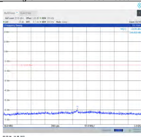
11g-CDD-Ant8-2437-30~1000
