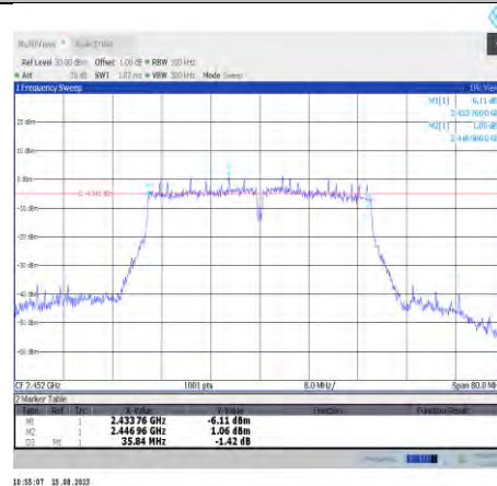
11n40MIMO-Ant8-2452
