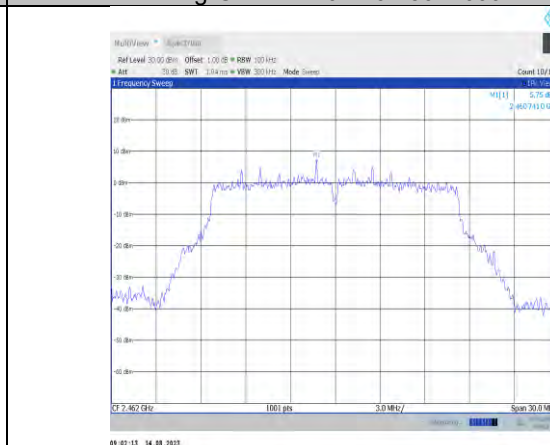
11g-CDD-Ant8-2462-0~Reference
