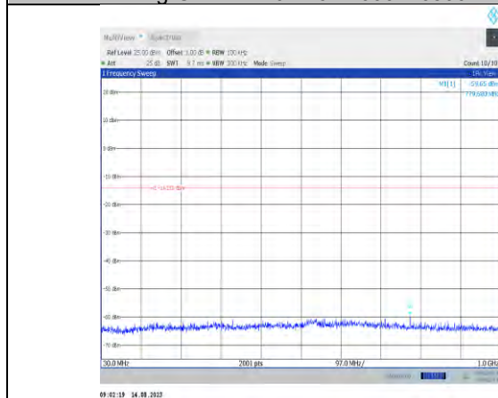
11g-CDD-Ant8-2462-30~1000
