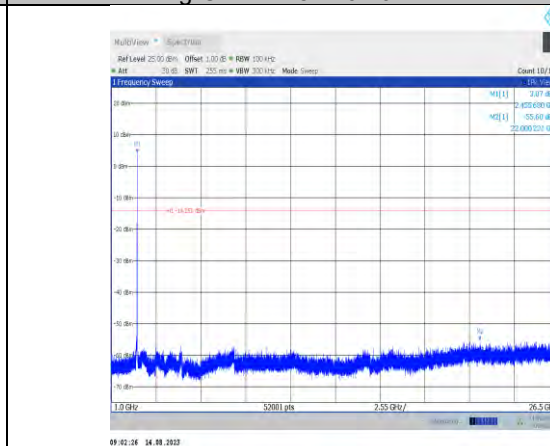
11g-CDD-Ant8-2462-1000~26500
