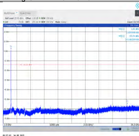
11g-CDD-Ant10-2437-1000~26500
