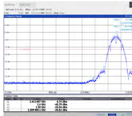
11b-CDD-Ant8-2412
