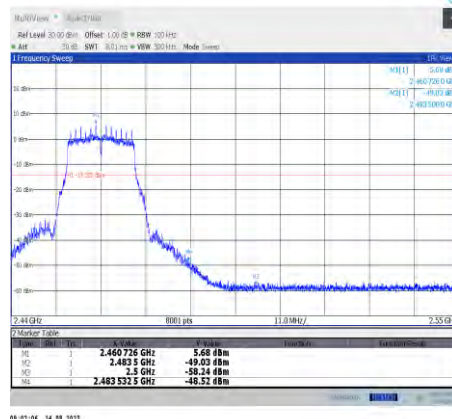
11g-CDD-Ant8-2462
