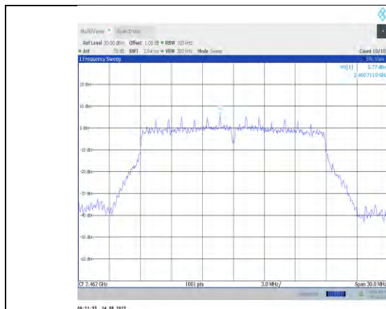
11n20MIMO-Ant10-2462-0~Reference
