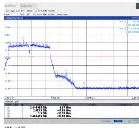
11n40MIMO-Ant8-2452
