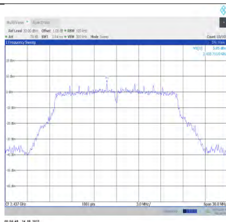
11g-CDD-Ant10-2437-0~Reference
