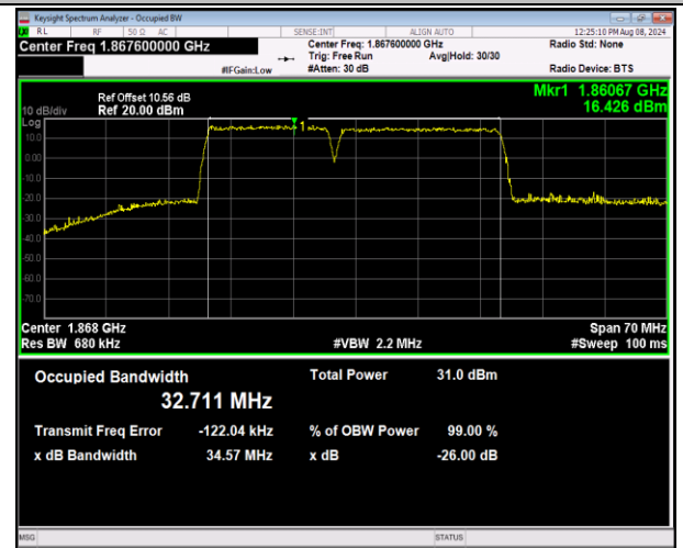
2-2-15MHz-20MHz-QPSK-QPSK-18678-18849-75RB#0-100 100RB#0-PASS
