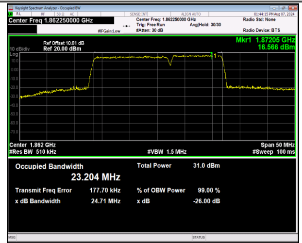
2-2-15MHz-10MHz-QPSK-QPSK-18675-18795-75RB#0-50RB#0-PASS
