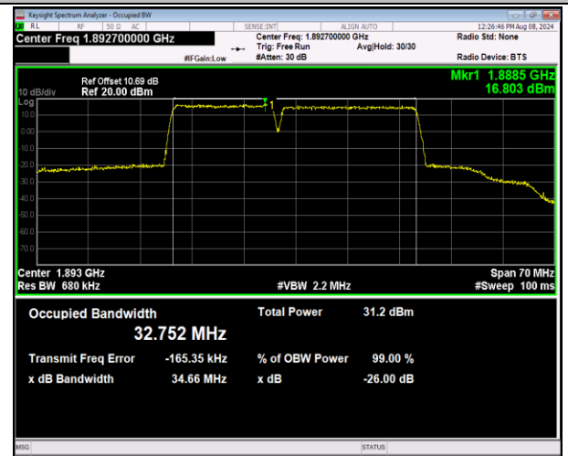
2-2-15MHz-20MHz-QPSK-QPSK-18929-19100-75RB#0- 100RB#0-PASS
