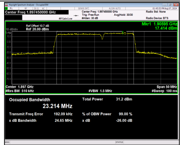
2-2-15MHz-10MHz-QPSK-QPSK-19027-19147-75RB#0- 50RB#0-PASS
