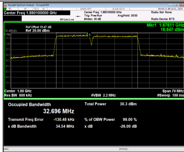
2-2-15MHz-20MHz-64QAM-64QAM-18803-18974-75RB# 0-100RB#0-PASS
