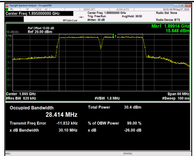
2-2-15MHz-15MHz-16QAM-16QAM-18975-19125-75RB#0-7 #0-75RB#0-PASS
