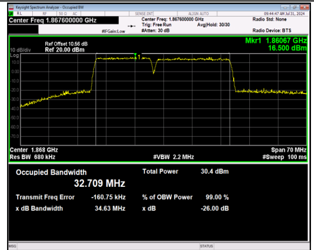
2-2-15MHz-20MHz-64QAM-64QAM-18678-18849-75RB#0-100 #0-100RB#0-PASS
