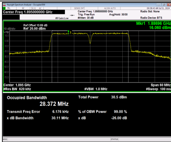
2-2-15MHz-15MHz-64QAM-64QAM-18975-19125-75RB#0-7 0-75RB#0-PASS
