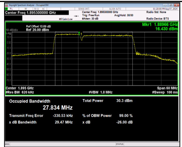
2-2-10MHz-20MHz-16QAM-16QAM-18956-19100-50RB#0-100RB#0-PASS
