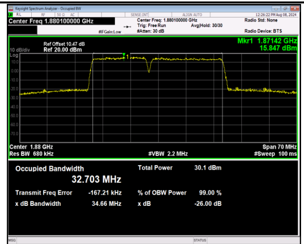
2-2-15MHz-20MHz-16QAM-16QAM-18803-18974-75RB #0-100RB#0-PASS
