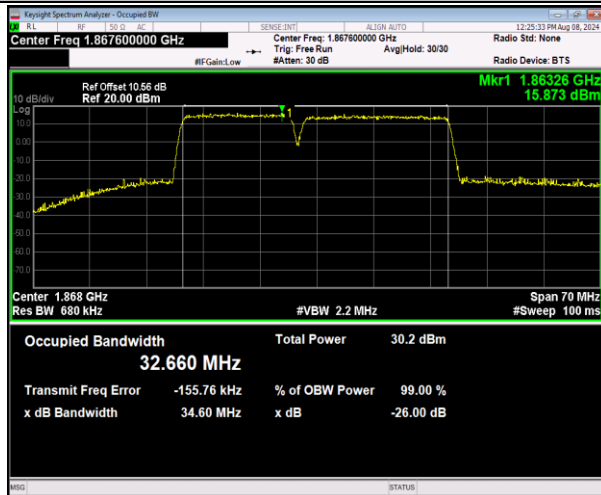
2-2-15MHz-20MHz-16QAM-16QAM-18678-18849-75RB#0-100 0-100RB#0-PASS
