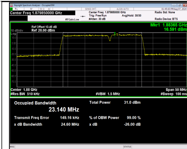
2-2-15MHz-10MHz-QPSK-QPSK-18851-18971-75RB#0-5 ORB#0-PASS
