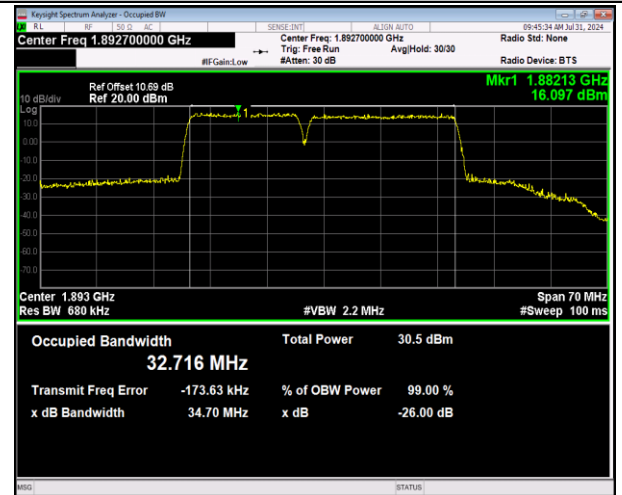
2-2-15MHz-20MHz-64QAM-64QAM-18929-19100-75RB #0-100RB#0-PASS
