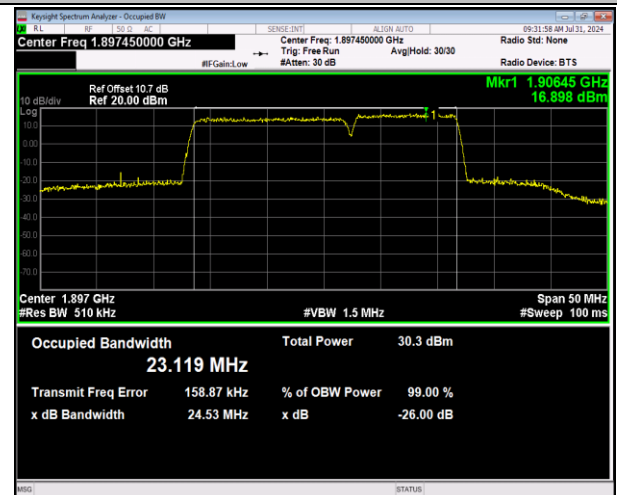
2-2-15MHz-10MHz-64QAM-64QAM-19027-19147-75RB #0-50RB#0-PASS
