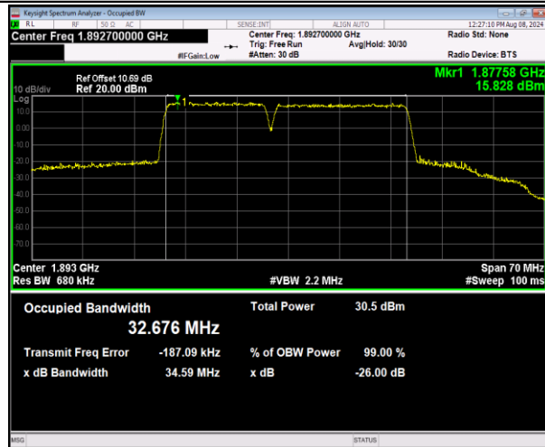
2-2-15MHz-20MHz-16QAM-16QAM-18929-19100-75RB# 0-100RB#0-PASS
