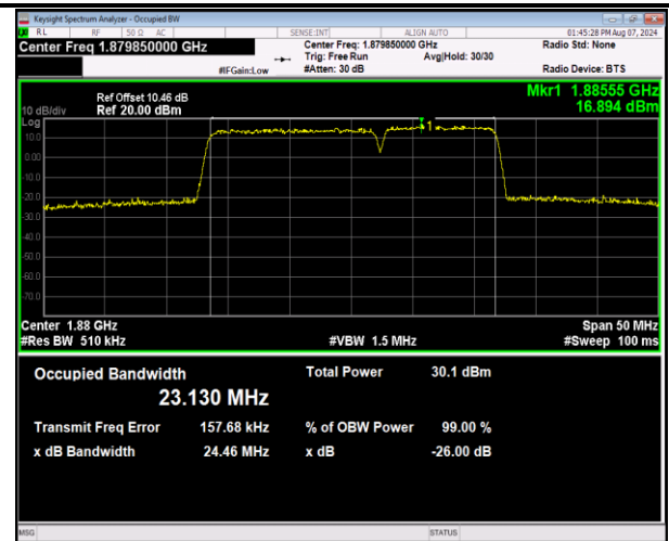
2-2-15MHz-10MHz-16QAM-16QAM-18851-18971-75RB #0-50RB#0-PASS
