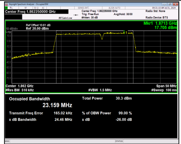
2-2-15MHz-10MHz-64QAM-64QAM-18675-18795-75RB#0-50RB#0-PASS
