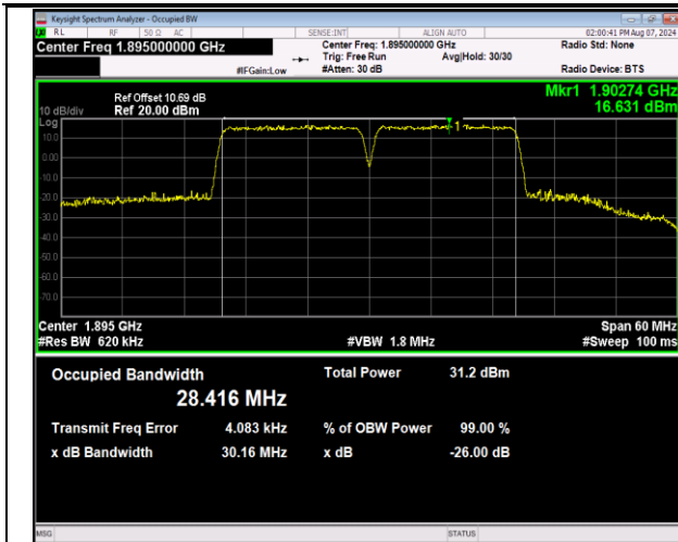
2-2-15MHz-15MHz-QPSK-18975-19125-75RB#0-7 5RB#0-PASS
