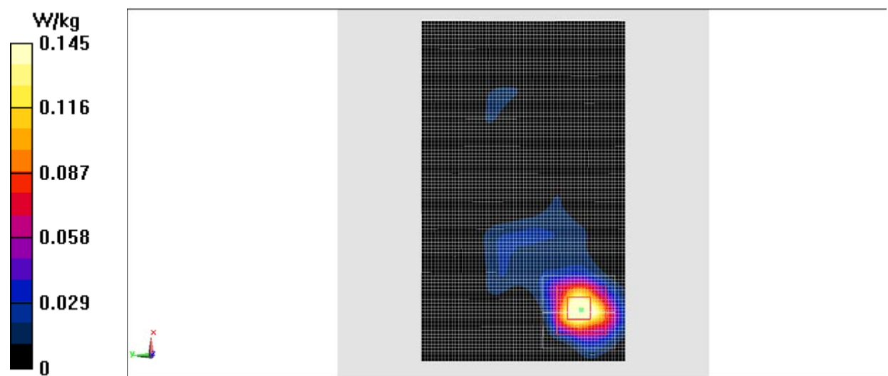
Fig.12 2450 MHz
