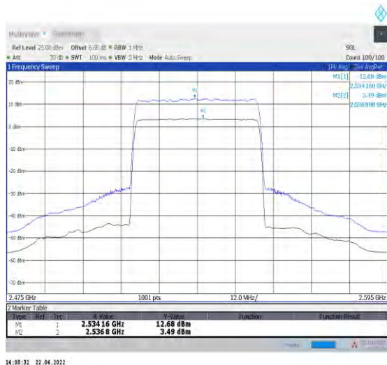
1-N7--15-40-M-1-DFT-256QAM-Outer_Full-216@0-A nt0-9.19-100%-0.00-9.19-PASS-≤13
