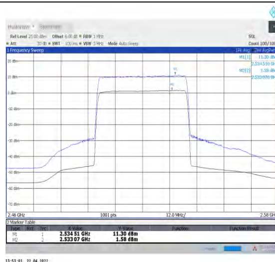
1-N7--15-40-L-2-CP-256QAM-Outer_Full-216@0-An t0-9.72-100%-0.00-9.72-PASS-≤13
