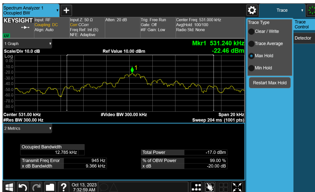
Plot 7-4. Occupied Bandwidth Measurement _ Click
