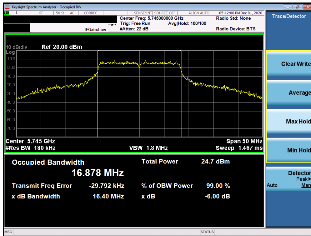
Plot 7-115. 6dB Bandwidth Plot SISO ANT2 (802.11a) (UNII Band 3) – Ch. 149
