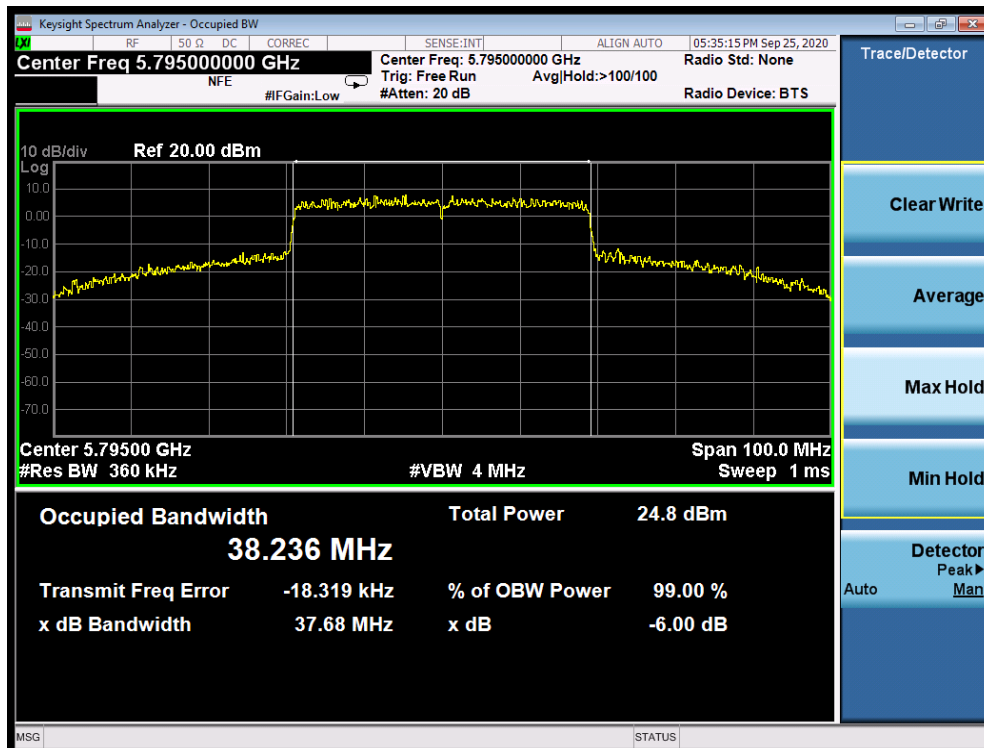
Plot 7-112. 6dB Bandwidth Plot SISO ANT1 (40MHz BW 802.11ax (UNII Band 3) – Ch. 159)
