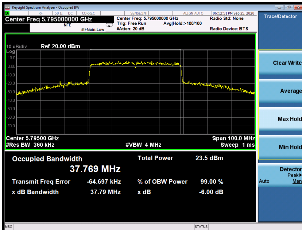
Plot 7-127. 6dB Bandwidth Plot SISO ANT2 (40MHz BW 802.11ax (UNII Band 3) – Ch. 159)
