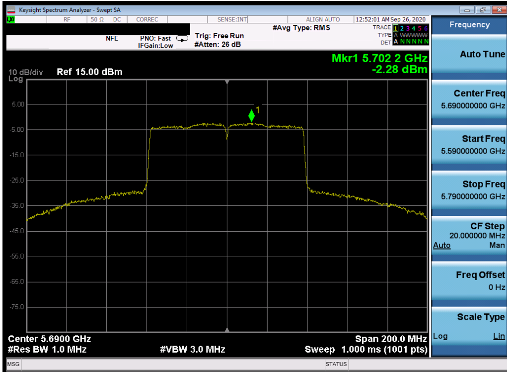
Plot 7-177. Power Spectral Density Plot SISO ANT1 (80MHz BW 802.11ac (UNII Band 2C) – Ch. 138)
