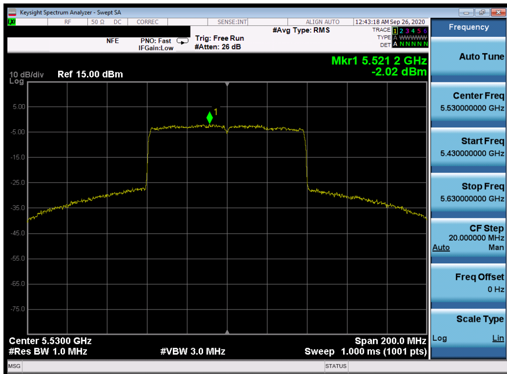
Plot 7-178. Power Spectral Density Plot SISO ANT1 (80MHz BW 802.11ax (UNII Band 2C) – Ch. 106)
