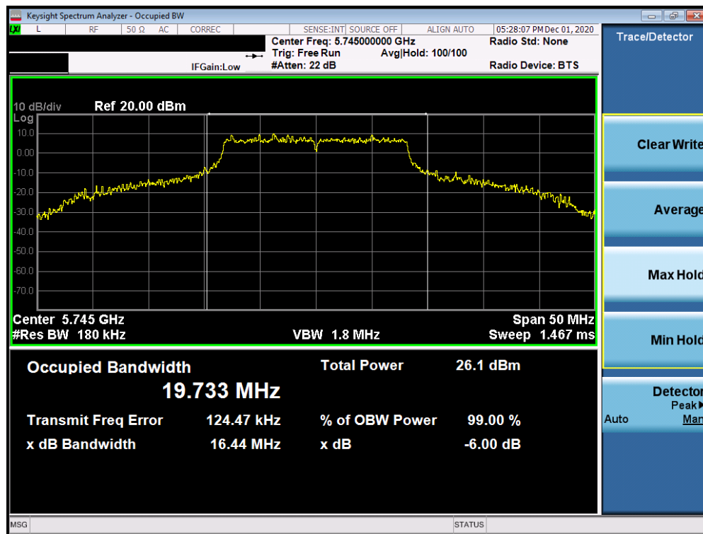
Plot 7-100. 6dB Bandwidth Plot SISO ANT1 (802.11a (UNII Band 3) – Ch. 149)
