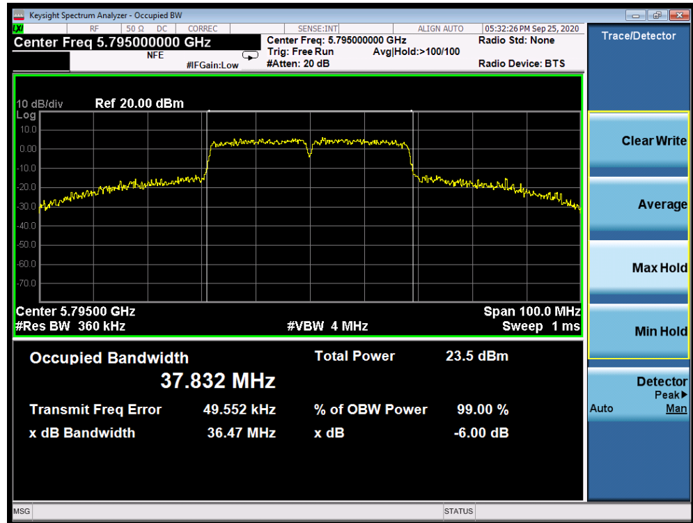
Plot 7-110. 6dB Bandwidth Plot SISO ANT1 (40MHz BW 802.11n (UNII Band 3) – Ch. 159)
