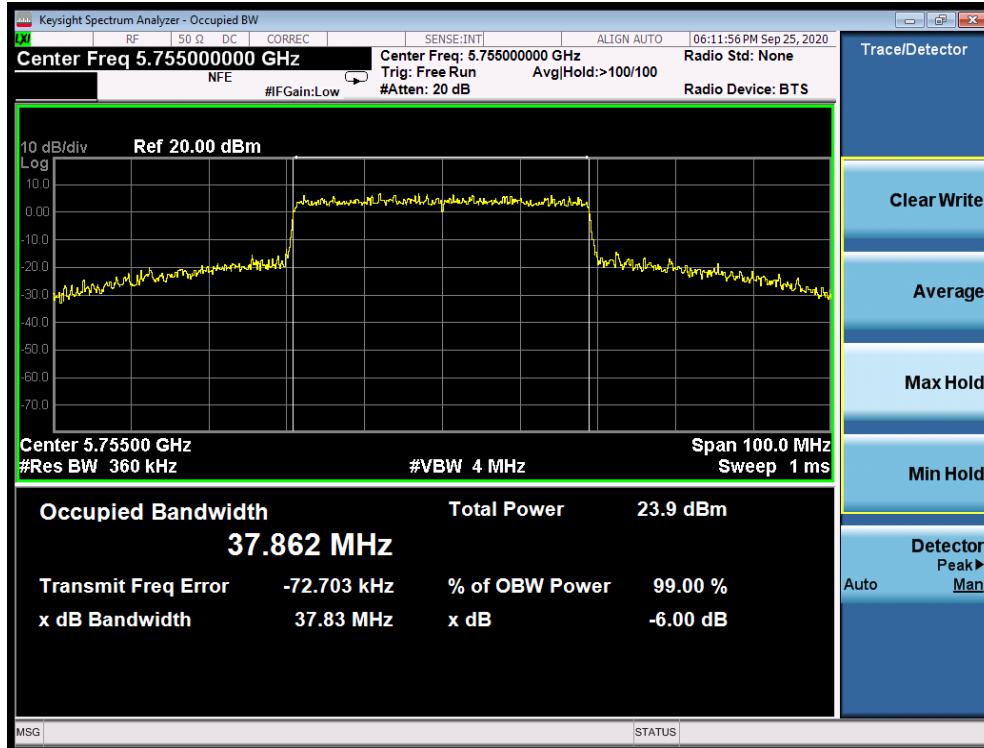
Plot 7-126. 6dB Bandwidth Plot SISO ANT2 (40MHz BW 802.11ax (UNII Band 3) – Ch. 151)
