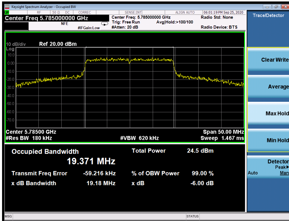
Plot 7-122. 6dB Bandwidth Plot SISO ANT2 (20MHz BW 802.11ax (UNII Band 3) – Ch. 157)
