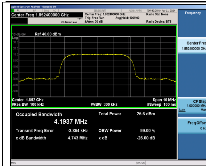
Band2-9262-4.743
