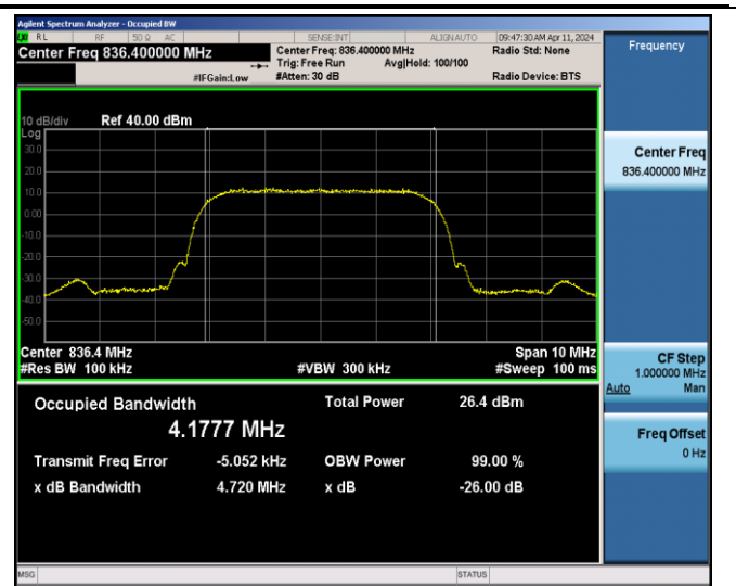
Band5-4182-4.720
