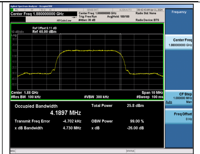
Band2-9400-4.730
