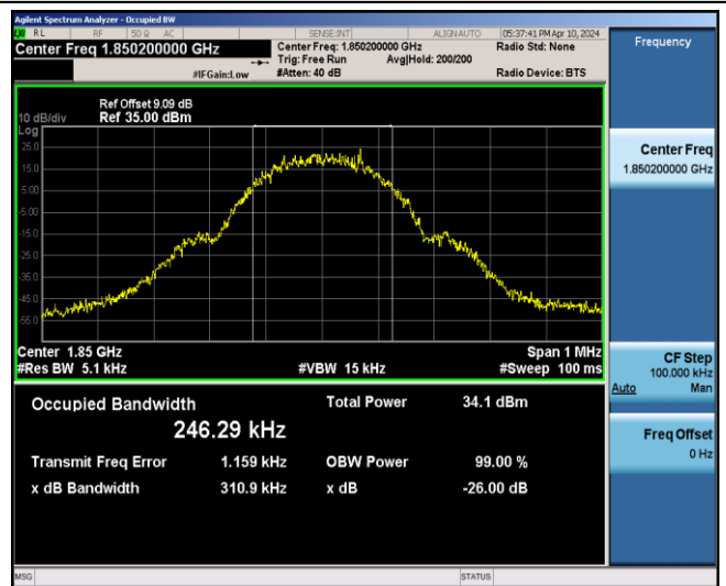
GSM1900-512-0-0.3109
