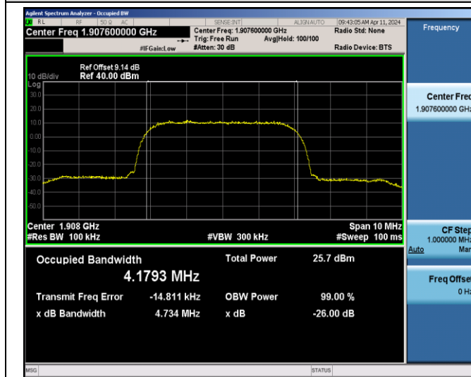
Band2-9538-4.734
