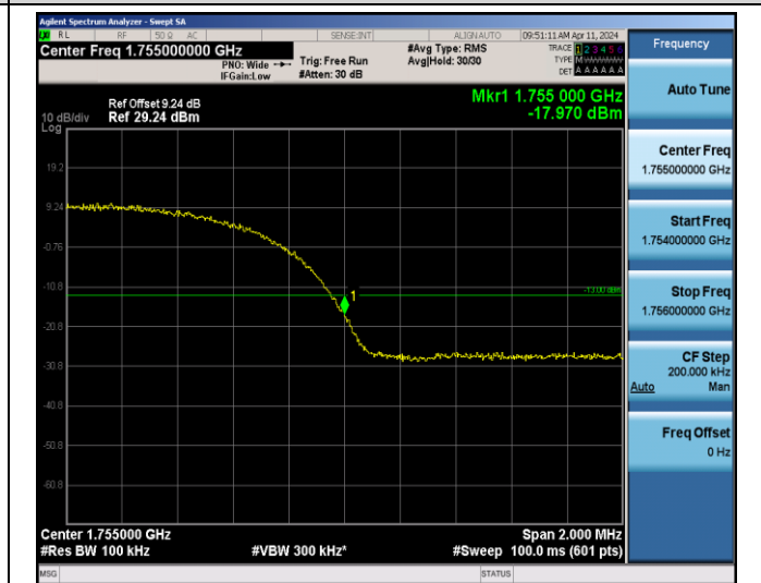
Band4-1513
