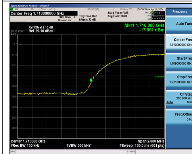
Band4-1312
