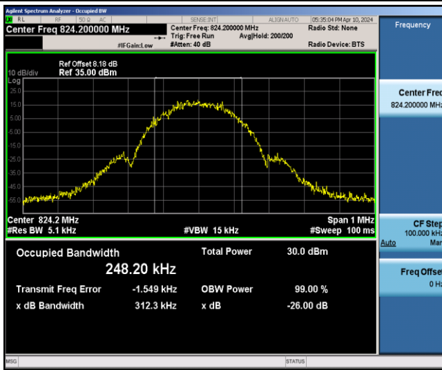
EGPRS850-128-8-0.3123
