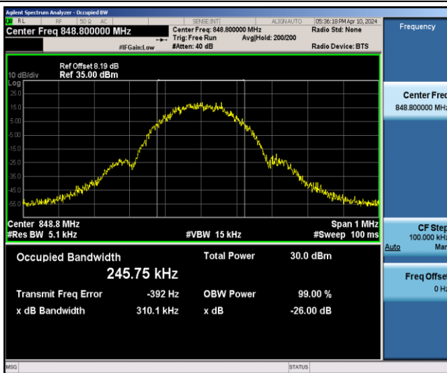
EGPRS850-251-8-0.3101
