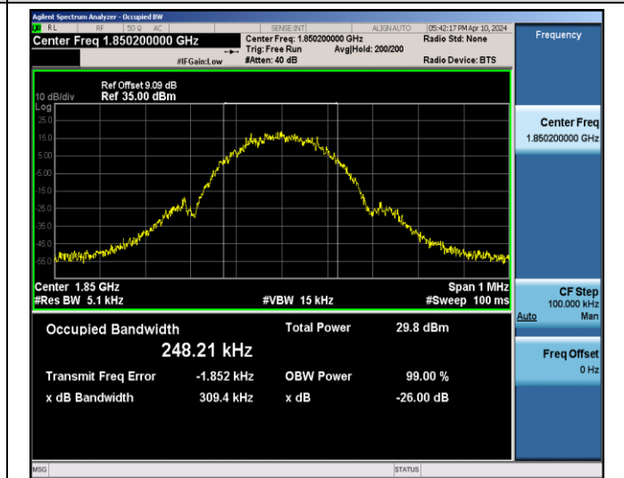
EGPRS1900-512-2-0.3094
