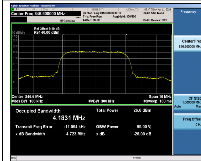
Band5-4233-4.723
