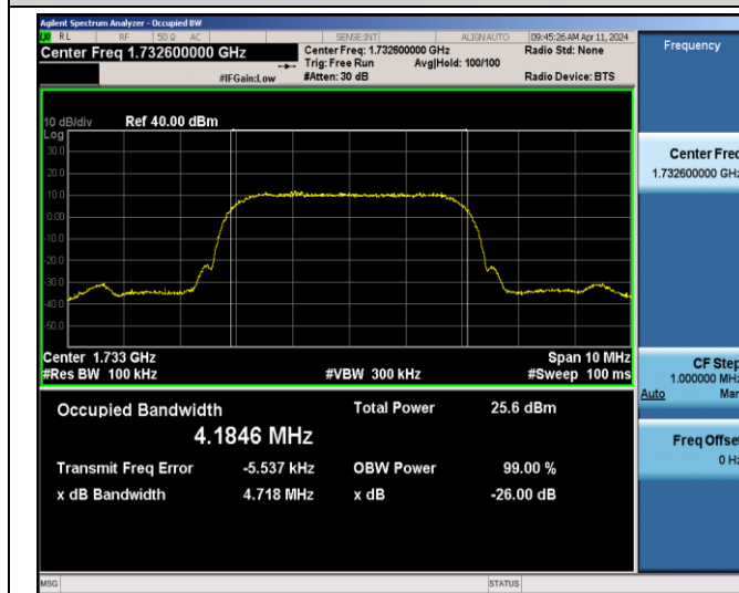
Band4-1413-4.718
