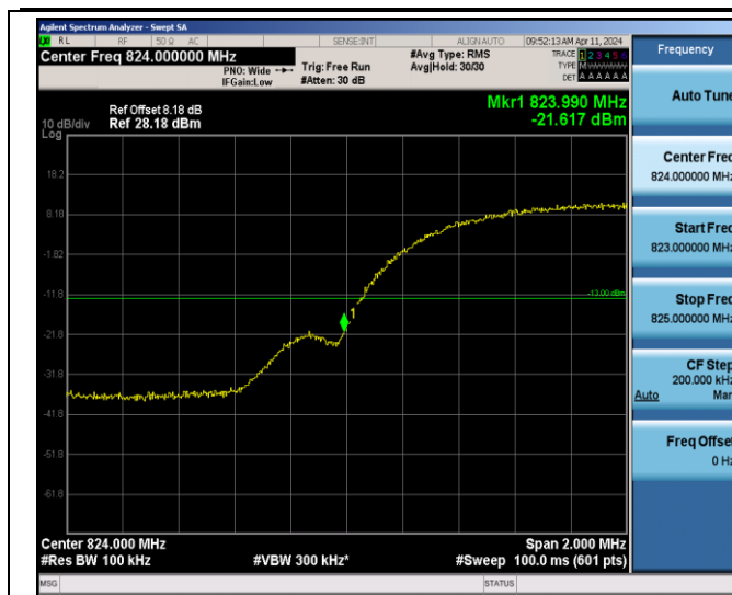
Band5-4132
