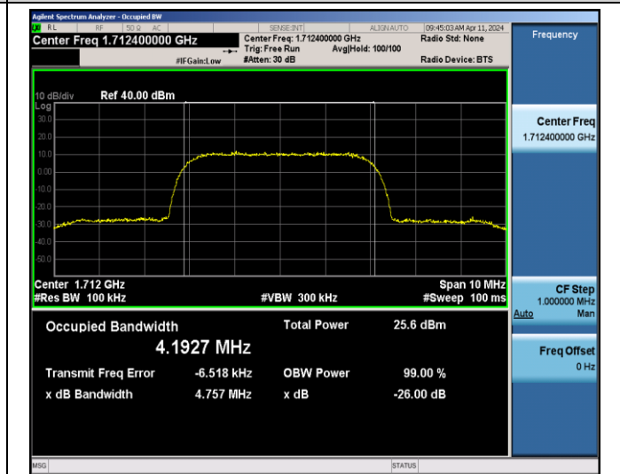
Band4-1312-4.757
