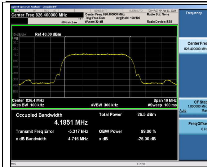
Band5-4132-4.716
