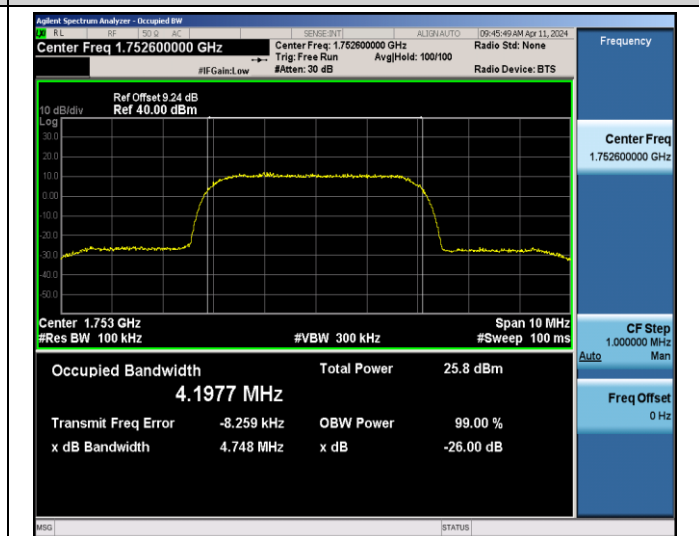
Band4-1513-4.748
