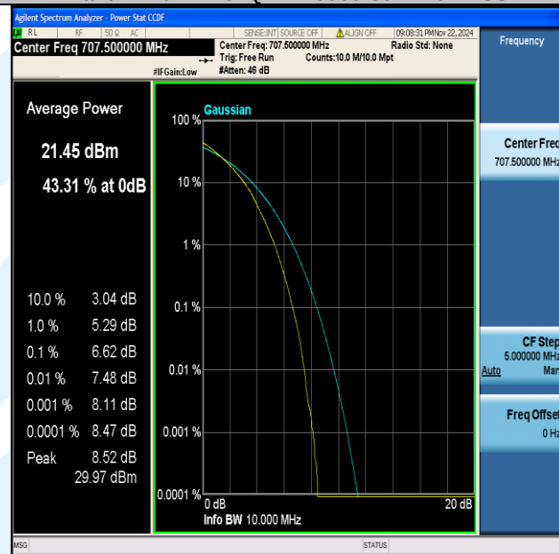
Band12-10MHz-64QAM-23095-50RB#0-PASS
