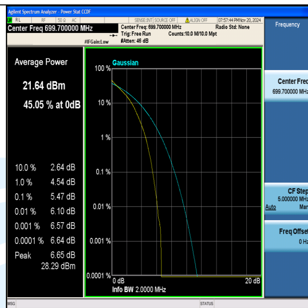
Band12-1.4MHz-QPSK-23017-6RB#0-PASS
