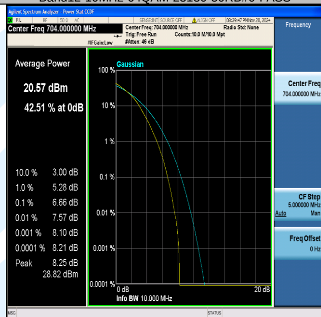
Band12-10MHz-16QAM-23060-50RB#0-PASS
