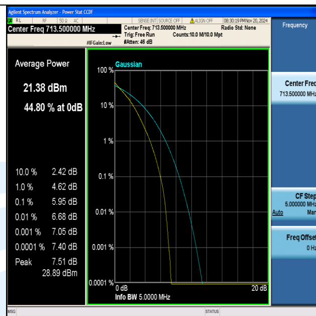
Band12-5MHz-QPSK-23155-25RB#0-PASS
