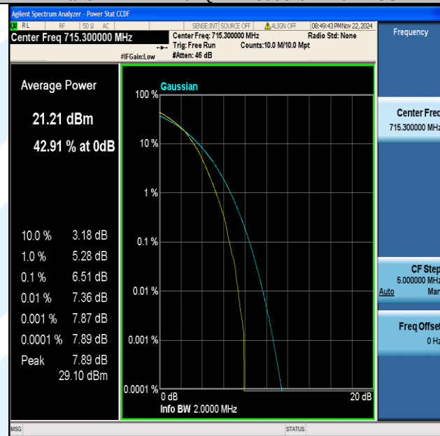
Band12-1.4MHz-64QAM-23173-6RB#0-PASS
