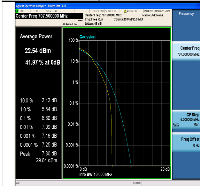
Band12-10MHz-64QAM-23095-1RB#0-PASS
