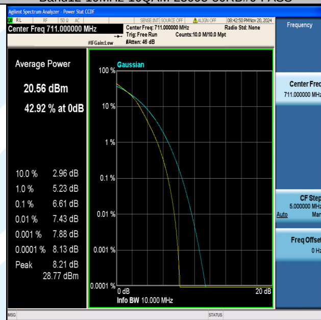
Band12-10MHz-16QAM-23130-50RB#0-PASS
