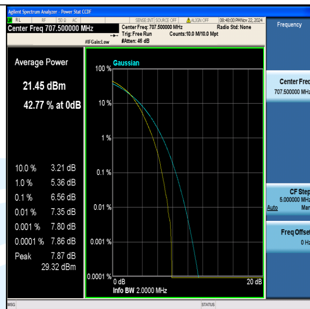
Band12-1.4MHz-64QAM-23095-6RB#0-PASS
