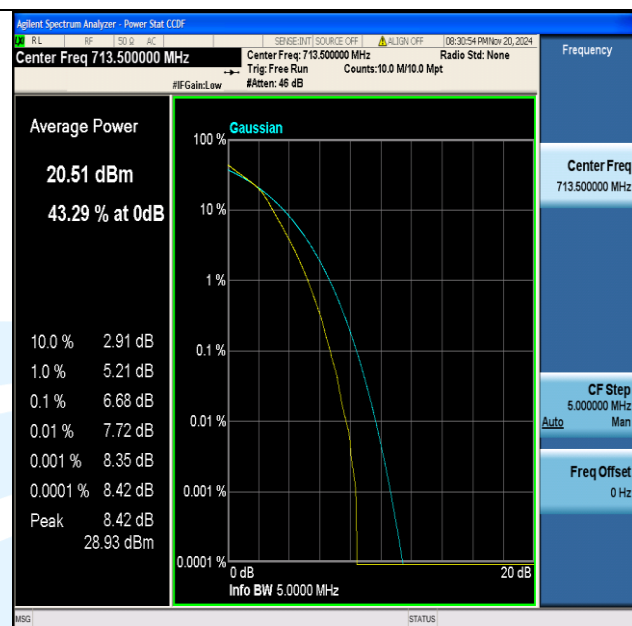
Band12-5MHz-16QAM-23155-25RB#0-PASS
