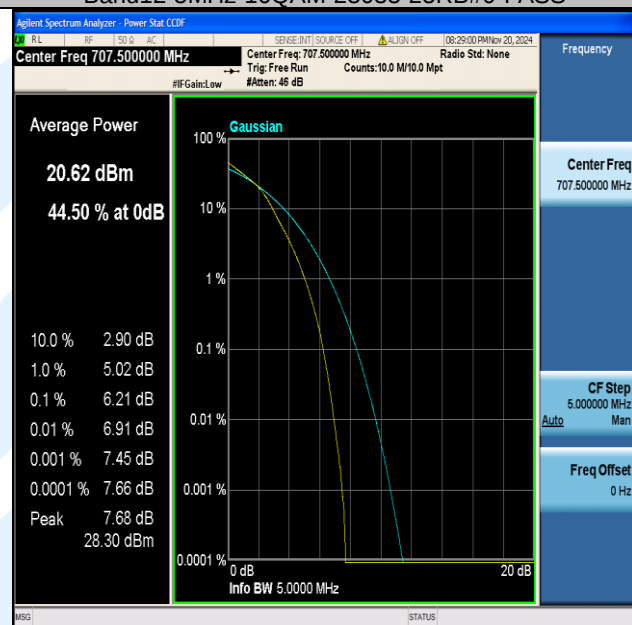
Band12-5MHz-16QAM-23095-25RB#0-PASS
