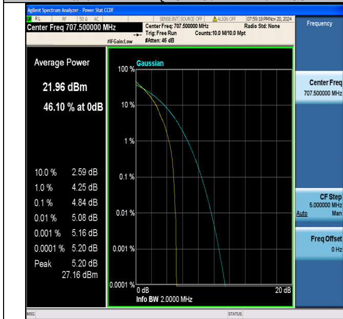
Band12-1.4MHz-QPSK-23095-1RB#0-PASS
