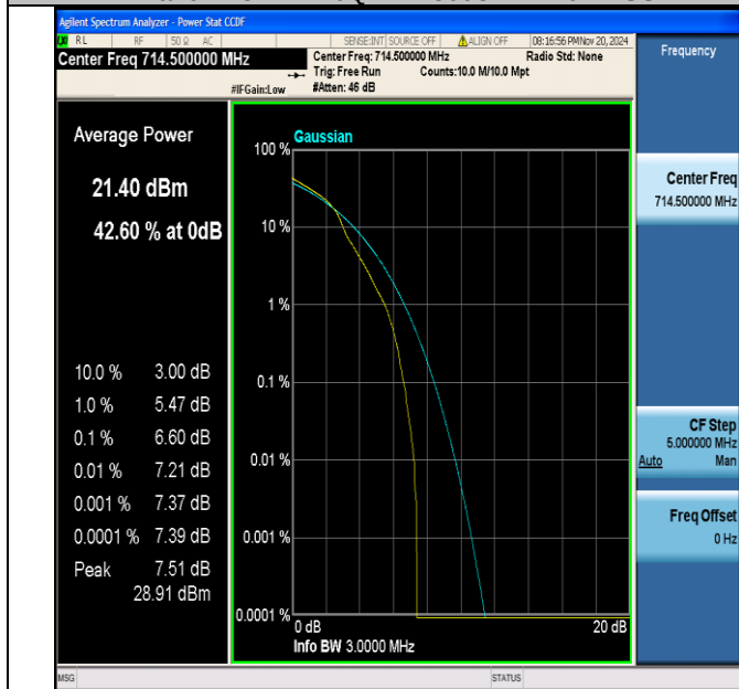
Band12-3MHz-16QAM-23165-1RB#0-PASS
