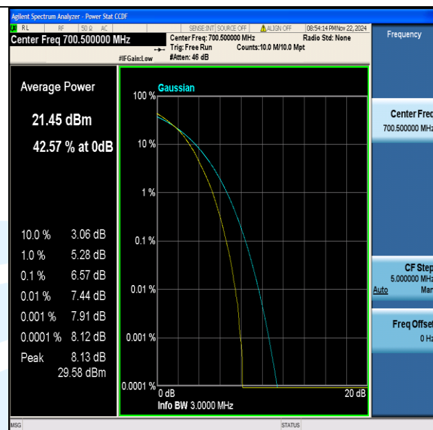
Band12-3MHz-64QAM-23025-15RB#0-PASS
