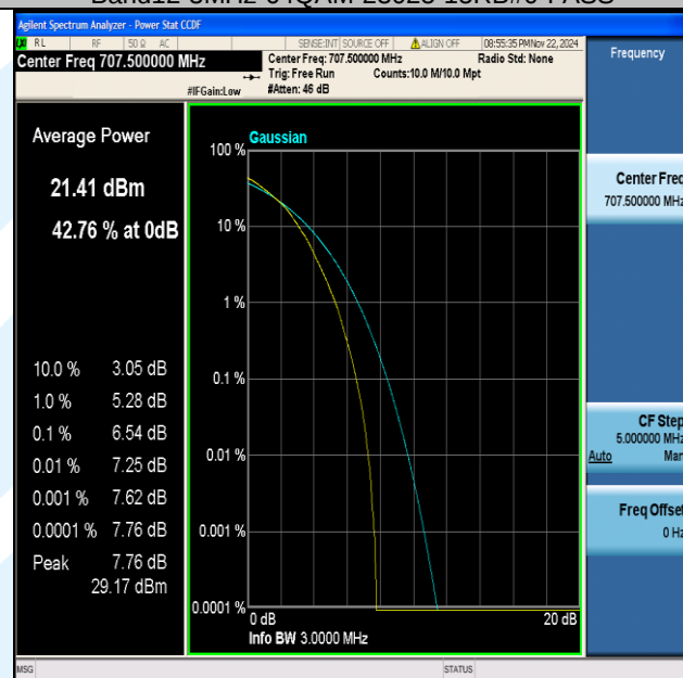
Band12-3MHz-64QAM-23095-15RB#0-PASS
