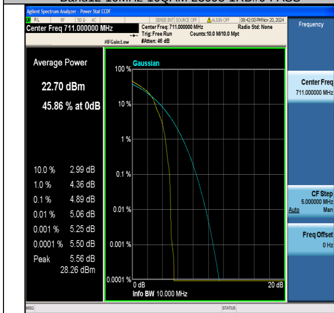
Band12-10MHz-16QAM-23130-1RB#0-PASS
