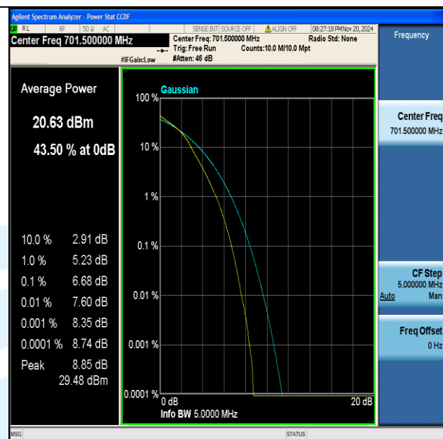
Band12-5MHz-16QAM-23035-25RB#0-PASS
