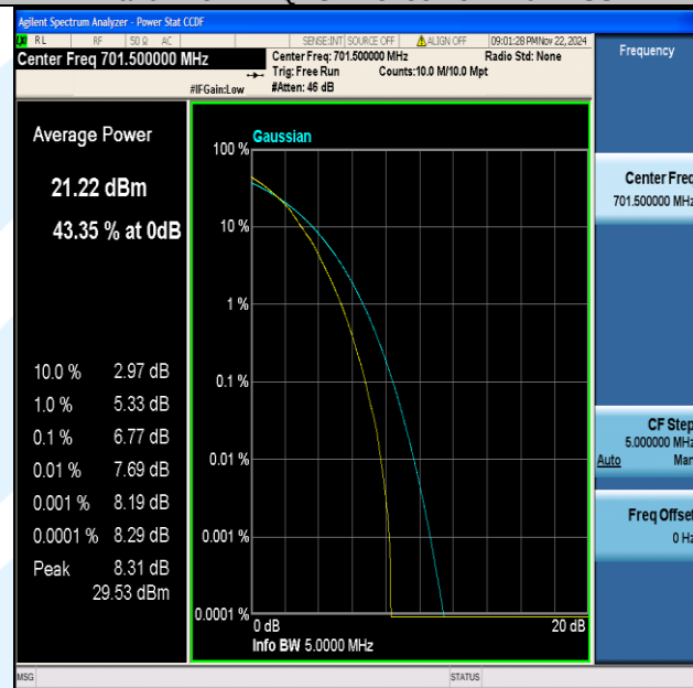
Band12-5MHz-64QAM-23035-25RB#0-PASS
