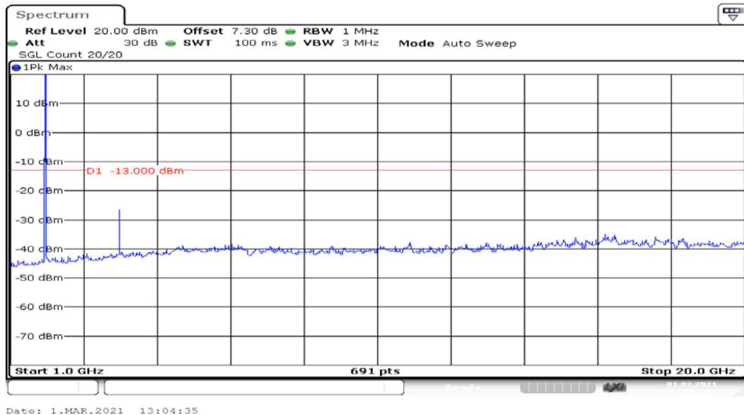
Channel 9400 1GHz~20GHz(dBm)
