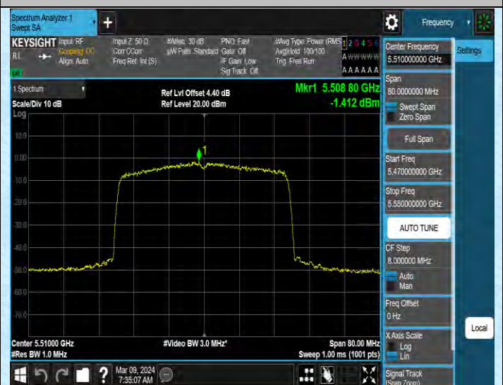
11AX40SISO-Ant2-5510-PASS
