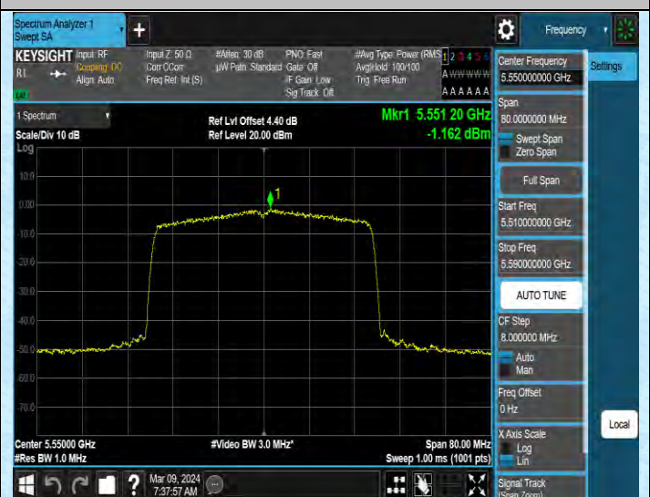
11AX40SISO-Ant2-5550-PASS
