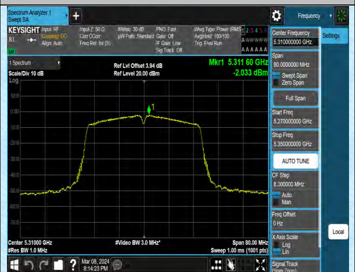
11AC40SISO-Ant2-5310-PASS
