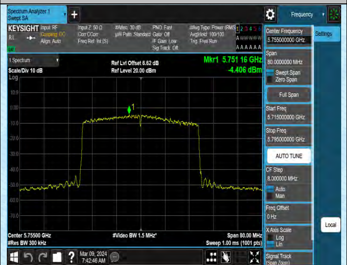
11AX40SISO-Ant2-5755-PASS
