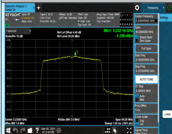
11AX40SISO-Ant1-5230-PASS
