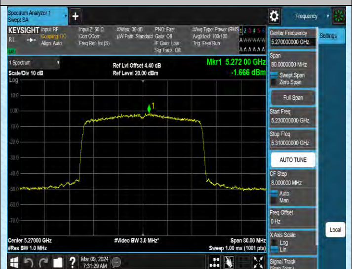
11AX40SISO-Ant2-5270-PASS
