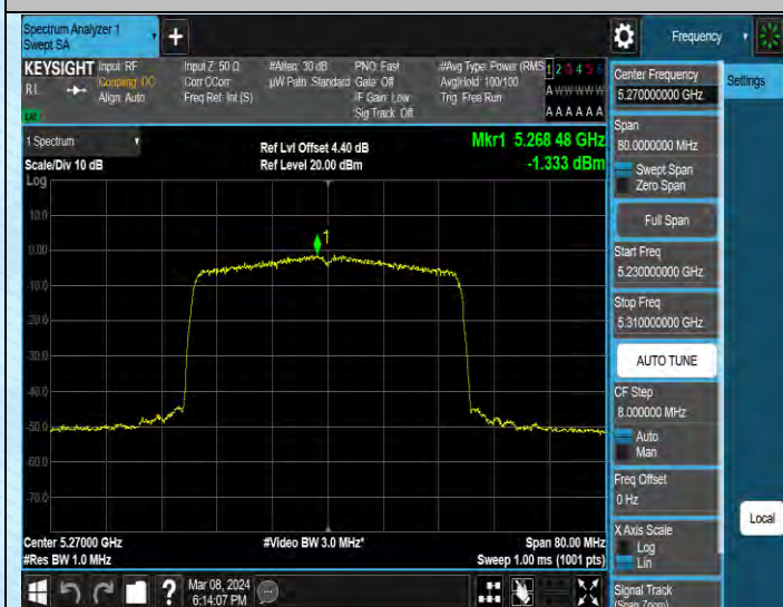
11AX40SISO-Ant1-5270-PASS
