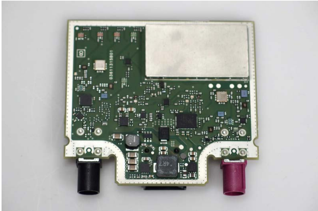
PCB Bottom Side (with shielding cover):
