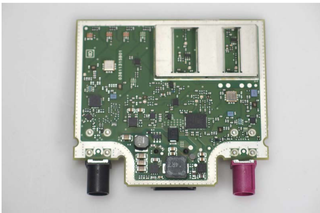
PCB Bottom Side (without shielding cover):
