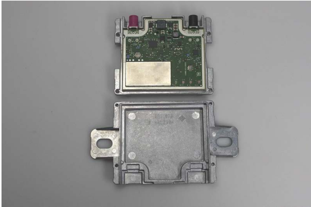
Bottom Cover with PCB:
