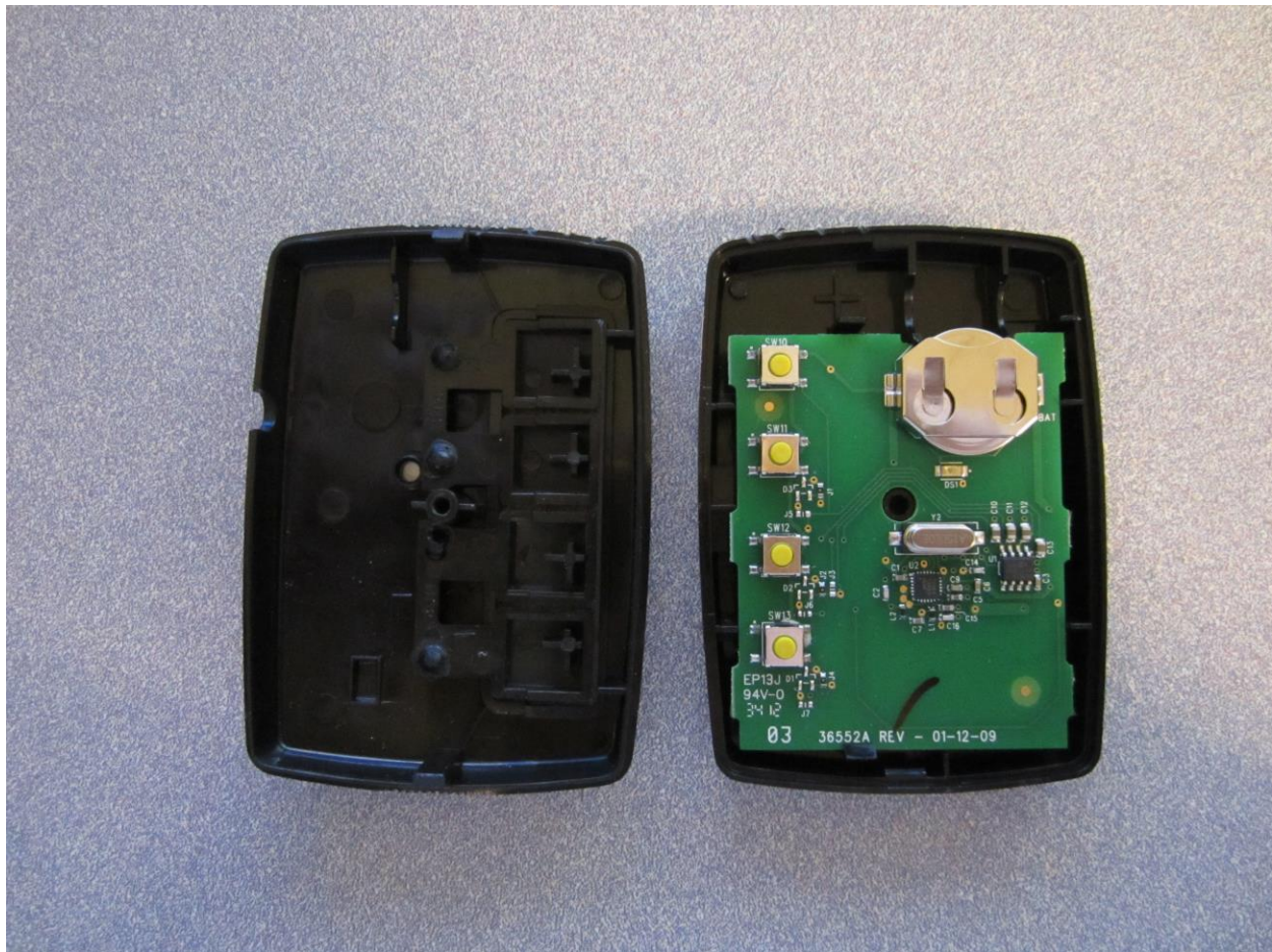
Figure 1: GIDFX4 Internal View / PCB Top
