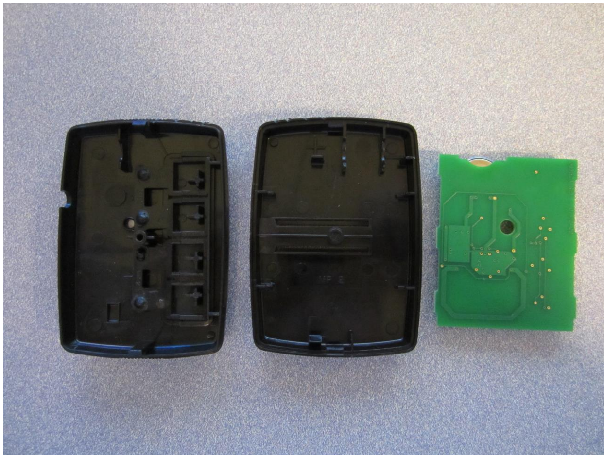
Figure 2: GIDFX4 Internal View / PCB Bottom
