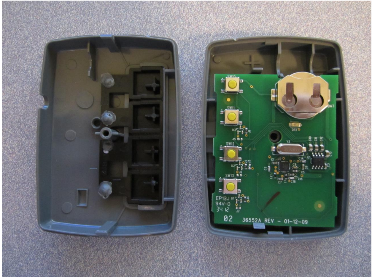
Figure 3: OCDFX4 Internal View / PCB Top
