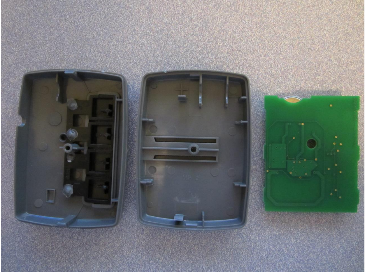
Figure 4: OCDFX4 Internal View / PCB Bottom
