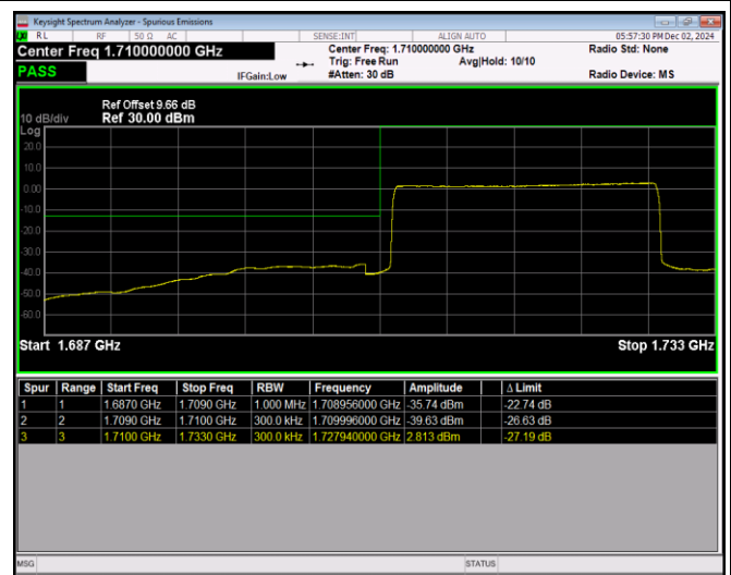
Band66-20MHz-64QAM-132572-1RB#99
