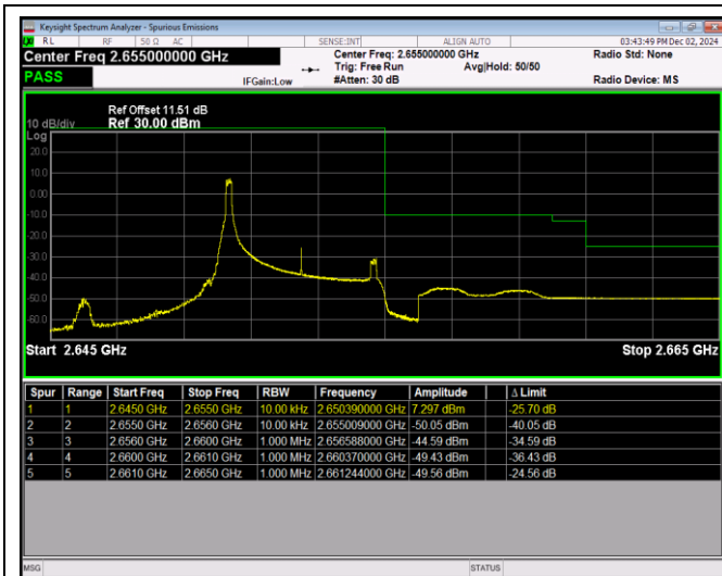
Band41-5MHz-16QAM-41215-25RB#0
