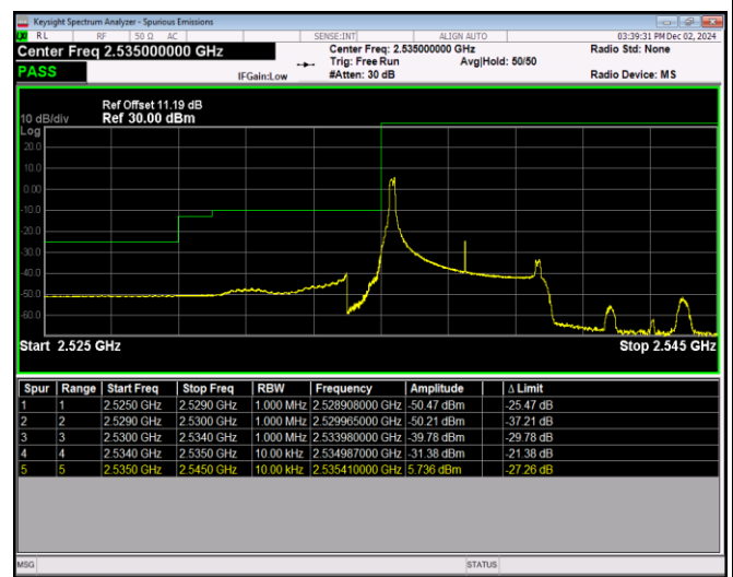
Band41-5MHz-64QAM-40065-25RB#0
