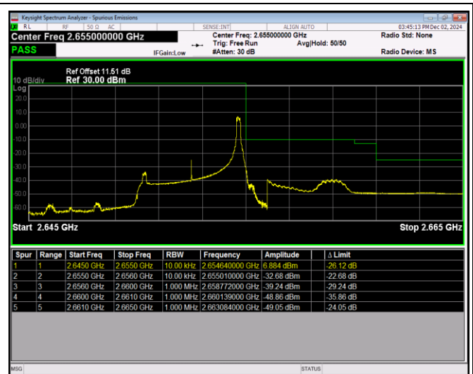
Band41-5MHz-64QAM-40065-1RB#0
