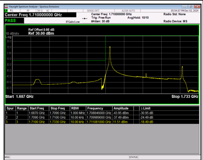
Band66-20MHz-QPSK-132072-100RB#0
