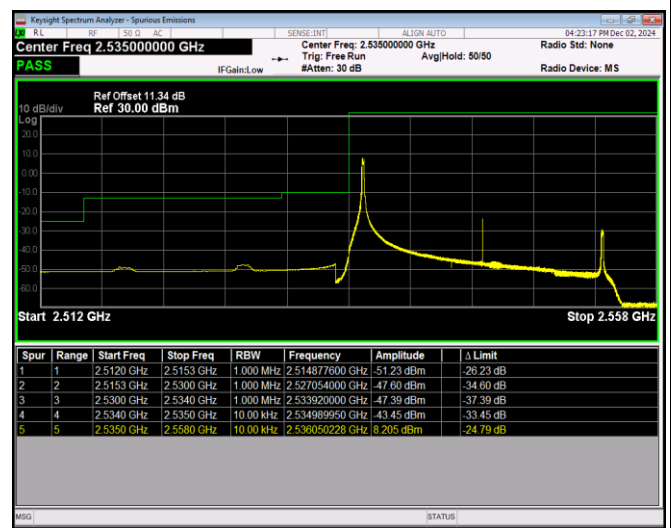
Band41-20MHz-64QAM-40140-100RB#0
