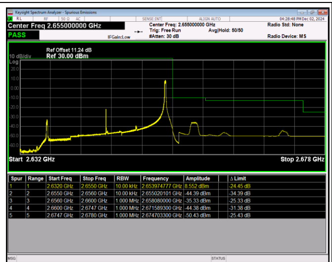
Band41-20MHz-16QAM-40140-1RB#0
