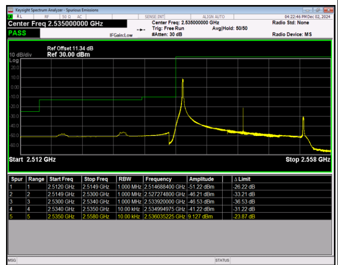
Band41-20MHz-16QAM-40140-100RB#0
