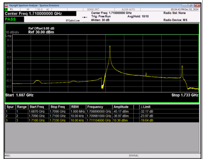
Band66-20MHz-64QAM-132072-100RB#0
