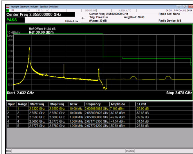
Band41-20MHz-64QAM-41140-100RB#0
