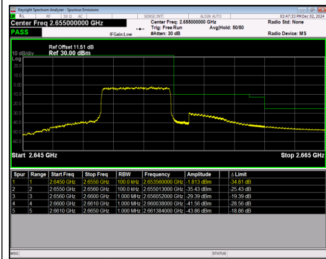
Band41-20MHz-QPSK-40140-1RB#99
