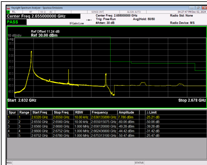
Band41-20MHz-16QAM-41140-100RB#0
