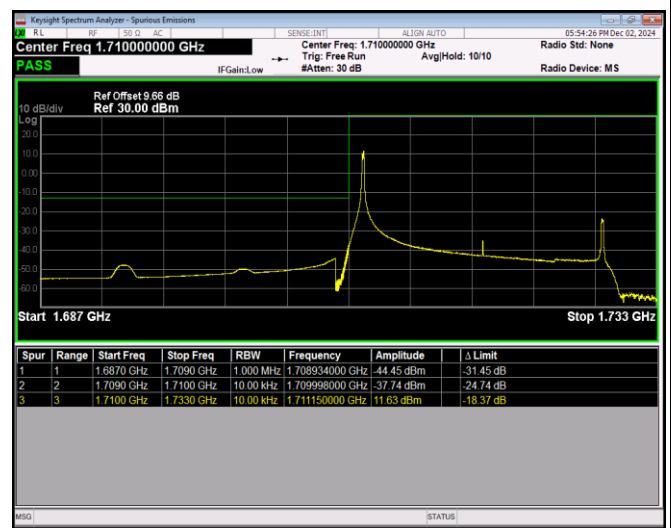
Band66-20MHz-16QAM-132072-100RB#0
