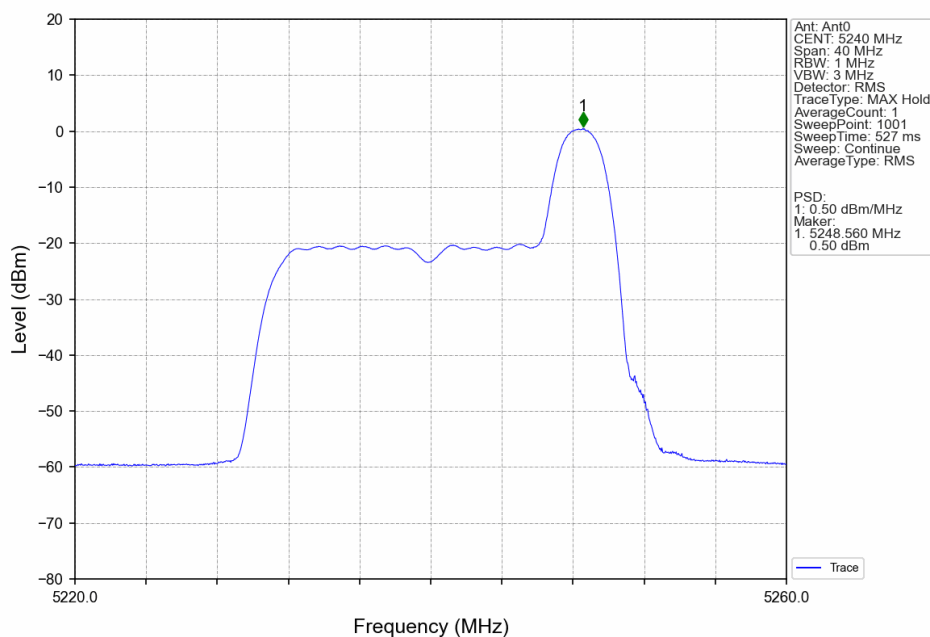
802.11ax(HEW20)_HCH_5240MHz_RU26_Right_Ant0_NTNV
