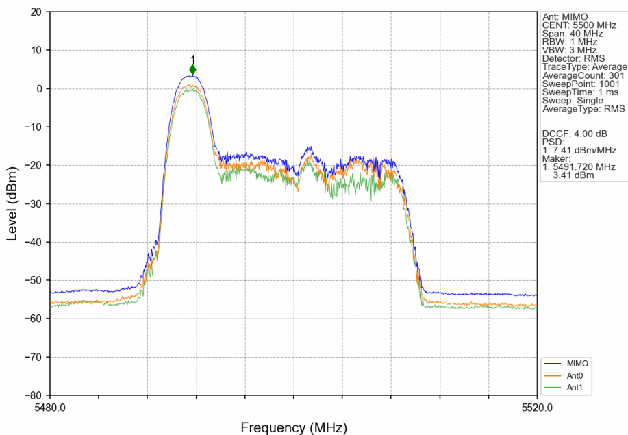
802.11ax(HEW20)_LCH_5500MHz_RU26_Left_MIMO_NTNV
