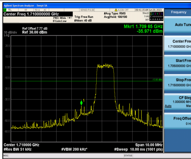
Band4-10MHz-QPSK-20000-6-0-Low--35.97-PASS
