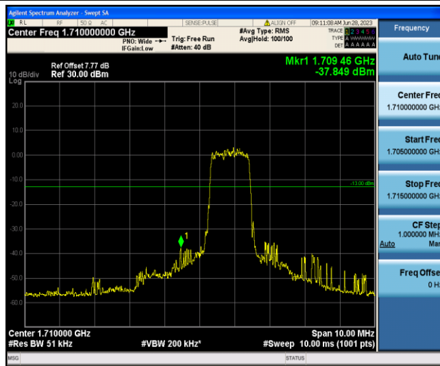
Band4-3MHz-16QAM-19965-6-0-Low--37.85-PASS
