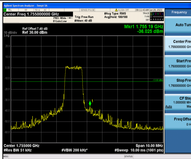
Band4-3MHz-QPSK-20385-6-0-High--36.02-PASS
