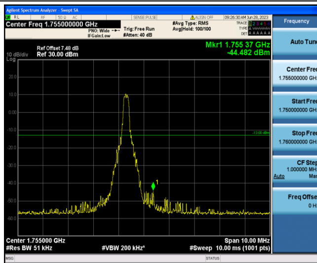
Band4-5MHz-16QAM-20375-1-5-High--44.48-PASS
