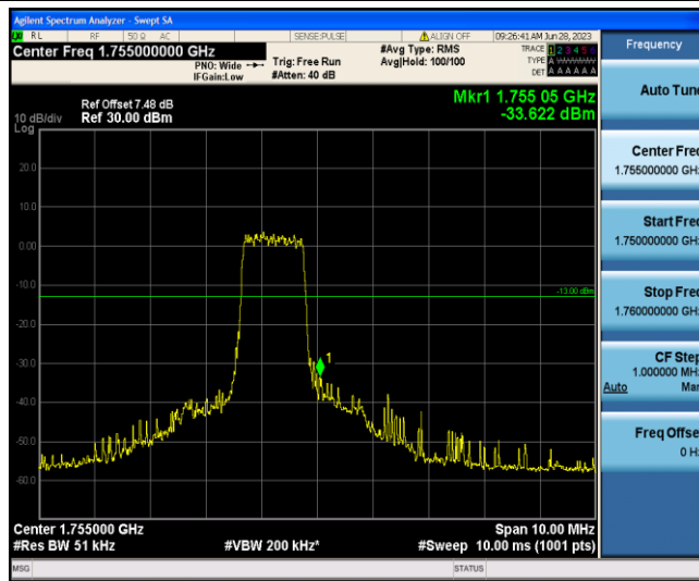
Band4-5MHz-QPSK-20375-6-0-High--33.62-PASS
