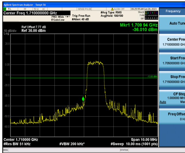
Band4-5MHz-QPSK-19975-6-0-Low--36.01-PASS
