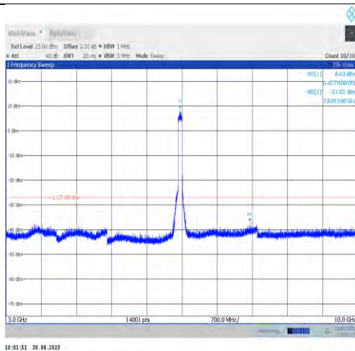
11ax80MIMO-Ant9-6465-3000~10000
