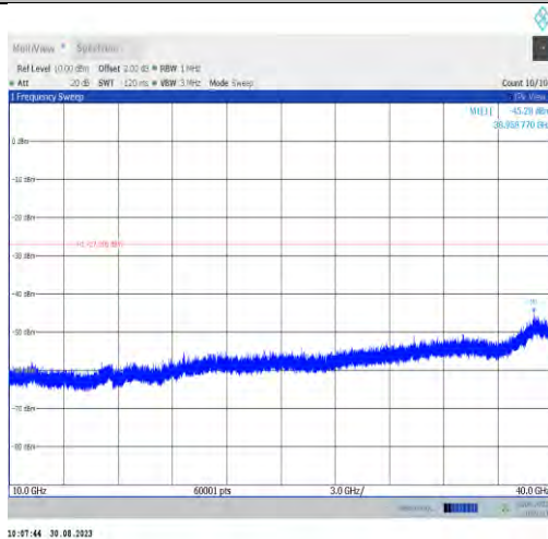
11ax80MIMO-Ant7-6545-10000~40000
