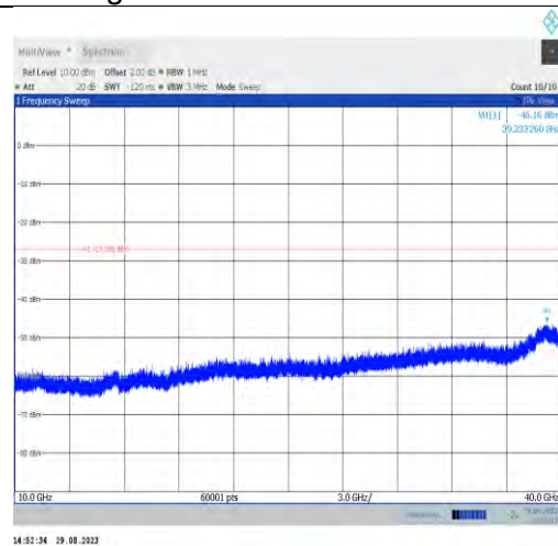
11ax40MIMO-Ant9-6965-10000~40000
