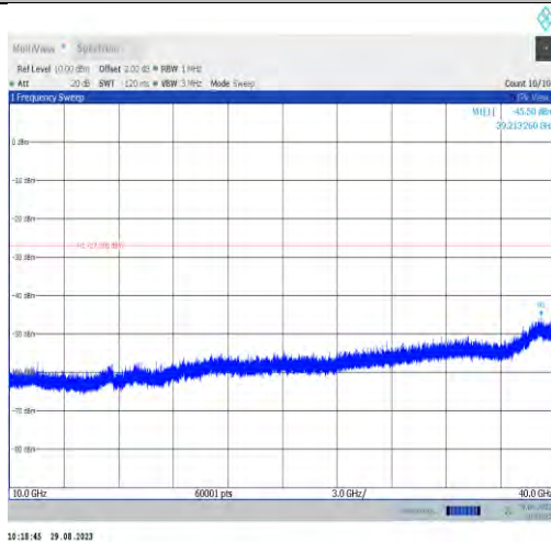
11ax40MIMO-Ant7-6525-10000~40000
