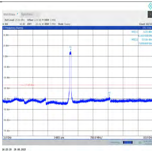
11ax80MIMO-Ant9-6145-3000~10000
