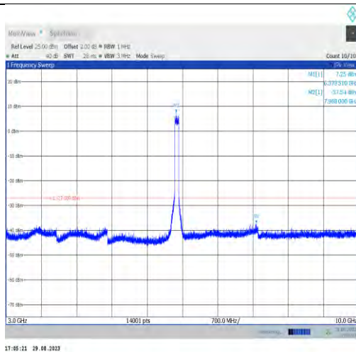
11ax80MIMO-Ant9-6385-3000~10000
