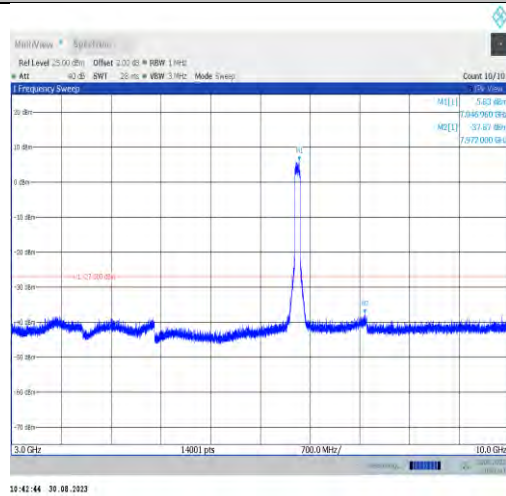
11ax80MIMO-Ant7-7025-3000~10000
