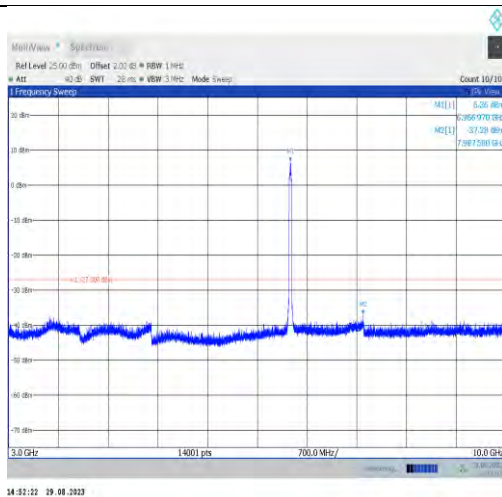
11ax40MIMO-Ant9-6965-3000~10000
