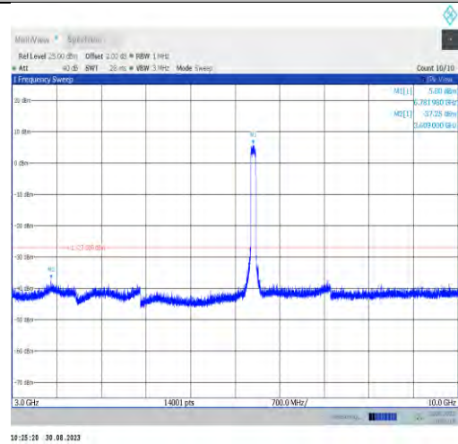
11ax80MIMO-Ant7-6785-3000~10000
