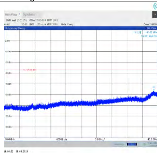
11ax40MIMO-Ant9-6685-10000~40000
