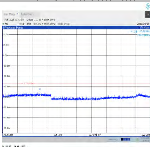
11ax40MIMO-Ant7-6565-30~3000
