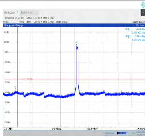
11ax80MIMO-Ant7-6625-3000~10000
