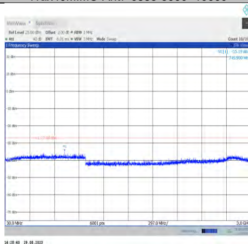
11ax40MIMO-Ant9-6885-30~3000
