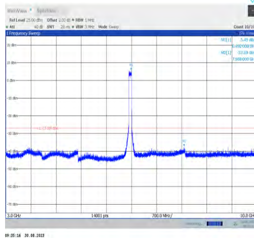
11ax80MIMO-Ant7-6465-3000~10000
