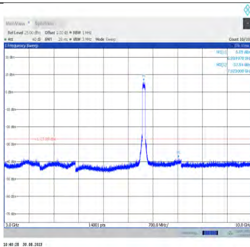
11ax80MIMO-Ant9-6945-3000~10000
