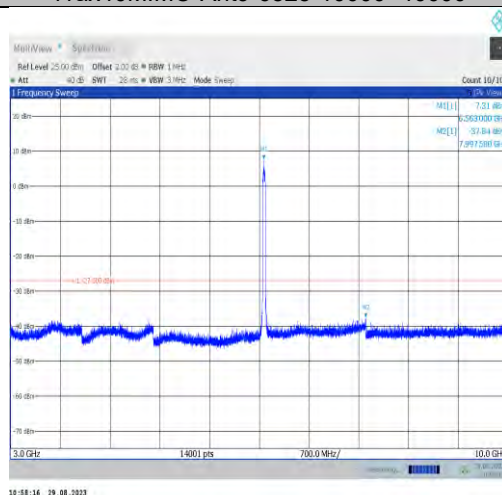
11ax40MIMO-Ant7-6565-3000~10000
