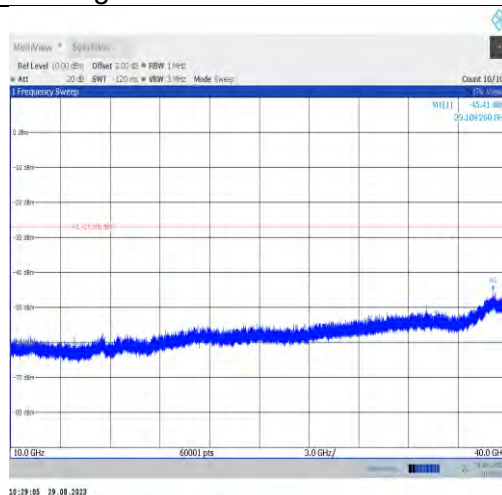
11ax40MIMO-Ant9-6525-10000~40000
