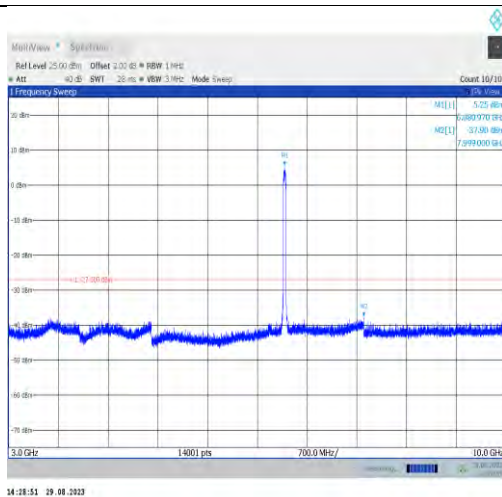
11ax40MIMO-Ant9-6885-3000~10000
