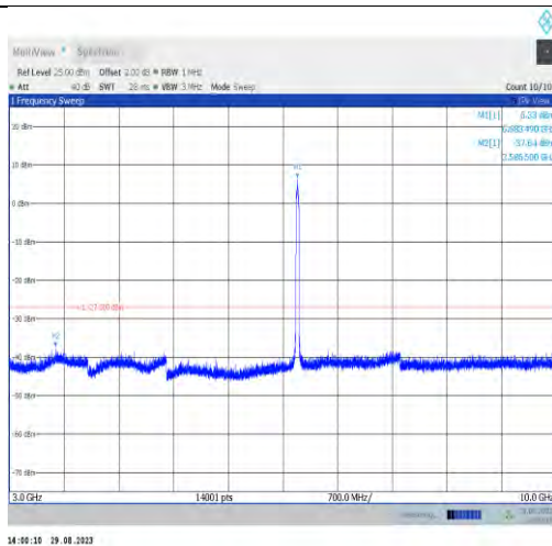
11ax40MIMO-Ant9-6685-3000~10000
