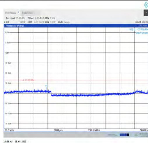
11ax40MIMO-Ant9-6925-30~3000
