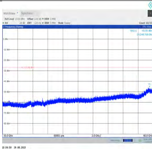
11ax80MIMO-Ant7-5985-10000~40000
