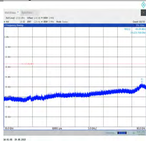
11ax80MIMO-Ant9-5985-10000~40000
