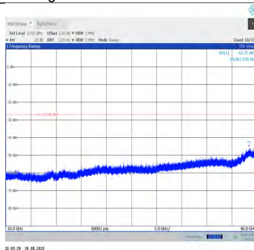
11ax40MIMO-Ant9-7085-10000~40000
