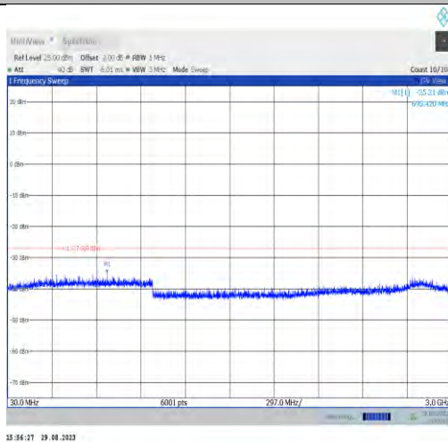
11ax80MIMO-Ant7-5985-30~3000
