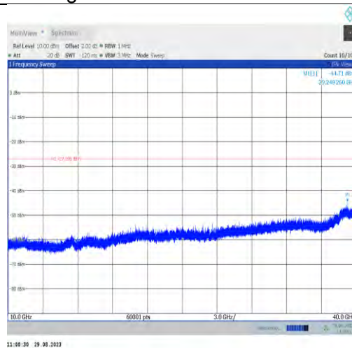
11ax40MIMO-Ant9-6565-10000~40000
