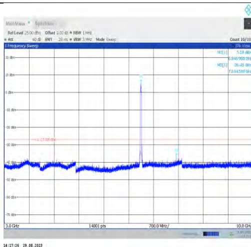
11ax40MIMO-Ant9-6845-3000~10000
