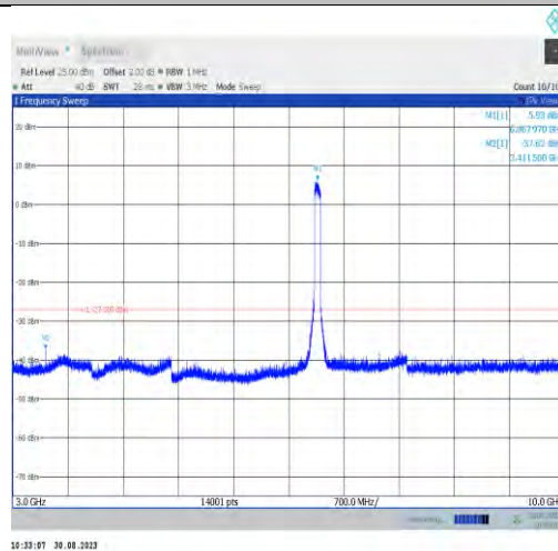
11ax80MIMO-Ant7-6865-3000~10000
