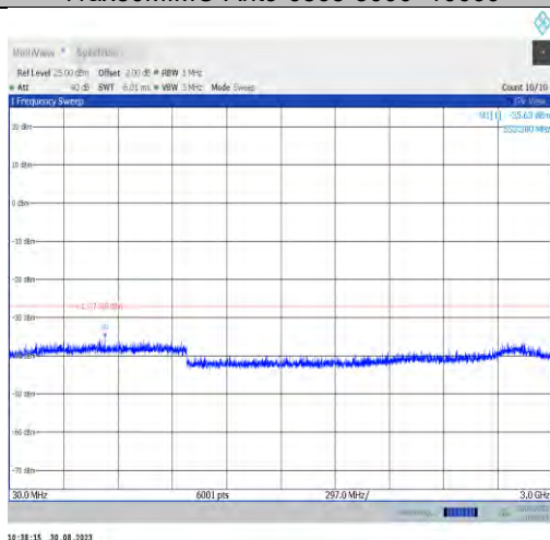
11ax80MIMO-Ant7-6945-30~3000
