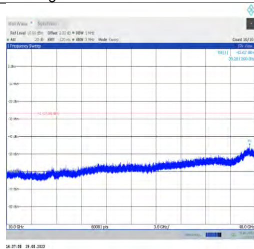
11ax40MIMO-Ant9-6925-10000~40000
