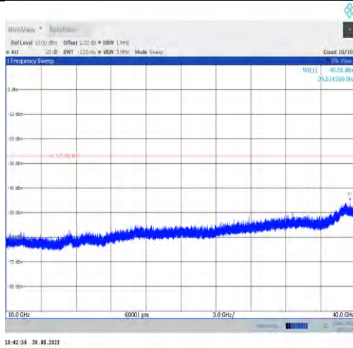
11ax80MIMO-Ant7-7025-10000~40000
