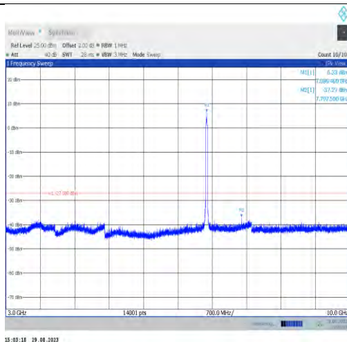
11ax40MIMO-Ant9-7085-3000~10000
