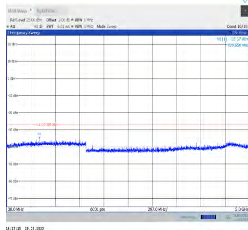
11ax40MIMO-Ant9-6845-30~3000
