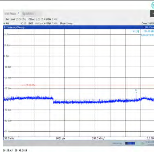
11ax40MIMO-Ant9-6525-30~3000
