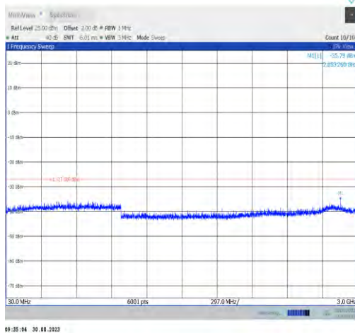
11ax80MIMO-Ant7-6465-30~3000
