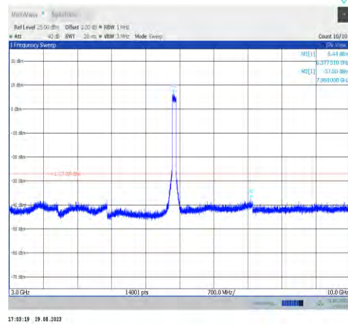
11ax80MIMO-Ant7-6385-3000~10000
