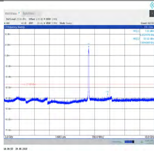
11ax40MIMO-Ant7-6925-3000~10000
