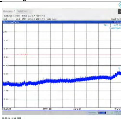
11ax80MIMO-Ant9-6865-10000~40000
