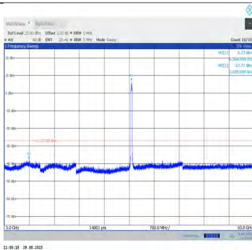
11ax40MIMO-Ant9-6565-3000~10000
