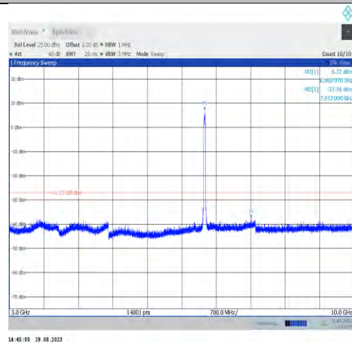
11ax40MIMO-Ant7-6965-3000~10000
