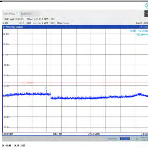
11ax40MIMO-Ant7-6965-30~3000
