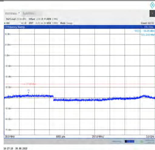
11ax80MIMO-Ant9-6785-30~3000
