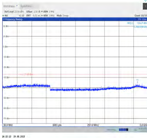
11ax40MIMO-Ant7-6845-30~3000
