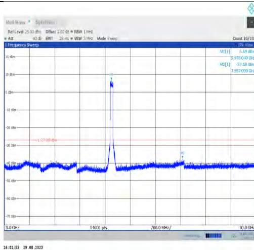
11ax80MIMO-Ant9-5985-3000~10000
