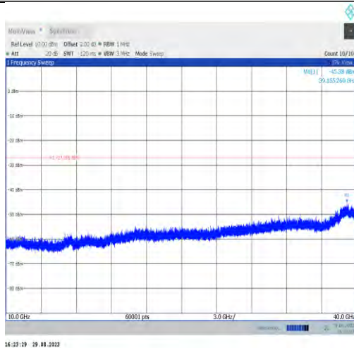
11ax80MIMO-Ant7-6145-10000~40000
