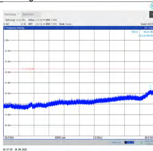
11ax80MIMO-Ant9-6785-10000~40000
