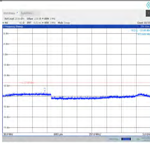
11ax80MIMO-Ant7-6625-30~3000
