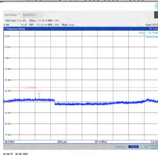
11ax80MIMO-Ant9-6865-30~3000
