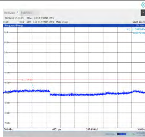
11ax80MIMO-Ant9-6625-30~3000
