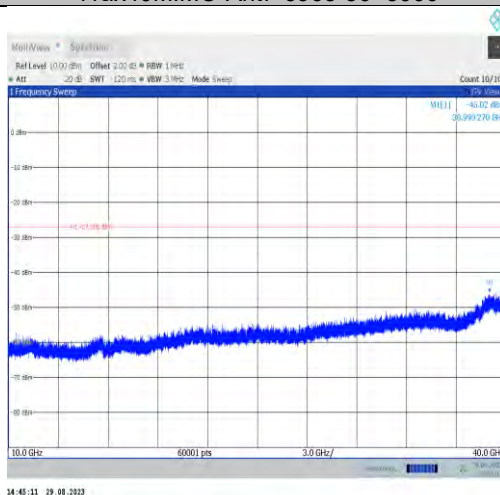
11ax40MIMO-Ant7-6965-10000~40000
