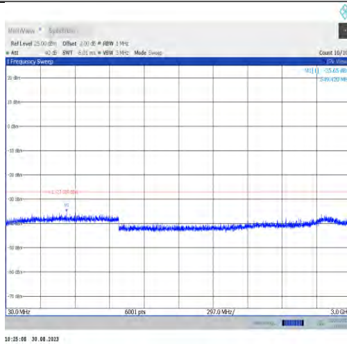
11ax80MIMO-Ant7-6785-30~3000
