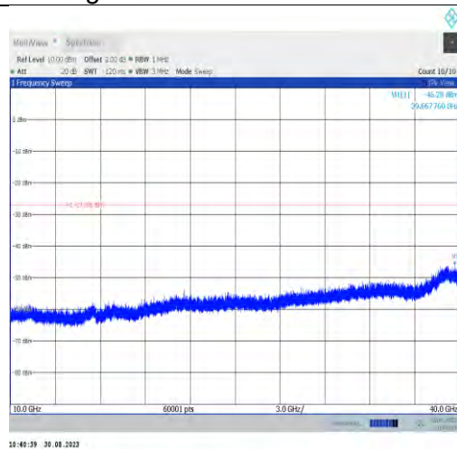
11ax80MIMO-Ant9-6945-10000~40000
