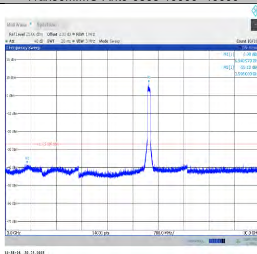
11ax80MIMO-Ant7-6945-3000~10000
