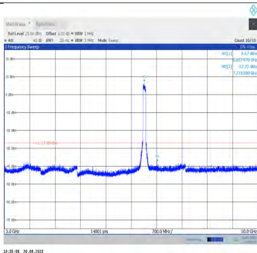
11ax80MIMO-Ant9-6865-3000~10000
