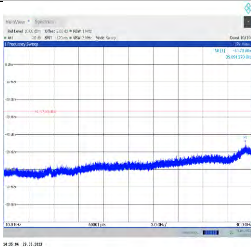
11ax40MIMO-Ant7-6925-10000~40000
