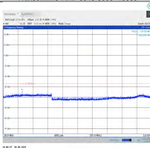
11ax80MIMO-Ant9-6945-30~3000
