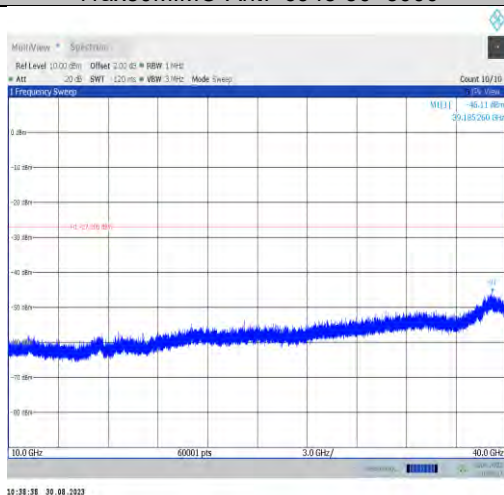
11ax80MIMO-Ant7-6945-10000~40000
