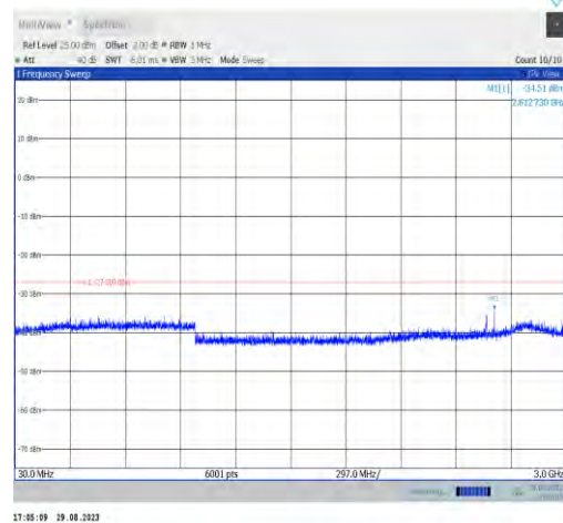
11ax80MIMO-Ant9-6385-30~3000
