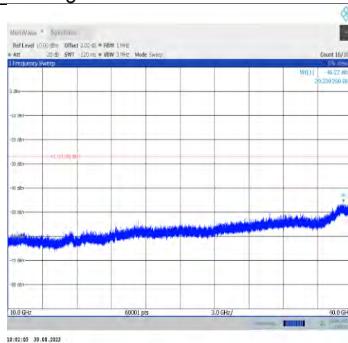
11ax80MIMO-Ant9-6465-10000~40000
