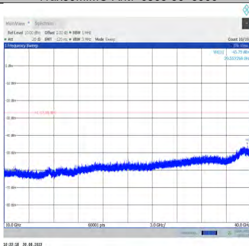
11ax80MIMO-Ant7-6865-10000~40000
