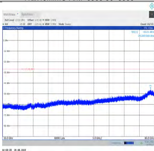
11ax40MIMO-Ant7-6565-10000~40000
