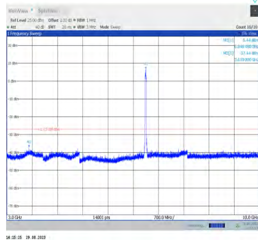
11ax40MIMO-Ant7-6845-3000~10000
