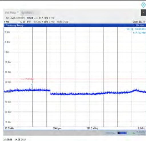
11ax80MIMO-Ant9-6145-30~3000
