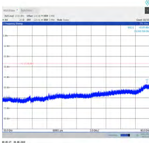
11ax80MIMO-Ant7-6465-10000~40000
