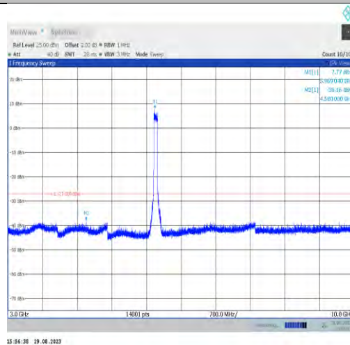
11ax80MIMO-Ant7-5985-3000~10000
