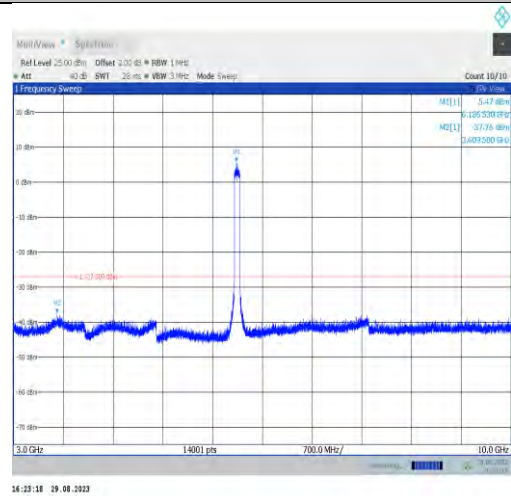
11ax80MIMO-Ant7-6145-3000~10000
