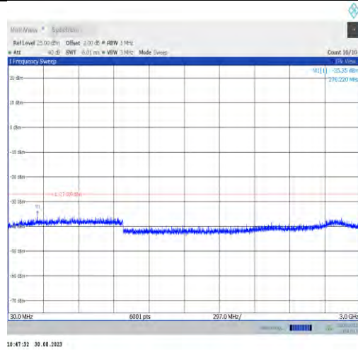
11ax80MIMO-Ant9-7025-30~3000
