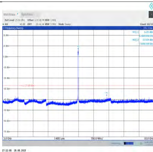
11ax40MIMO-Ant9-6485-3000~10000
