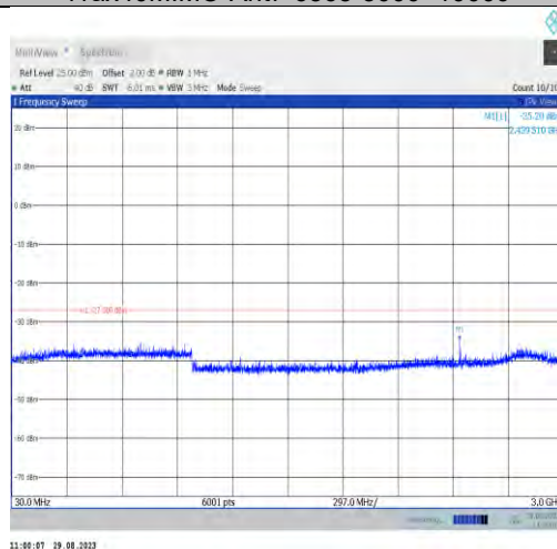
11ax40MIMO-Ant9-6565-30~3000
