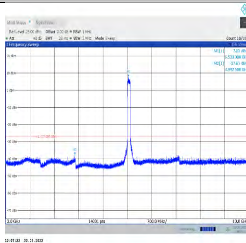
11ax80MIMO-Ant7-6545-3000~10000
