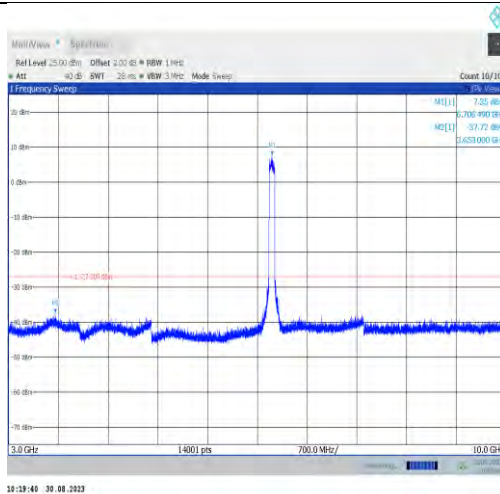
11ax80MIMO-Ant9-6705-3000~10000
