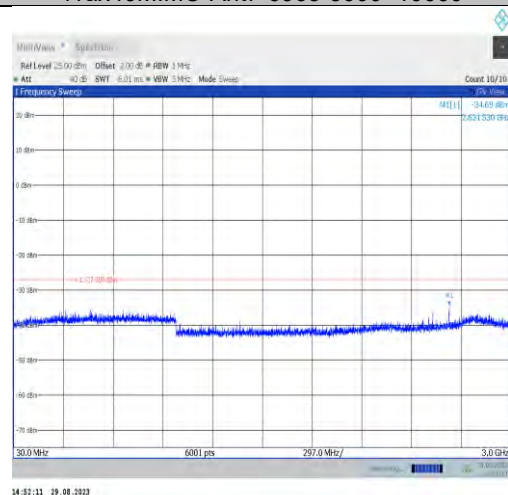
11ax40MIMO-Ant9-6965-30~3000
