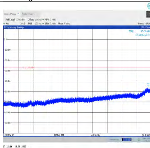
11ax40MIMO-Ant9-6485-10000~40000
