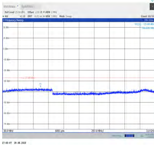
11ax80MIMO-Ant7-6385-30~3000
