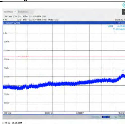
11ax80MIMO-Ant9-6385-10000~40000
