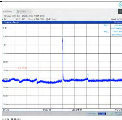
11ax40MIMO-Ant9-6525-3000~10000
