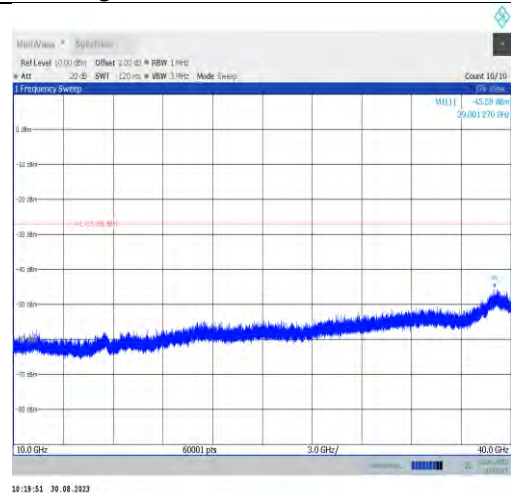
11ax80MIMO-Ant9-6705-10000~40000
