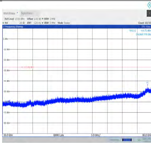
11ax80MIMO-Ant7-6625-10000~40000
