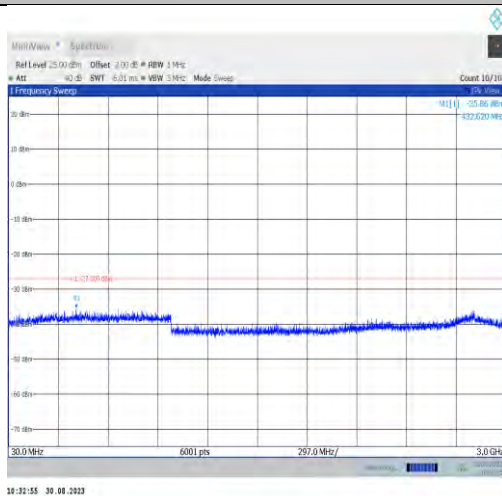
11ax80MIMO-Ant7-6865-30~3000
