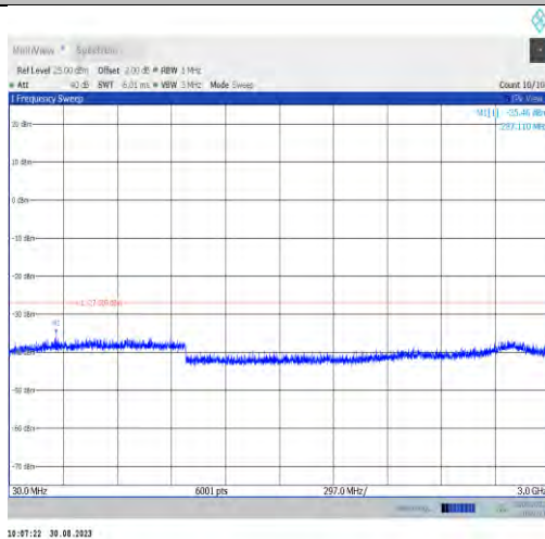
11ax80MIMO-Ant7-6545-30~3000
