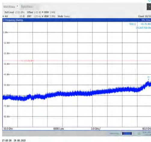
11ax80MIMO-Ant7-6385-10000~40000
