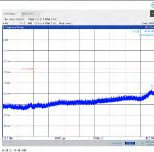
11ax80MIMO-Ant7-6785-10000~40000
