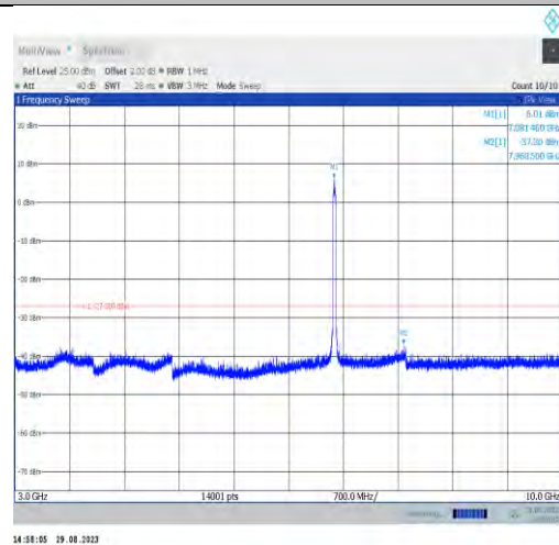
11ax40MIMO-Ant7-7085-3000~10000
