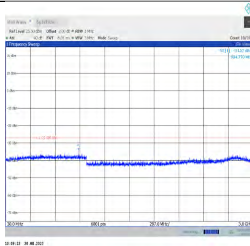
11ax80MIMO-Ant9-6545-30~3000
