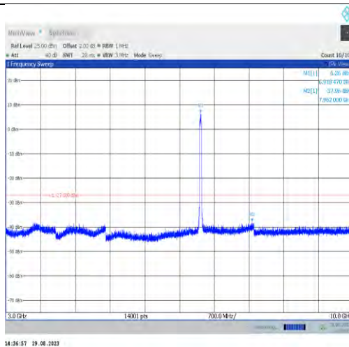
11ax40MIMO-Ant9-6925-3000~10000
