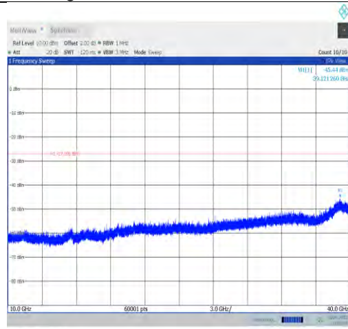
11ax80MIMO-Ant9-6545-10000~40000
