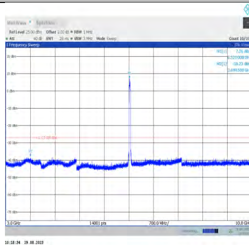
11ax40MIMO-Ant7-6525-3000~10000
