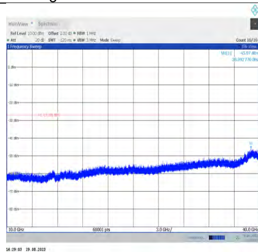
11ax40MIMO-Ant9-6885-10000~40000
