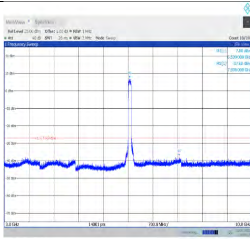
11ax80MIMO-Ant9-6545-3000~10000
