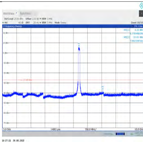
11ax80MIMO-Ant9-6785-3000~10000
