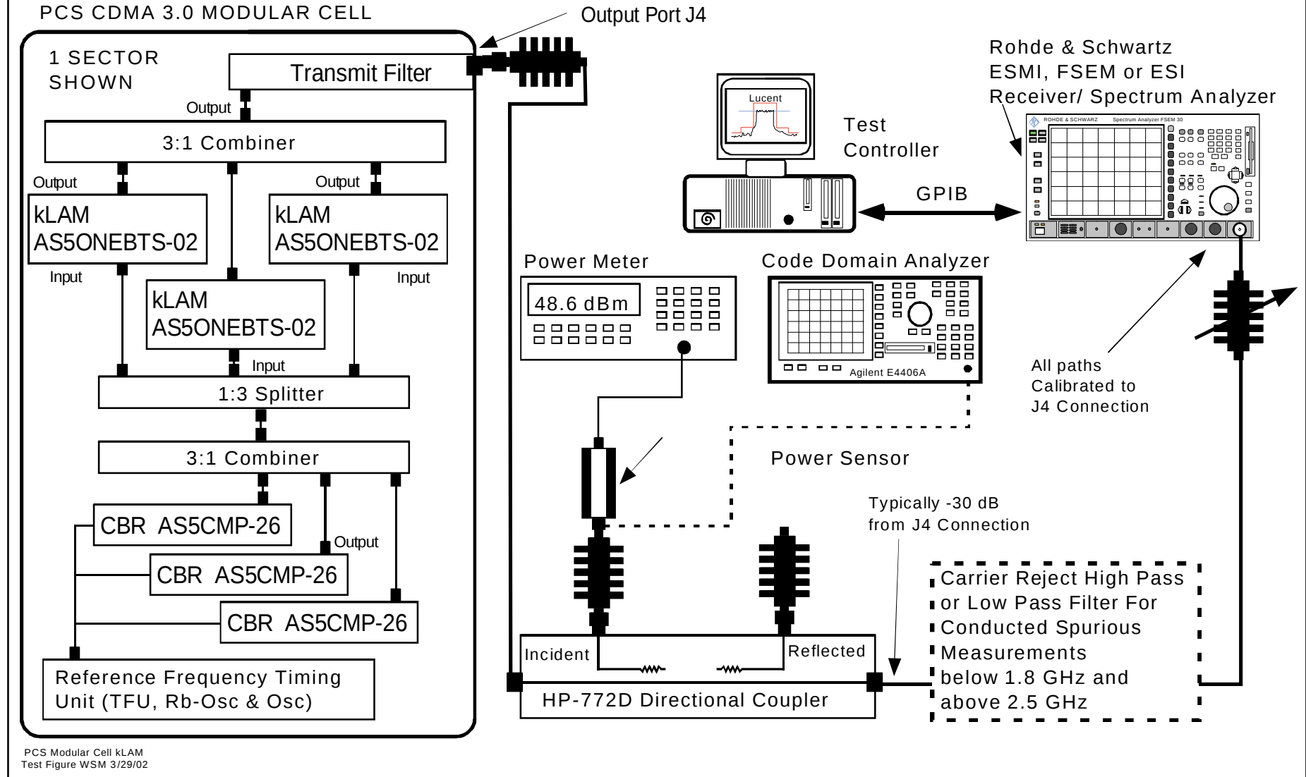
Figure 12A/14A/15A Test Configuration For RF Power, Occupied Bandwidth and Conducted Spurious
