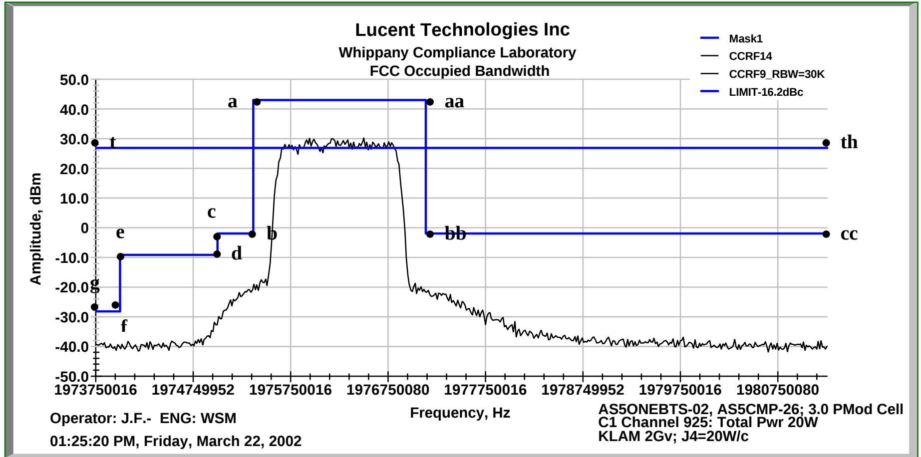
Figure 14B Occupied Bandwidth Mask
