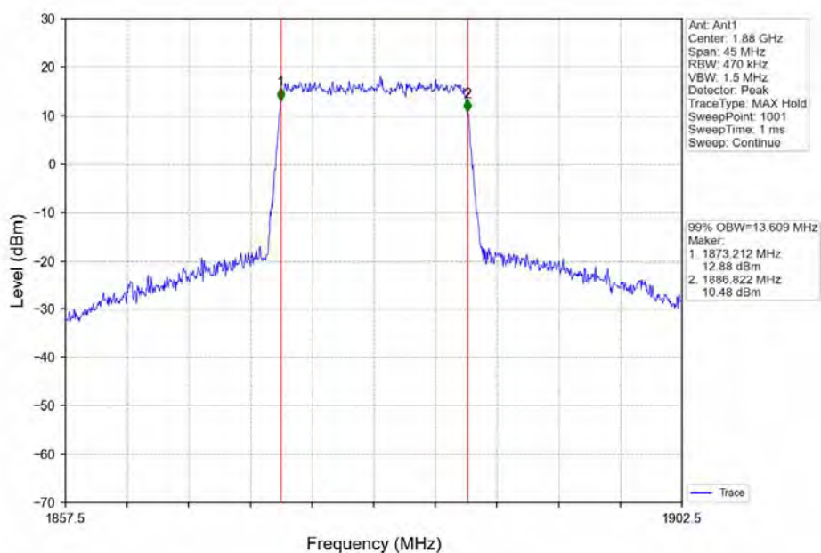
Band2_15MHz_64QAM_MCH_1880MHz_RB_75_0_NTNV
