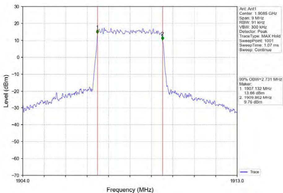
Band2_3MHz_64QAM_HCH_1908.5MHz_RB_15_0_NTNV
