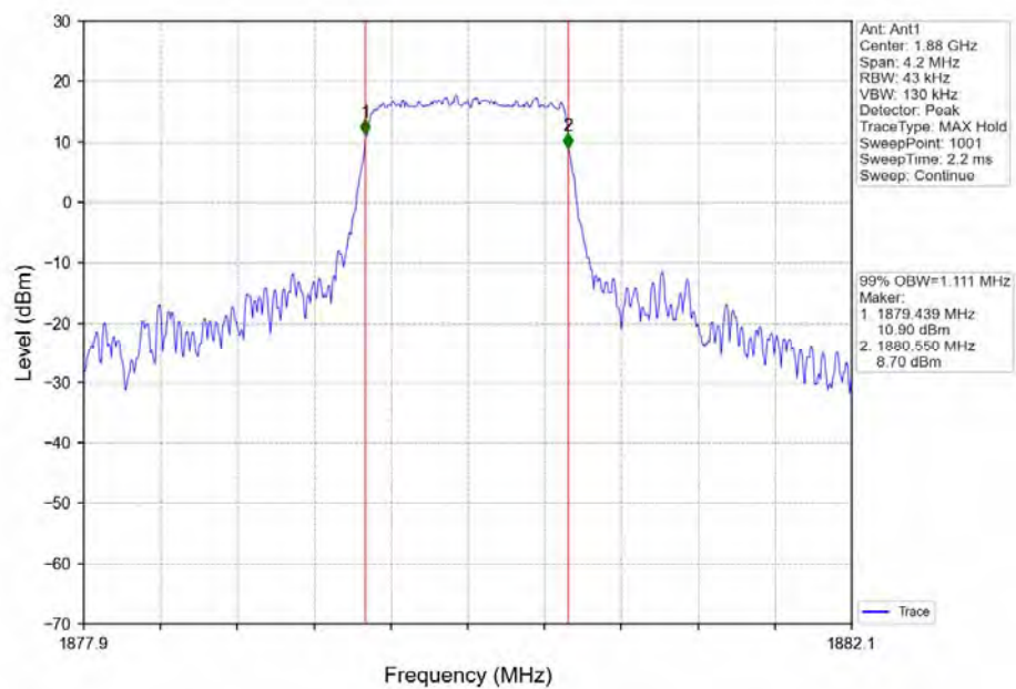
Band2_1.4MHz_64QAM_MCH_1880MHz_RB_6_0_NTNV
