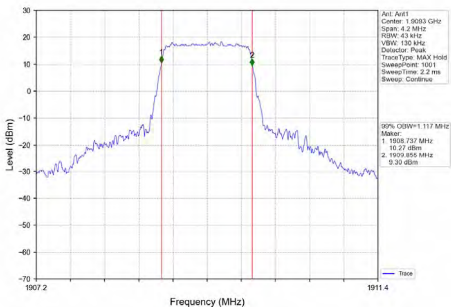
Band2_1.4MHz_16QAM_HCH_1909.3MHz_RB_6_0_NTNV
