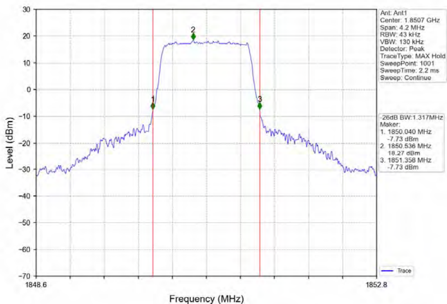
Band2_1.4MHz_16QAM_LCH_1850.7MHz_RB_6_0_NTNV
