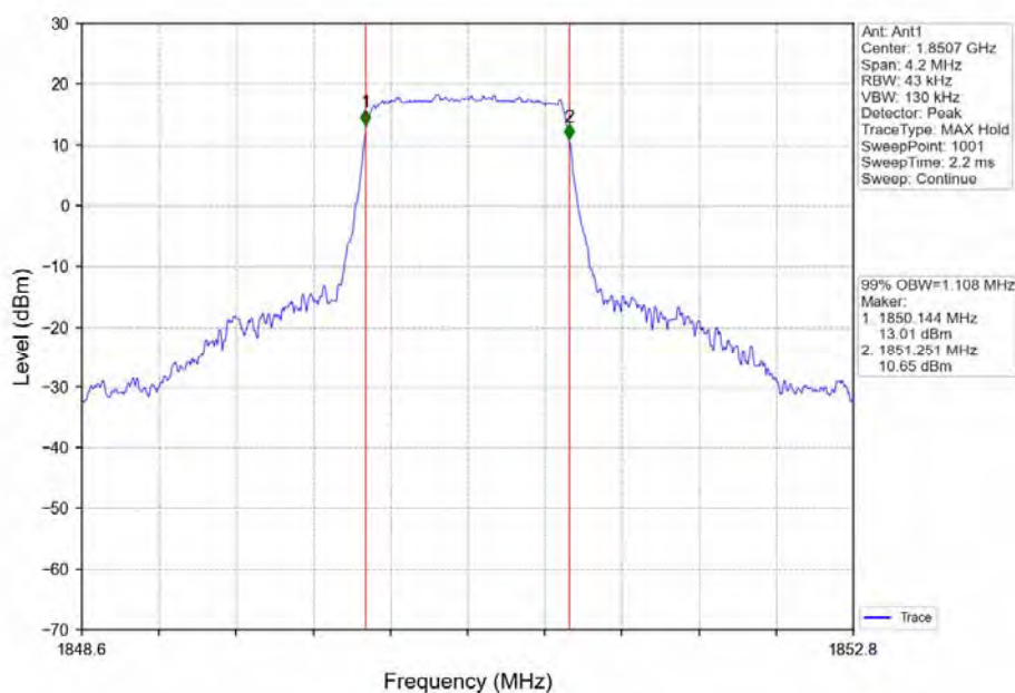
Band2_1.4MHz_16QAM_LCH_1850.7MHz_RB_6_0_NTNV
