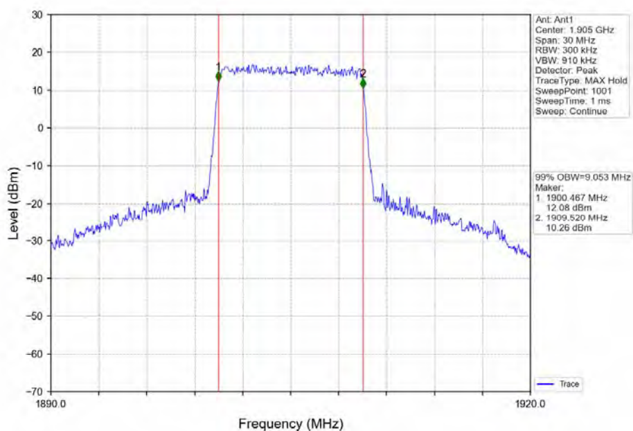
Band2_10MHz_64QAM_HCH_1905MHz_RB_50_0_NTNV
