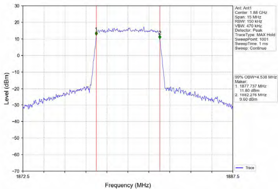
Band2_5MHz_64QAM_MCH_1880MHz_RB_25_0_NTNV
