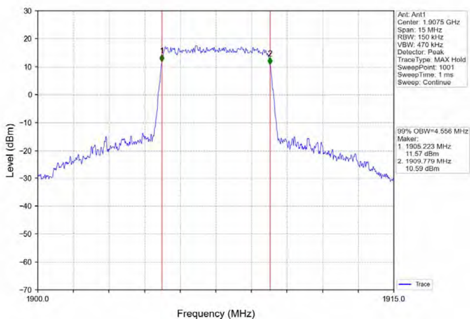
Band2_5MHz_16QAM_HCH_1907.5MHz_RB_25_0_NTNV
