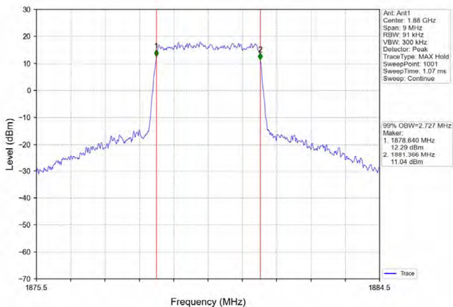
Band2_3MHz_16QAM_MCH_1880MHz_RB_15_0_NTNV
