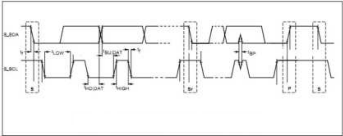
Figure 6: Definition of Timing for F/S-Mode Devices on the I²C-Bus
