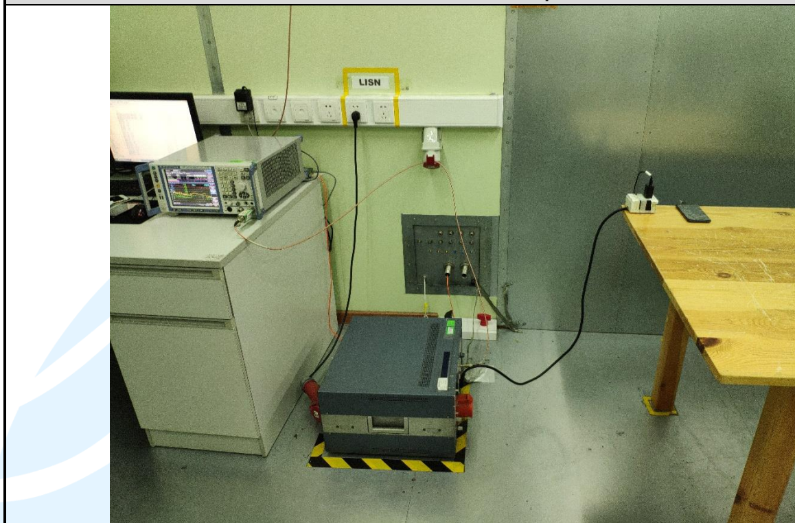
Conducted Emission Test Setup - Mode 5
