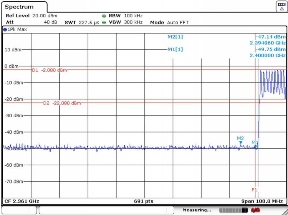
8-DPSK Low Channel Hopping ON
