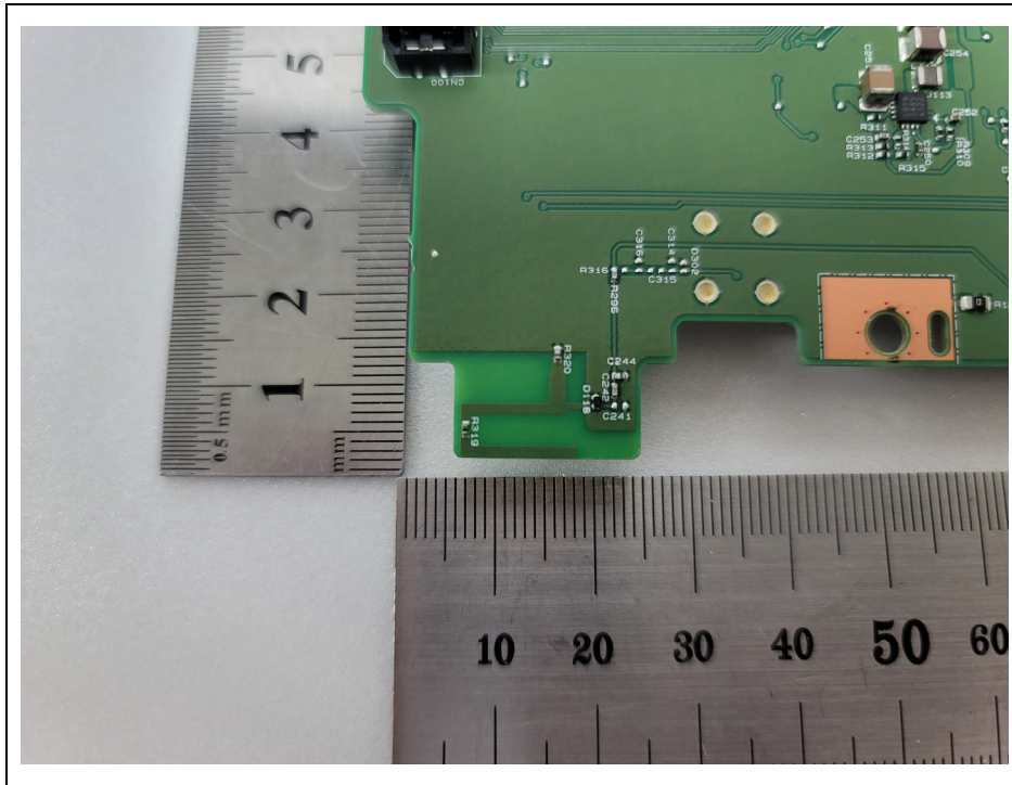
<BT Antenna>
