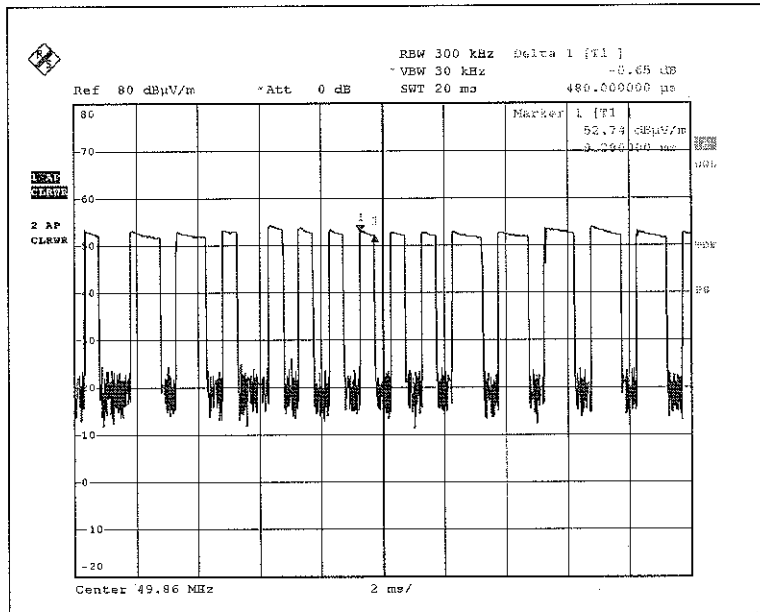
Duty Cycle 3
