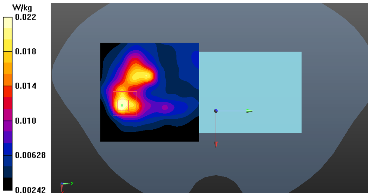
Fig.28 Bluetooth Body
