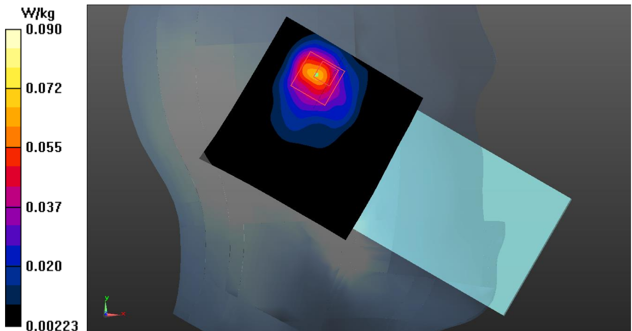
Fig.27 Bluetooth Head
