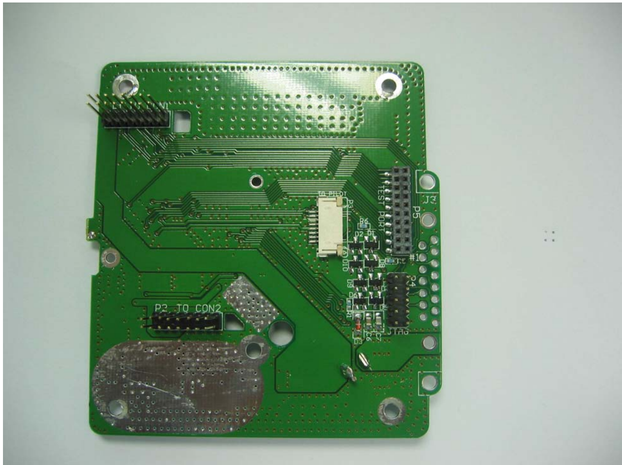
LPA - Rev D1 Mother Board - Part A - Bottom
