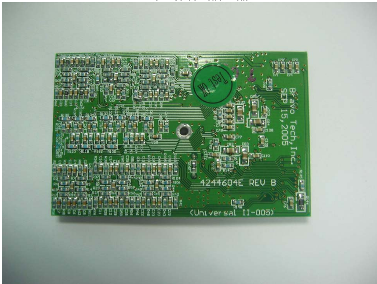
LPA - Rev B Control Board - Bottom
