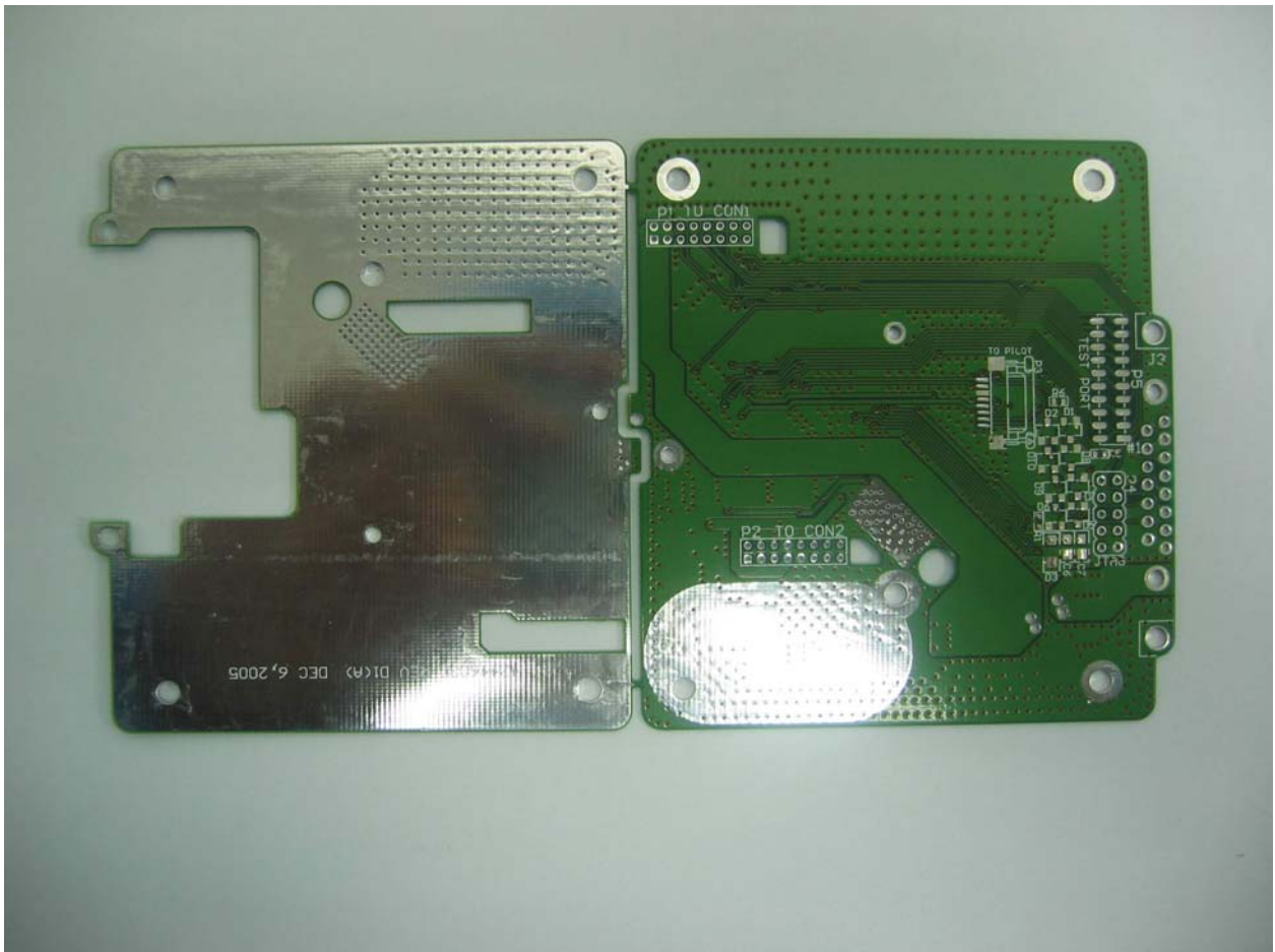
LPA - Rev D1 Mother Board - Bottom
