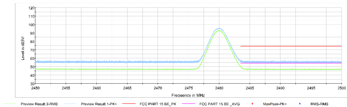
Fig.16. Frequency Band Edges: \pi/4 DQPSK, Channel 78, Hopping Off, 2.45 GHz - 2.50GHz
