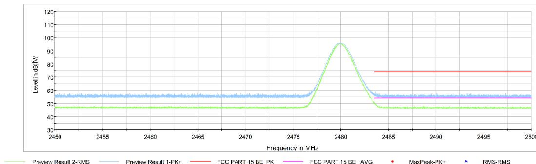
Fig.14. Frequency Band Edges: GFSK, Channel 78, Hopping Off, ch11, 2.45 GHz - 2.50GHz
