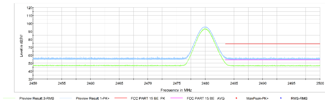
Fig.18. Frequency Band Edges: 8DPSK, Channel 78, 2.45 GHz - 2.50GHz
