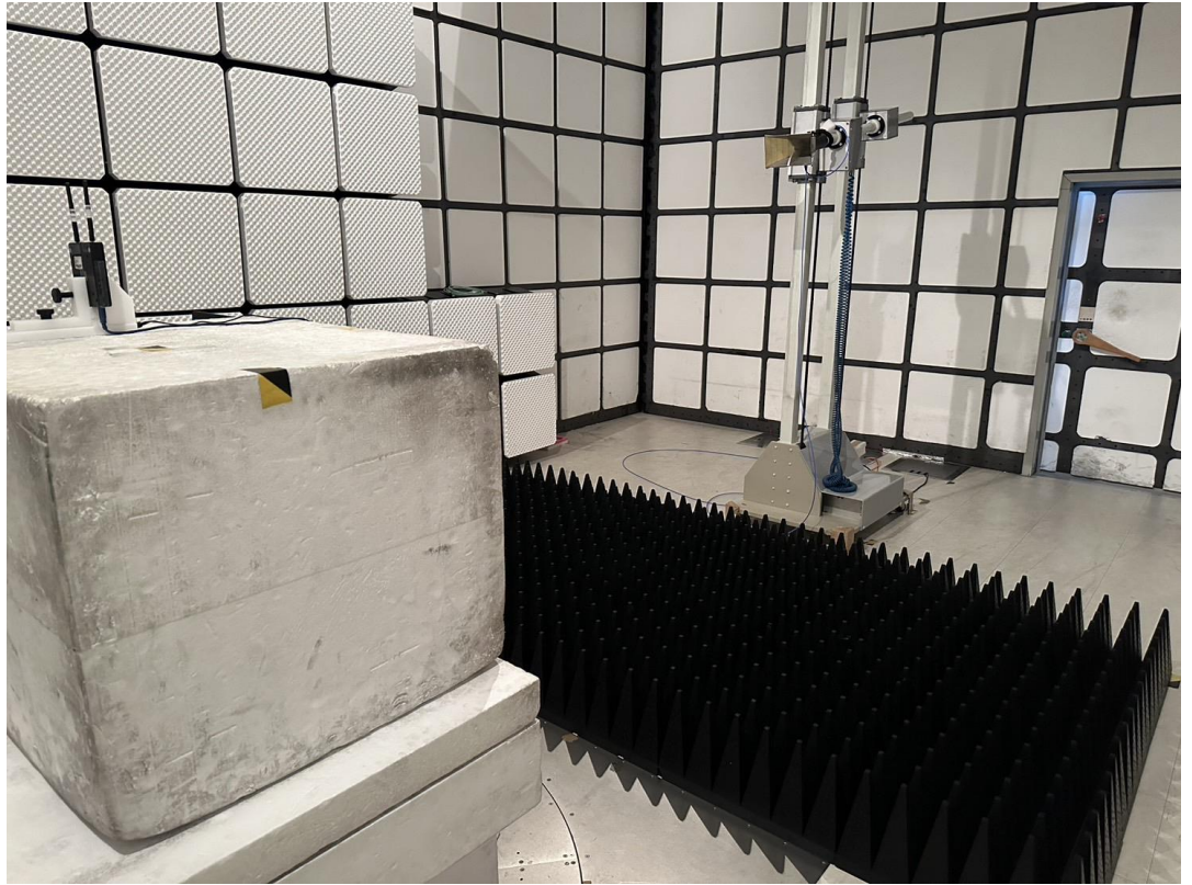
Side View
