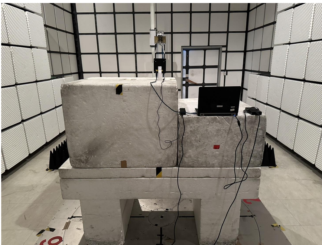
Rear View
