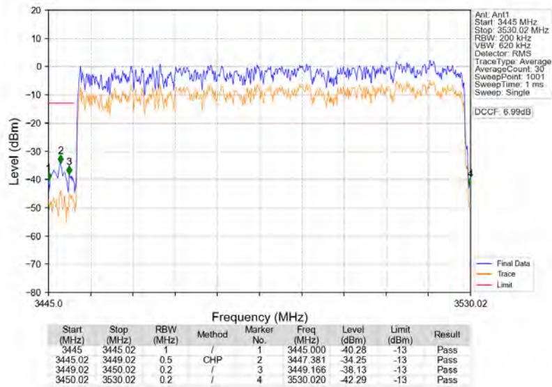
n77d_30kHz_SISO_NTNV_80MHz_DFT-s-OFDM_PI/2_BPSK_3490.02MHz_Outer_Full
