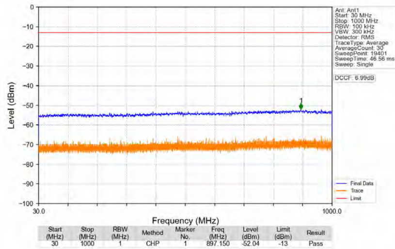
n77d_30kHz_SISO_NTNV_50MHz_DFT-s-OFDM_QPSK_3475.02MHz_Edge_1RB_Left
