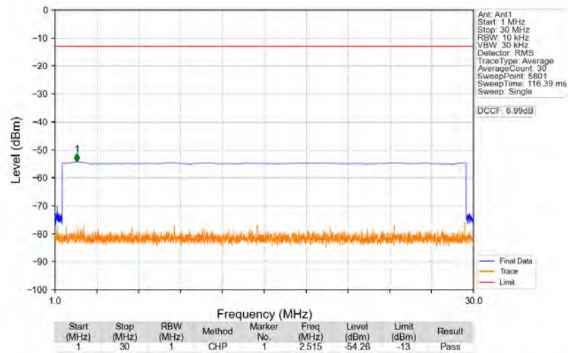
n77d_30kHz_SISO_NTNV_40MHz_CP-OFDM_QPSK_3500.01MHz_Edge_1RB_Left
