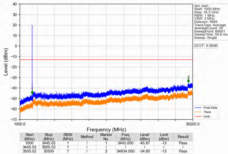
n77d_30kHz_SISO_NTNV_50MHz_CP-OFDM_QPSK_3475.02MHz_Edge_1RB_Left
