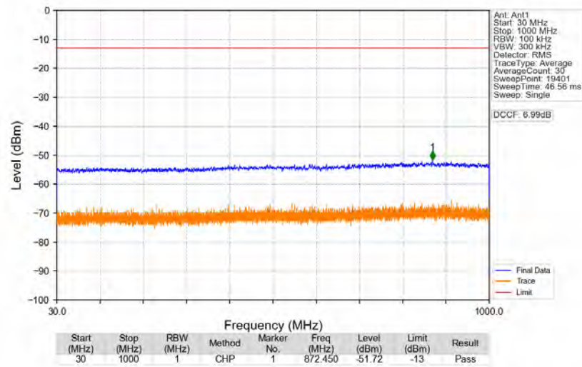
n77d_30kHz_SISO_NTNV_70MHz_DFT-s-OFDM_QPSK_3485.01MHz_Edge_1RB_Left
