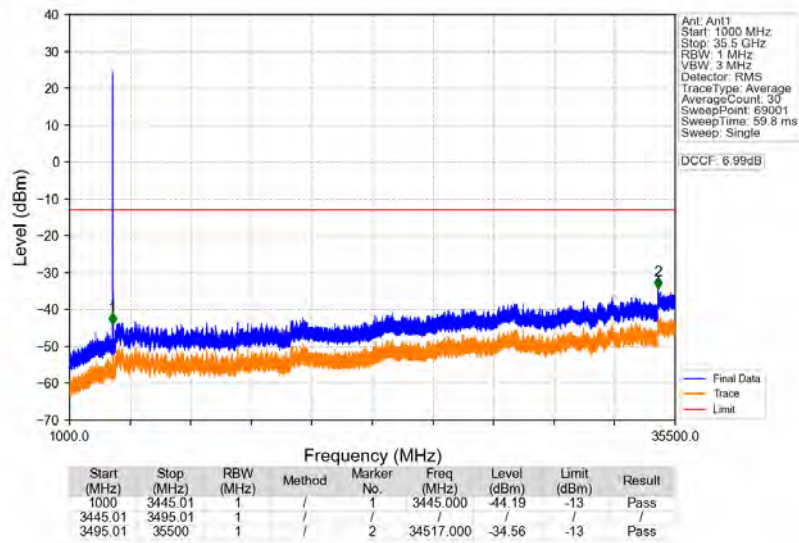
n77d_30kHz_SISO_NTNV_40MHz_DFT-s-OFDM_PI/2_BPSK_3470.01MHz_Edge_1RB_Left
