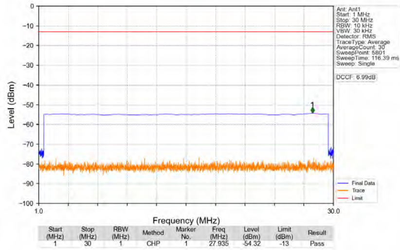
n77d_30kHz_SISO_NTNV_30MHz_CP-OFDM_QPSK_3534.99MHz_Edge_1RB_Right
