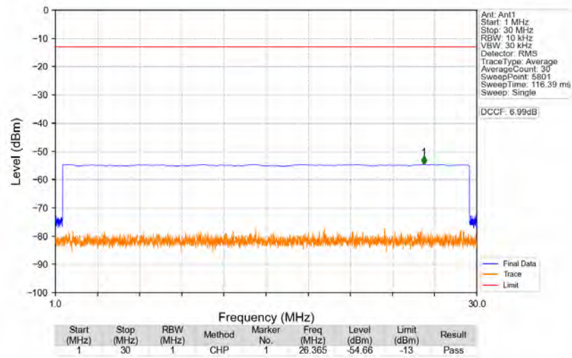
n77d_30kHz_SISO_NTNV_80MHz_DFT-s-OFDM_QPSK_3490.02MHz_Edge_1RB_Left
