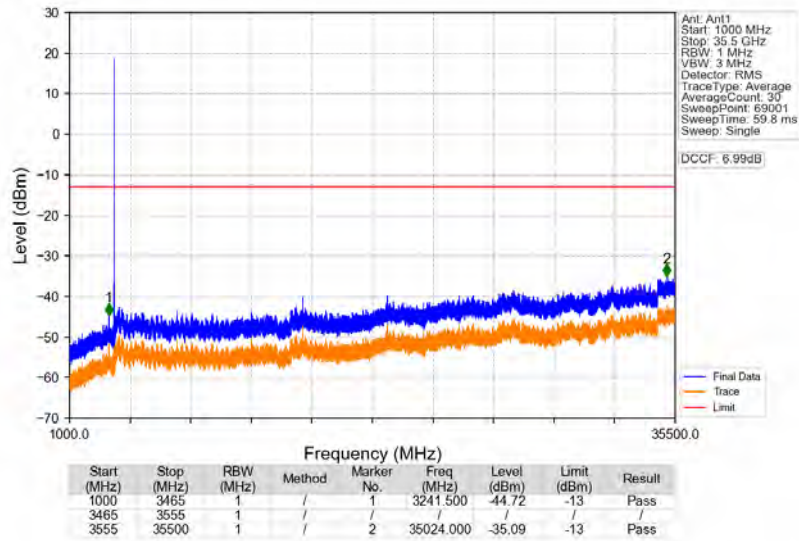
n77d_30kHz_SISO_NTNV_80MHz_DFT-s-OFDM_QPSK_3510MHz_Edge_1RB_Right
