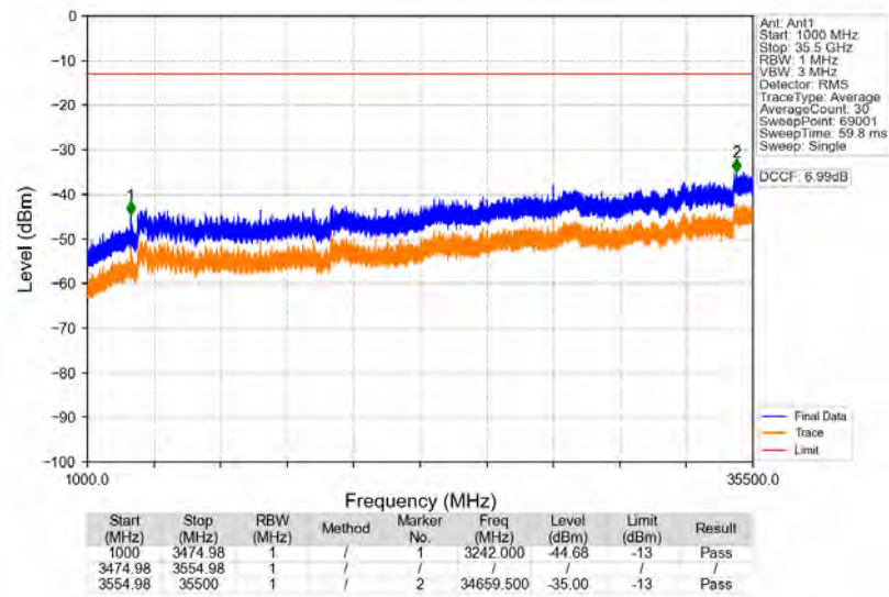
n77d_30kHz_SISO_NTNV_70MHz_DFT-s-OFDM_PI/2_BPSK_3514.98MHz_Edge_1RB_Right
