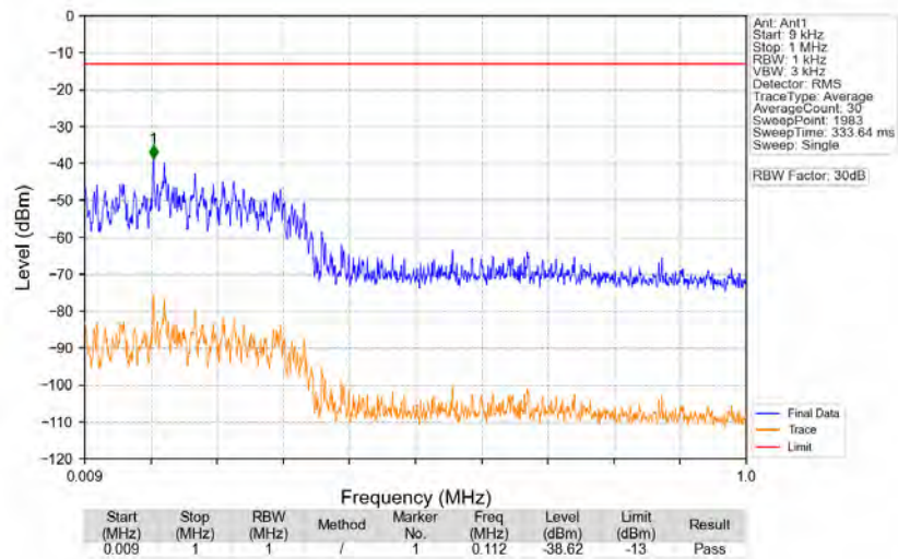
n77d_30kHz_SISO_NTNV_80MHz_DFT-s-OFDM_QPSK_3510MHz_Edge_1RB_Right
