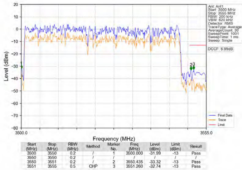
n77d_30kHz_SISO_NTNV_50MHz_DFT-s-OFDM_QPSK_3525MHz_Outer_Full
