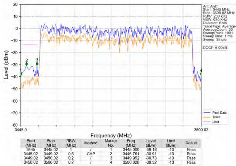
n77d_30kHz_SISO_NTNV_50MHz_DFT-s-OFDM_QPSK_3475.02MHz_Outer_Full
