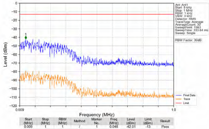
n77d_30kHz_SISO_NTNV_60MHz_CP-OFDM_QPSK_3519.99MHz_Edge_1RB_Right
