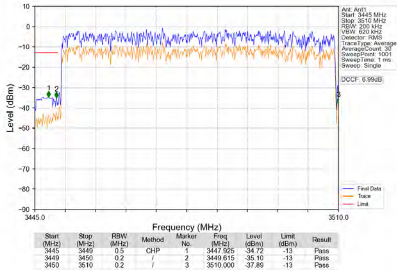
n77d_30kHz_SISO_NTNV_60MHz_CP-OFDM_QPSK_3480MHz_Outer_Full
