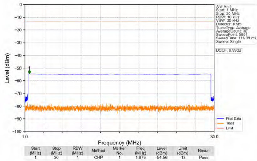
n77d_30kHz_SISO_NTNV_70MHz_DFT-s-OFDM_QPSK_3485.01MHz_Edge_1RB_Left
