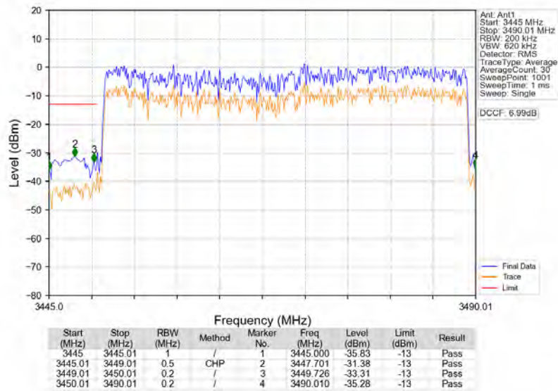
n77d_30kHz_SISO_NTNV_40MHz_CP-OFDM_QPSK_3470.01MHz_Outer_Full
