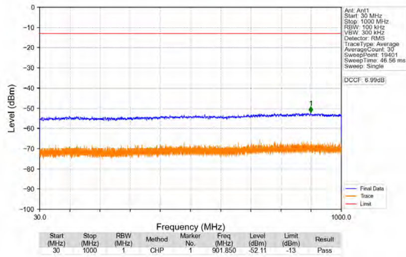
n77d_30kHz_SISO_NTNV_70MHz_CP-OFDM_QPSK_3500.01MHz_Edge_1RB_Left
