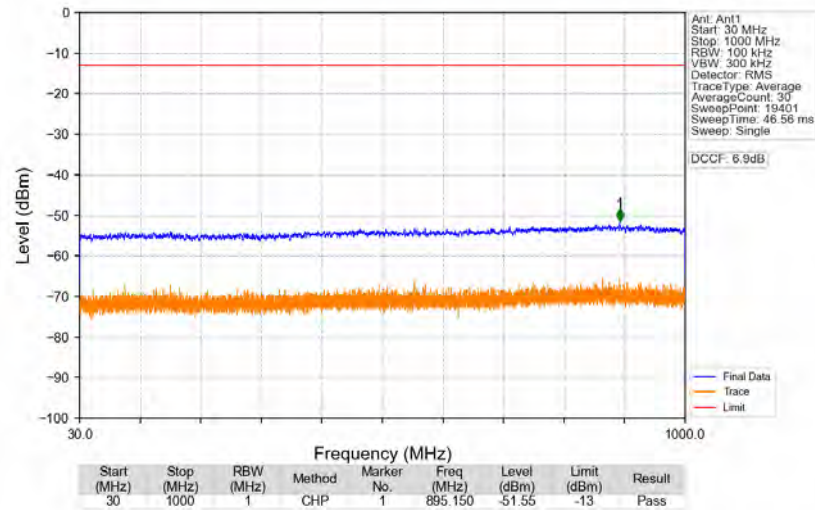
n77d_30kHz_SISO_NTNV_30MHz_CP-OFDM_QPSK_3465MHz_Edge_1RB_Left
