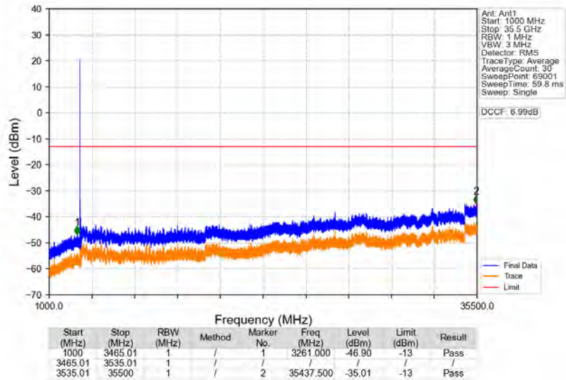
n77d_30kHz_SISO_NTNV_60MHz_CP-OFDM_QPSK_3500.01MHz_Edge_1RB_Left
