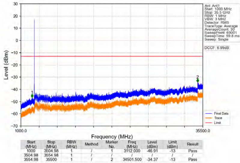
n77d_30kHz_SISO_NTNV_40MHz_CP-OFDM_QPSK_3529.98MHz_Edge_1RB_Right
