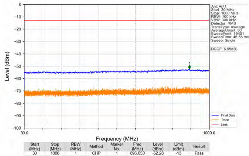
n77d_30kHz_SISO_NTNV_60MHz_CP-OFDM_QPSK_3480MHz_Edge_1RB_Left
