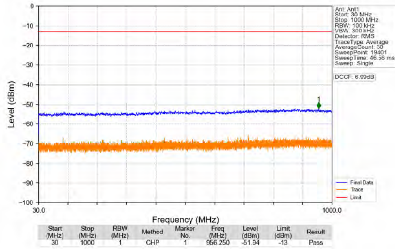
n77d_30kHz_SISO_NTNV_50MHz_DFT-s-OFDM_QPSK_3500.01MHz_Edge_1RB_Left
