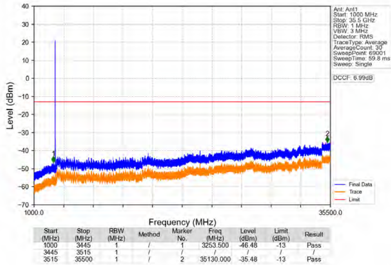
n77d_30kHz_SISO_NTNV_60MHz_DFT-s-OFDM_QPSK_3480MHz_Edge_1RB_Left
