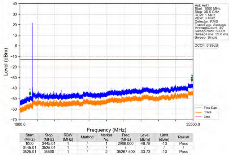
n77d_30kHz_SISO_NTNV_70MHz_DFT-s-OFDM_PI/2_BPSK_3485.01MHz_Edge_1RB_Left
