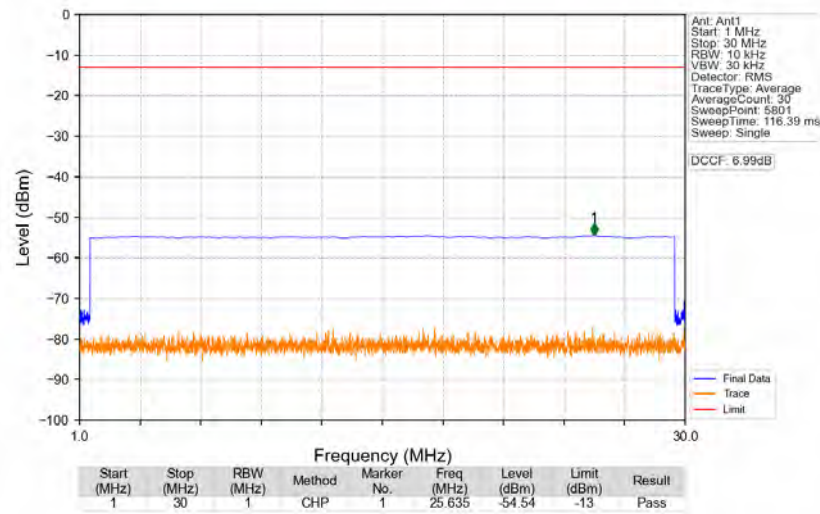
n77d_30kHz_SISO_NTNV_80MHz_DFT-s-OFDM_QPSK_3500.01MHz_Edge_1RB_Left
