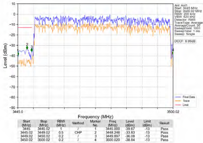
n77d_30kHz_SISO_NTNV_50MHz_CP-OFDM_QPSK_3475.02MHz_Outer_Full
