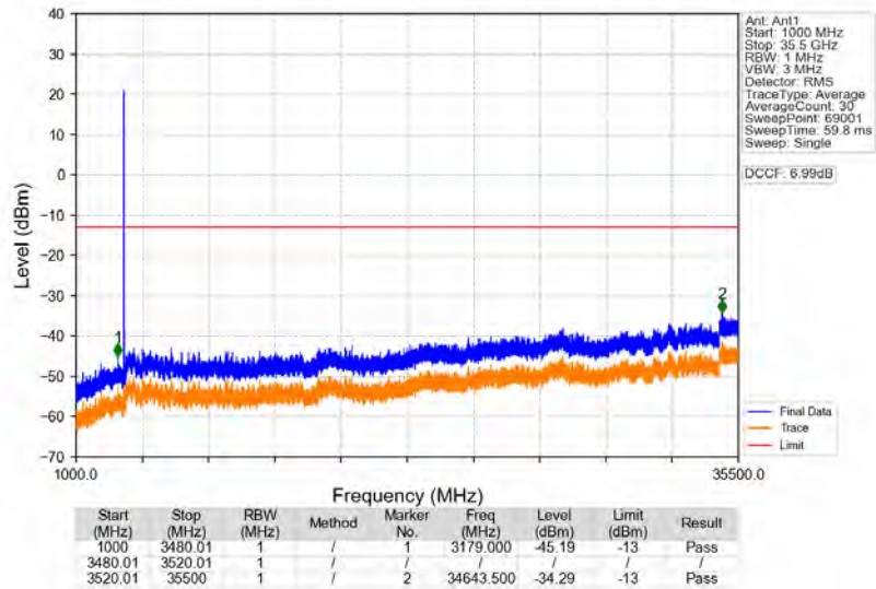
n77d_30kHz_SISO_NTNV_30MHz_CP-OFDM_QPSK_3500.01MHz_Edge_1RB_Left
