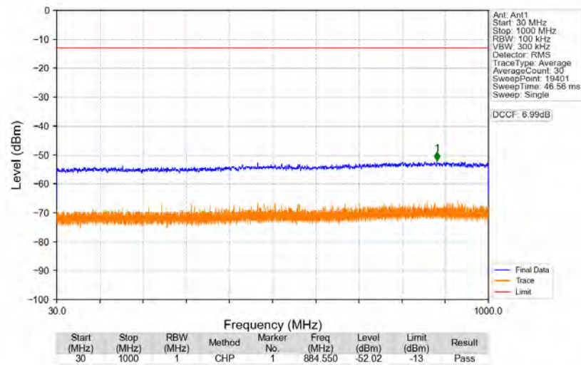
n77d_30kHz_SISO_NTNV_40MHz_DFT-s-OFDM_QPSK_3470.01MHz_Edge_1RB_Left
