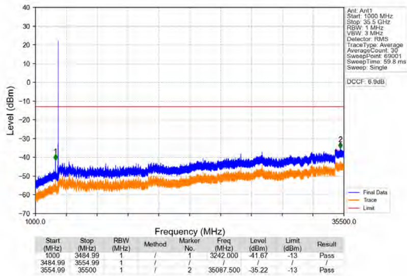
n77d_30kHz_SISO_NTNV_60MHz_DFT-s-OFDM_QPSK_3519.99MHz_Edge_1RB_Right
