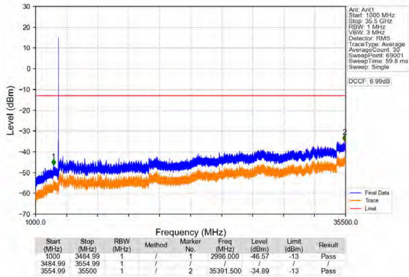
n77d_30kHz_SISO_NTNV_60MHz_CP-OFDM_QPSK_3519.99MHz_Edge_1RB_Right
