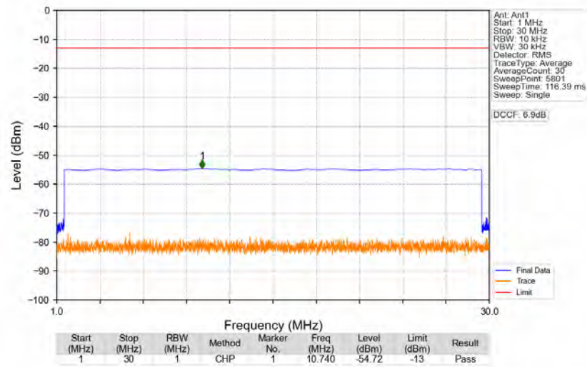
n77d_30kHz_SISO_NTNV_70MHz_CP-OFDM_QPSK_3514.98MHz_Edge_1RB_Right
