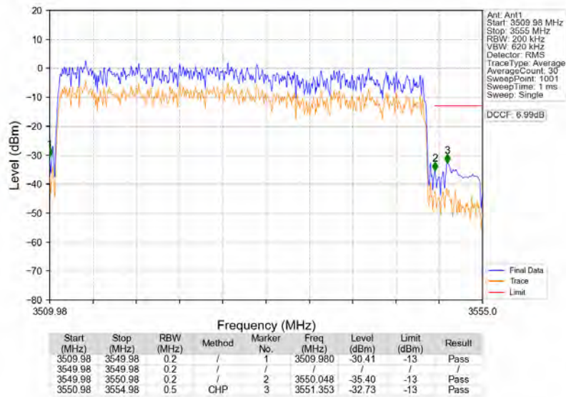
n77d_30kHz_SISO_NTNV_40MHz_CP-OFDM_QPSK_3529.98MHz_Outer_Full
