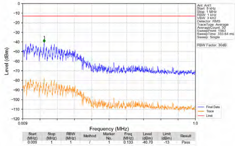
n77d_30kHz_SISO_NTNV_60MHz_CP-OFDM_QPSK_3500.01MHz_Edge_1RB_Left
