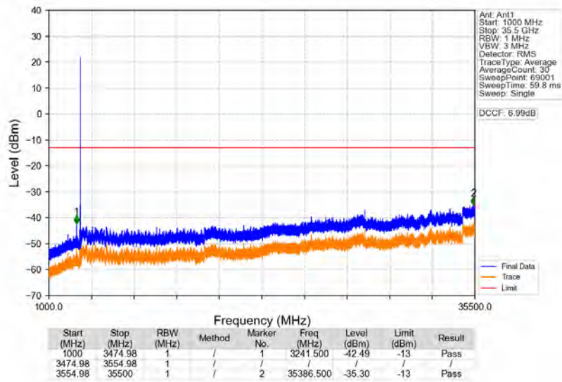
n77d_30kHz_SISO_NTNV_70MHz_DFT-s-OFDM_QPSK_3514.98MHz_Edge_1RB_Right
