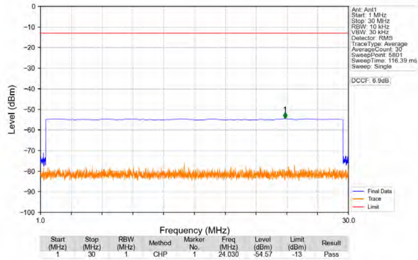
n77d_30kHz_SISO_NTNV_30MHz_CP-OFDM_QPSK_3465MHz_Edge_1RB_Left
