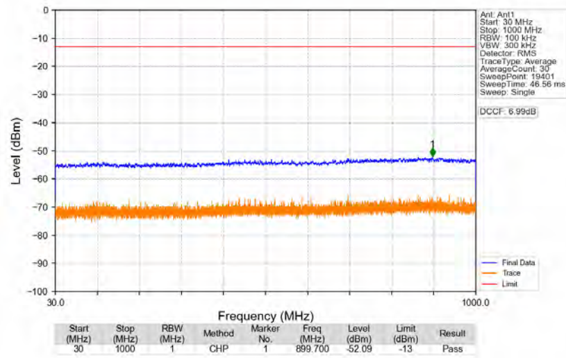
n77d_30kHz_SISO_NTNV_70MHz_DFT-s-OFDM_QPSK_3500.01MHz_Edge_1RB_Left
