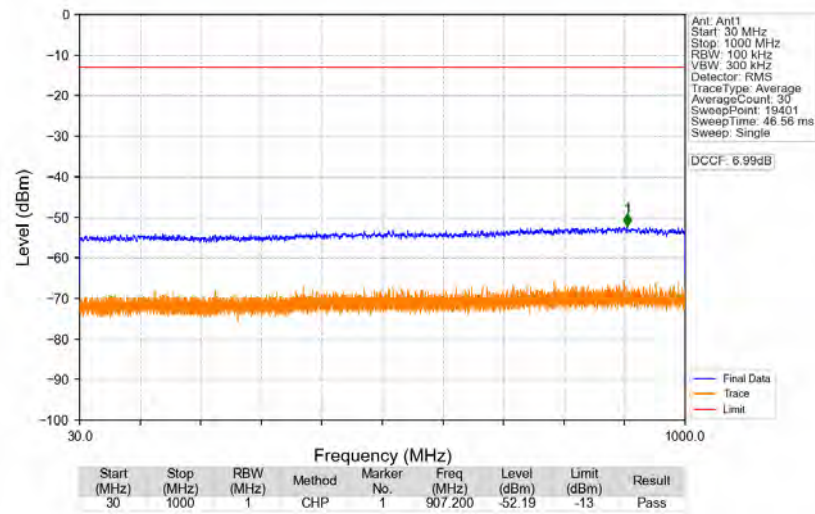
n77d_30kHz_SISO_NTNV_40MHz_DFT-s-OFDM_QPSK_3500.01MHz_Edge_1RB_Left
