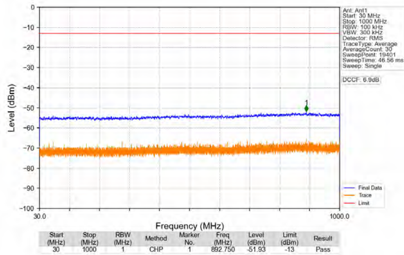
n77d_30kHz_SISO_NTNV_60MHz_DFT-s-OFDM_QPSK_3519.99MHz_Edge_1RB_Right
