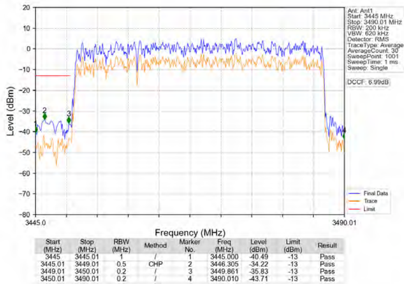
n77d_30kHz_SISO_NTNV_40MHz_DFT-s-OFDM_QPSK_3470.01MHz_Outer_Full
