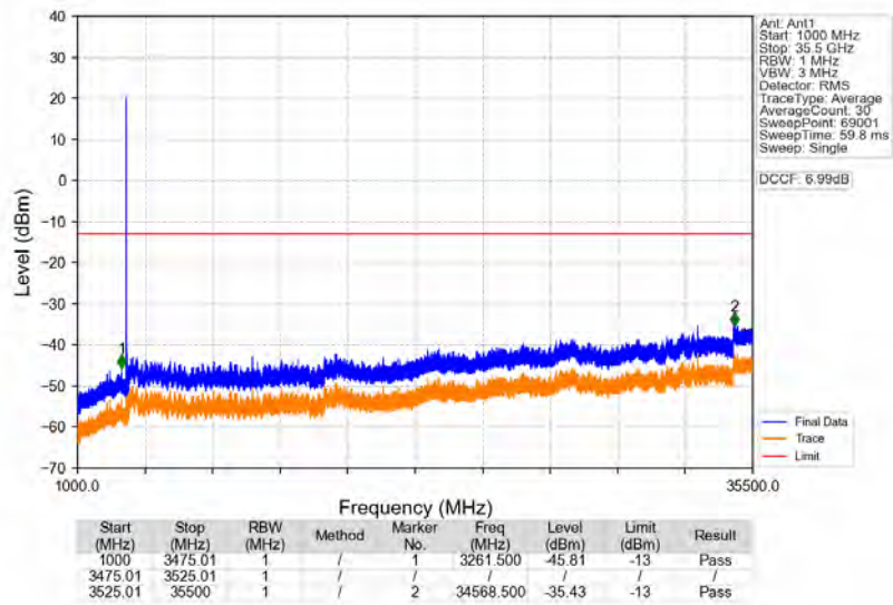
n77d_30kHz_SISO_NTNV_40MHz_CP-OFDM_QPSK_3500.01MHz_Edge_1RB_Left
