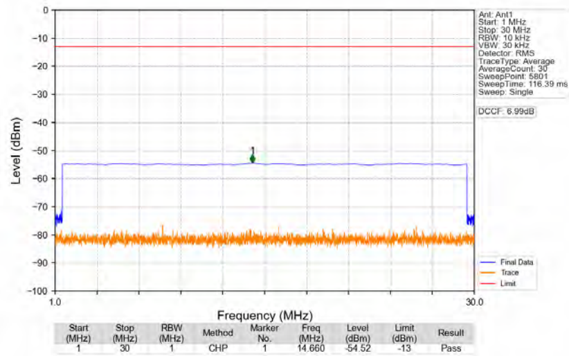
n77d_30kHz_SISO_NTNV_80MHz_DFT-s-OFDM_QPSK_3510MHz_Edge_1RB_Right
