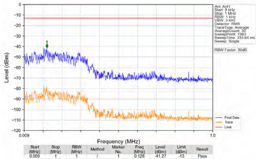
n77d_30kHz_SISO_NTNV_40MHz_DFT-s-OFDM_QPSK_3529.98MHz_Edge_1RB_Right
