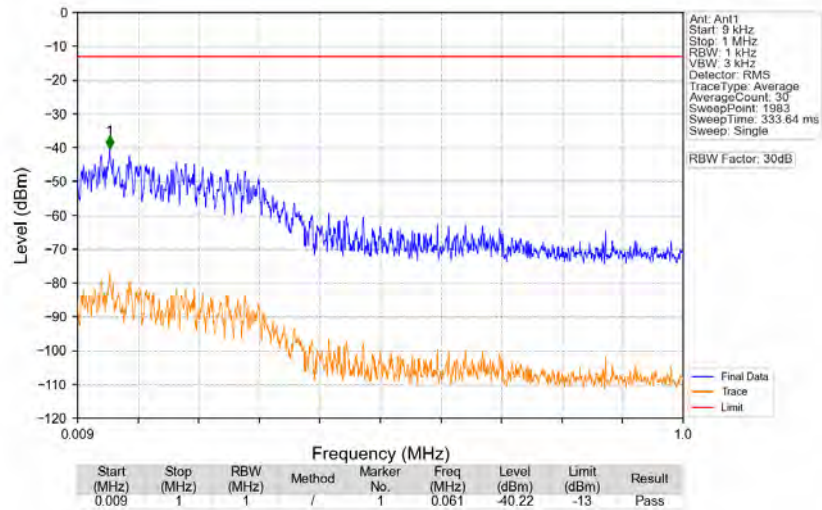
n77d_30kHz_SISO_NTNV_50MHz_CP-OFDM_QPSK_3475.02MHz_Edge_1RB_Left
