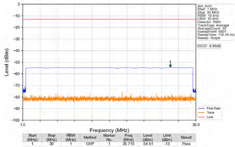
n77d_30kHz_SISO_NTNV_50MHz_DFT-s-OFDM_QPSK_3475.02MHz_Edge_1RB_Left
