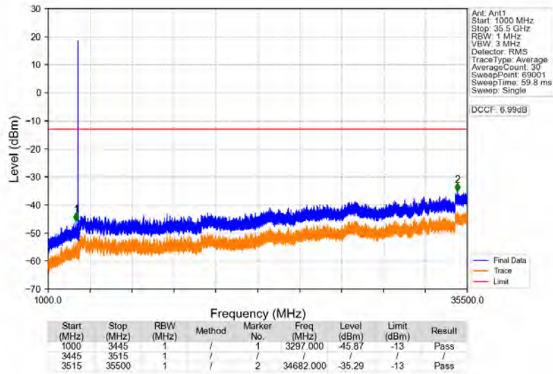
n77d_30kHz_SISO_NTNV_60MHz_CP-OFDM_QPSK_3480MHz_Edge_1RB_Left
