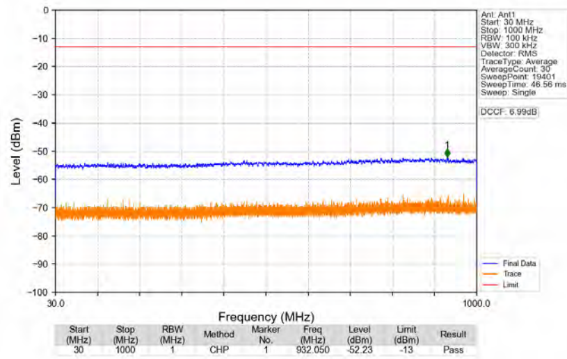
n77d_30kHz_SISO_NTNV_60MHz_DFT-s-OFDM_QPSK_3500.01MHz_Edge_1RB_Left
