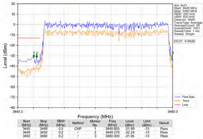
n77d_30kHz_SISO_NTNV_30MHz_CP-OFDM QPSK_3465MHz_Outer_Full
