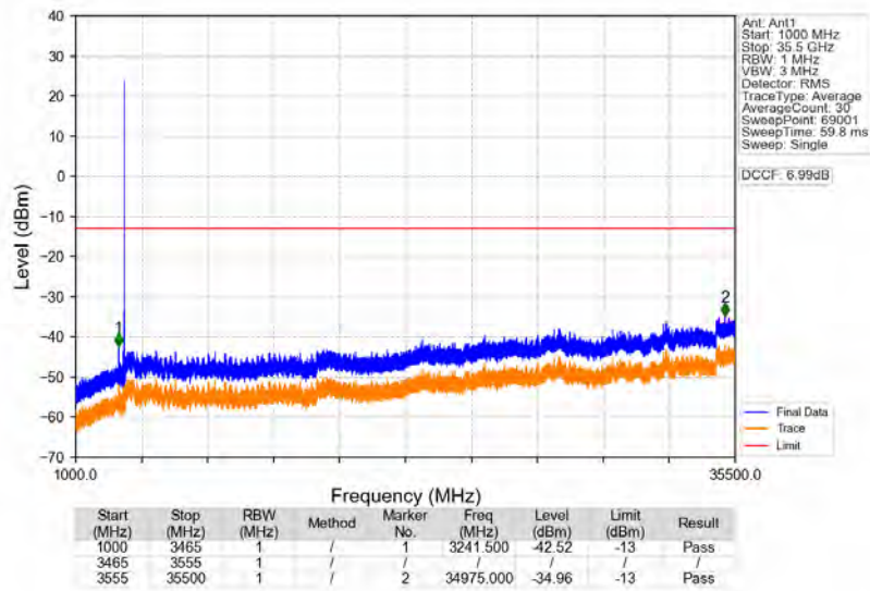
n77d_30kHz_SISO_NTNV_80MHz_DFT-s-OFDM_PI/2_BPSK_3510MHz_Edge_1RB_Right
