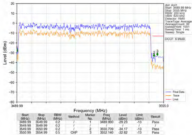
n77d_30kHz_SISO_NTNV_60MHz_CP-OFDM_QPSK_3519.99MHz_Outer_Full
