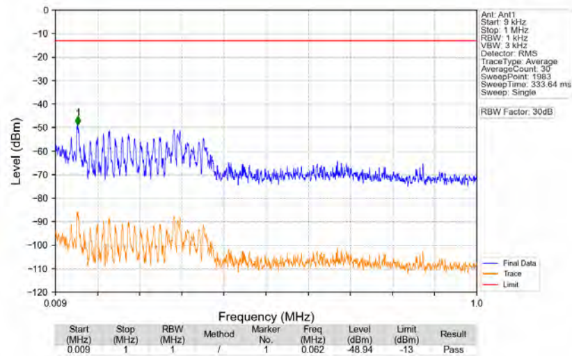
n77d_30kHz_SISO_NTNV_70MHz_DFT-s-OFDM_QPSK_3514.98MHz_Edge_1RB_Right
