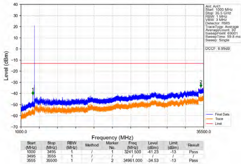
n77d_30kHz_SISO_NTNV_50MHz_DFT-s-OFDM_PI/2_BPSK_3525MHz_Edge_1RB_Right
