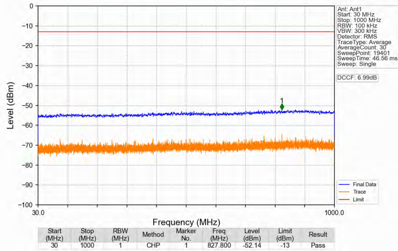
n77d_30kHz_SISO_NTNV_30MHz_CP-OFDM_QPSK_3500.01MHz_Edge_1RB_Left
