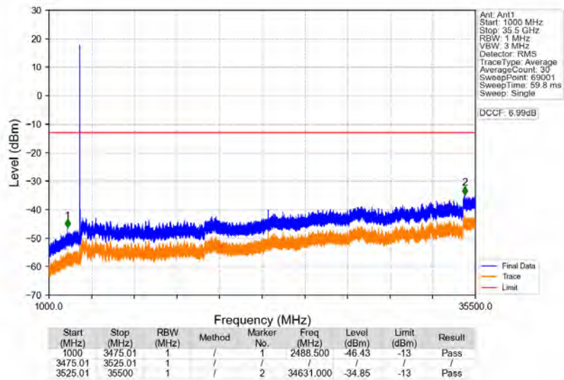
n77d_30kHz_SISO_NTNV_40MHz_DFT-s-OFDM_QPSK_3500.01MHz_Edge_1RB_Left
