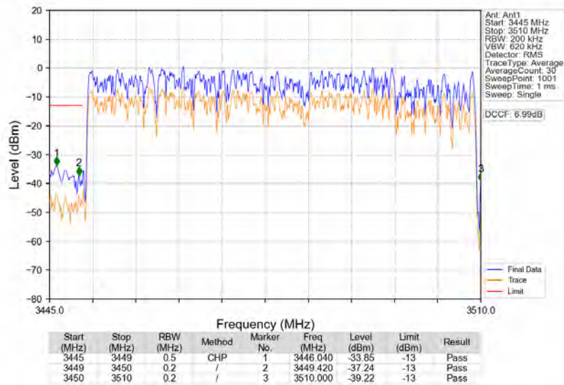
n77d_30kHz_SISO_NTNV_60MHz_DFT-s-OFDM_QPSK_3480MHz_Outer_Full
