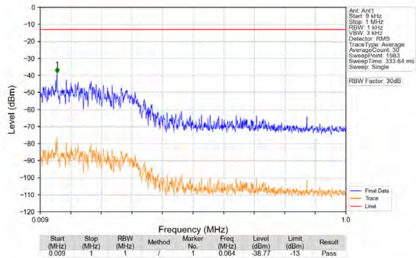
n77d_30kHz_SISO_NTNV_60MHz_CP-OFDM_QPSK_3480MHz_Edge_1RB_Left
