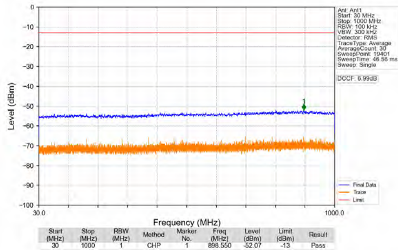
n77d_30kHz_SISO_NTNV_40MHz_DFT-s-OFDM_QPSK_3529.98MHz_Edge_1RB_Right
