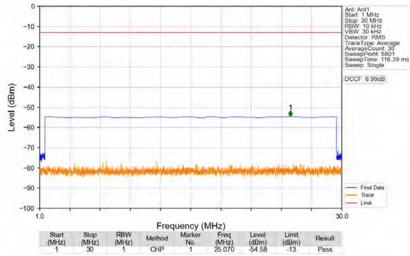
n77d_30kHz_SISO_NTNV_50MHz_DFT-s-OFDM_QPSK_3525MHz_Edge_1RB_Right
