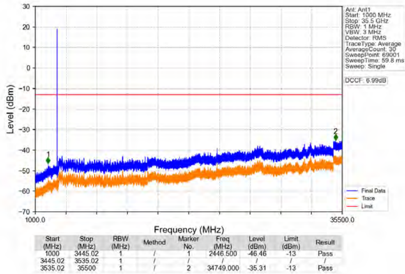
n77d_30kHz_SISO_NTNV_80MHz_DFT-s-OFDM_QPSK_3490.02MHz_Edge_1RB_Left
