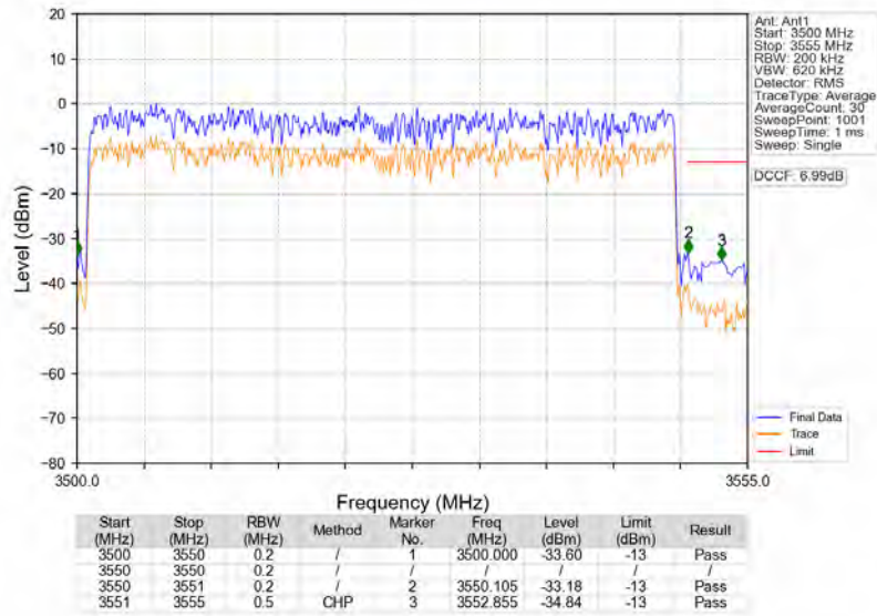
n77d_30kHz_SISO_NTNV_50MHz_CP-OFDM_QPSK_3525MHz_Outer_Full
