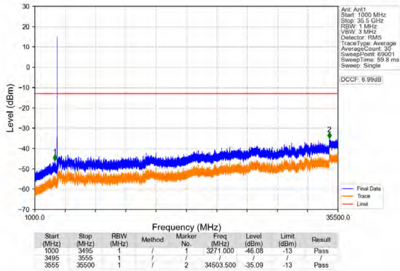
n77d_30kHz_SISO_NTNV_50MHz_CP-OFDM_QPSK_3525MHz_Edge_1RB_Right
