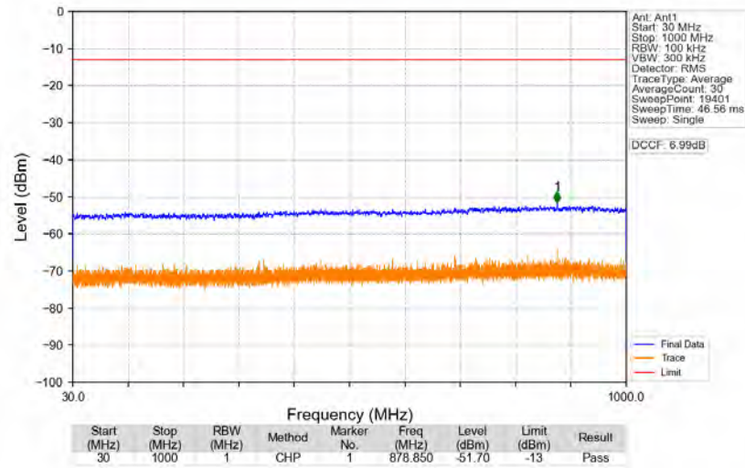
n77d_30kHz_SISO_NTNV_30MHz_CP-OFDM_QPSK_3534.99MHz_Edge_1RB_Right
