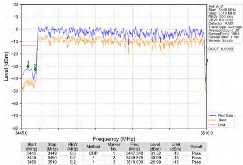
n77d_30kHz_SISO_NTNV_60MHz_DFT-s-OFDM_PI/2_BPSK_3480MHz_Outer_Full
