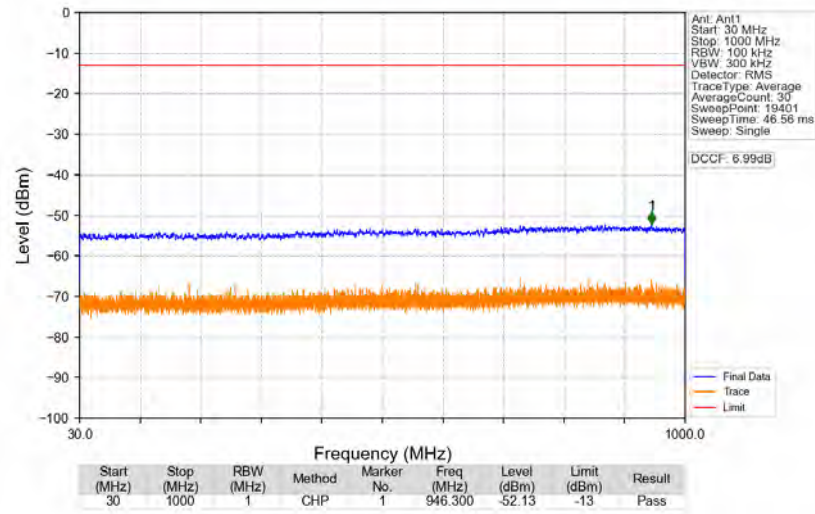
n77d_30kHz_SISO_NTNV_60MHz_CP-OFDM_QPSK_3500.01MHz_Edge_1RB_Left
