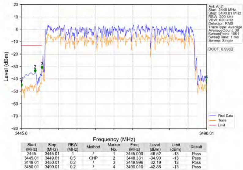
n77d_30kHz_SISO_NTNV_40MHz_DFT-s-OFDM_PI/2_BPSK_3470.01MHz_Outer_Full
