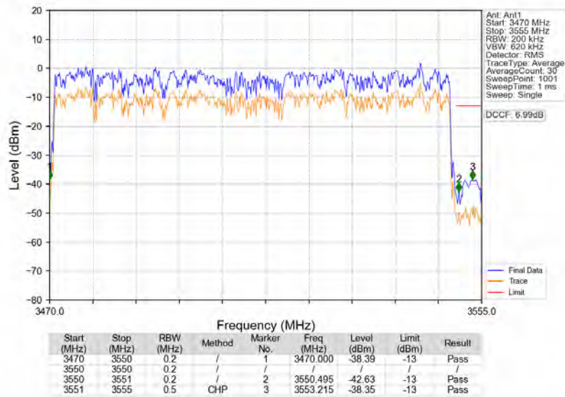
n77d_30kHz_SISO_NTNV_80MHz_DFT-s-OFDM_QPSK_3510MHz_Outer_Full
