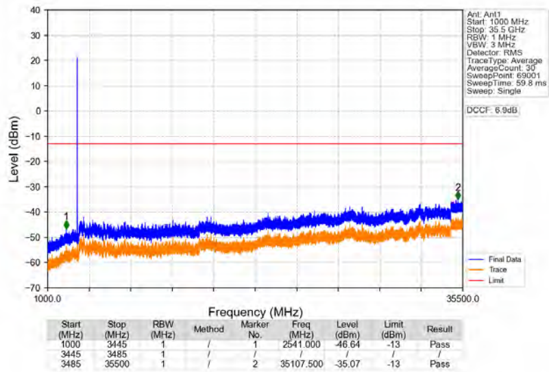
n77d_30kHz_SISO_NTNV_30MHz_CP-OFDM QPSK_3465MHz_Edge_1RB_Left
