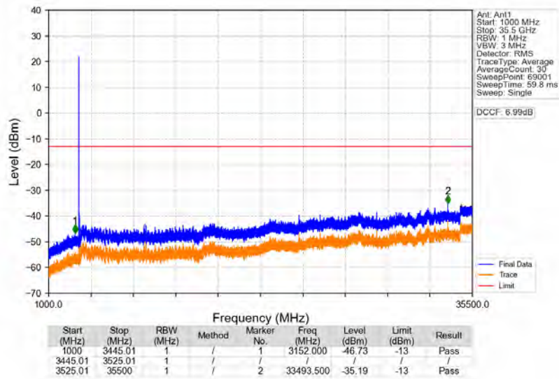
n77d_30kHz_SISO_NTNV_70MHz_DFT-s-OFDM_QPSK_3485.01MHz_Edge_1RB_Left
