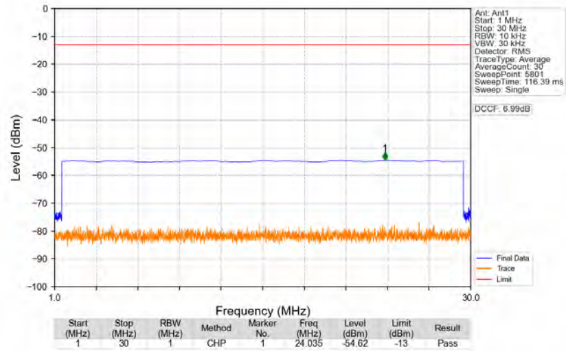
n77d_30kHz_SISO_NTNV_70MHz_DFT-s-OFDM_QPSK_3500.01MHz_Edge_1RB_Left
