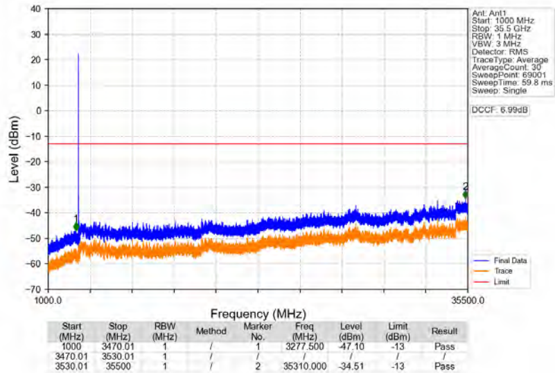
n77d_30kHz_SISO_NTNV_50MHz_CP-OFDM_QPSK_3500.01MHz_Edge_1RB_Left
