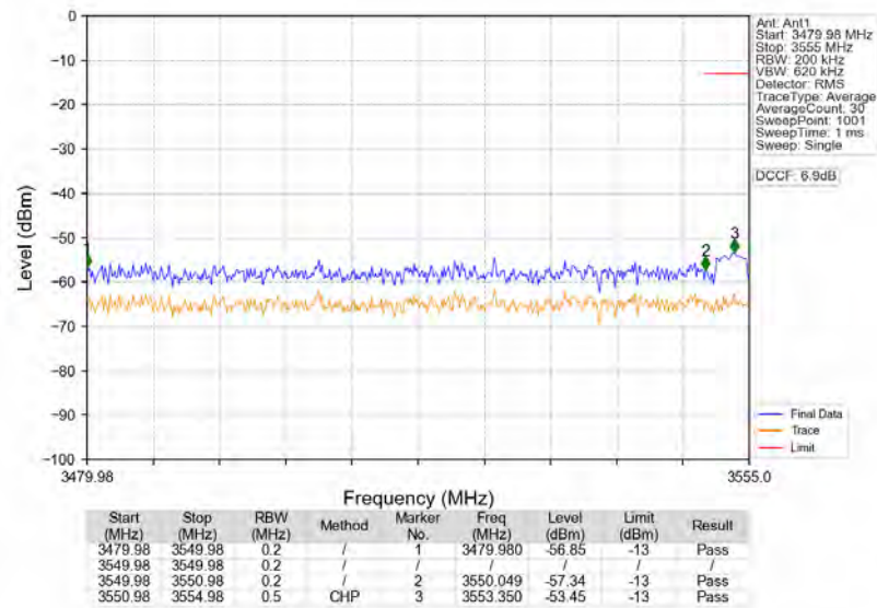
n77d_30kHz_SISO_NTNV_70MHz_DFT-s-OFDM_QPSK_3514.98MHz_Outer_Full
