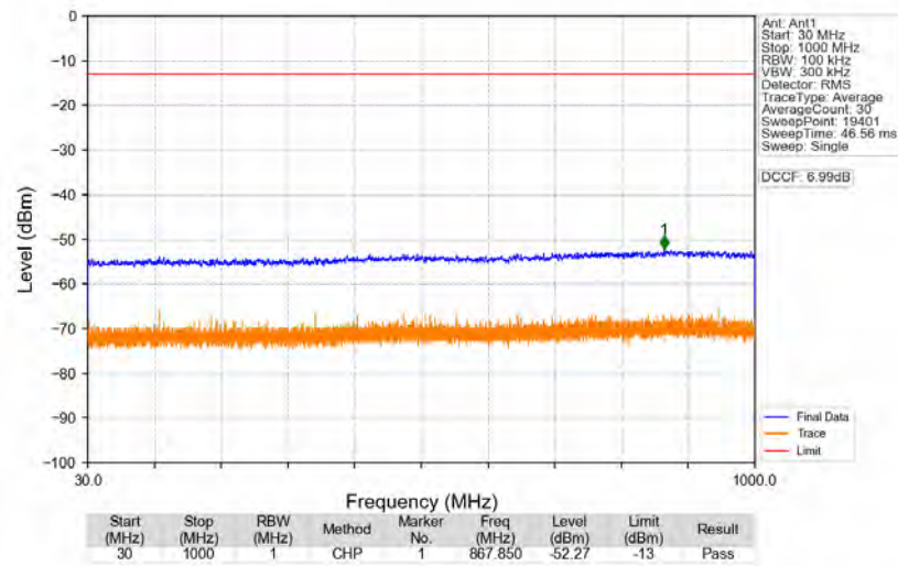
n77d_30kHz_SISO_NTNV_70MHz_DFT-s-OFDM_QPSK_3514.98MHz_Edge_1RB_Right
