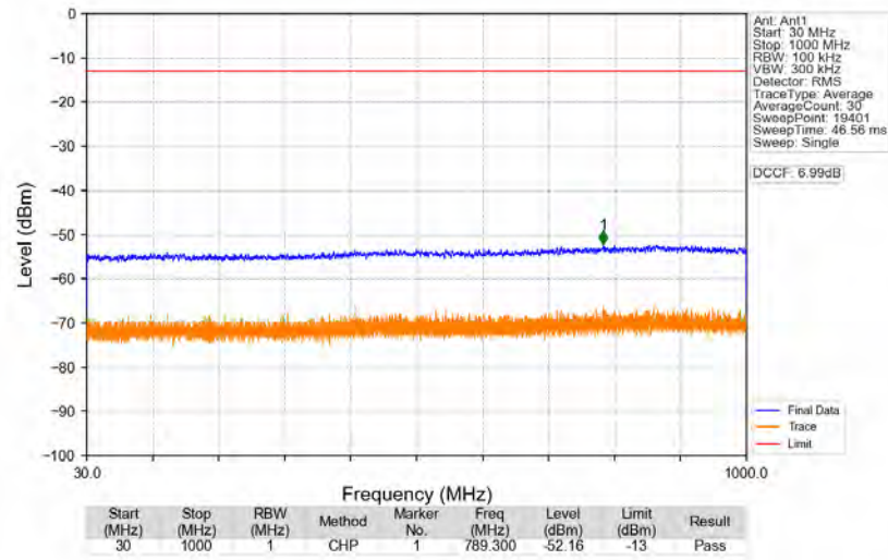
n77d_30kHz_SISO_NTNV_80MHz_DFT-s-OFDM_QPSK_3500.01MHz_Edge_1RB_Left
