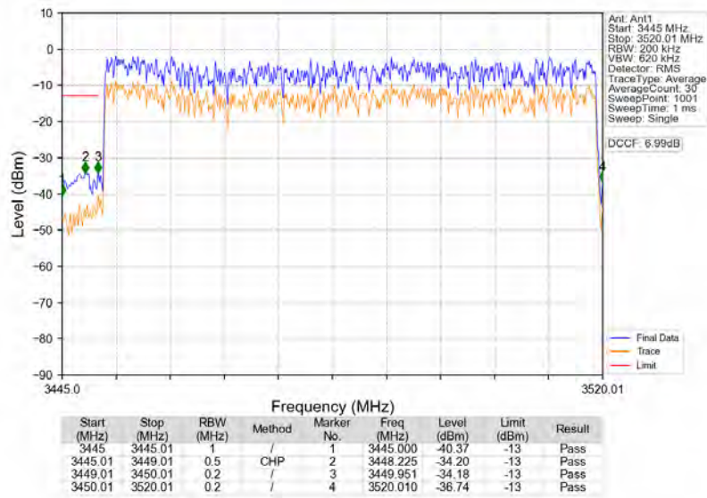
n77d_30kHz_SISO_NTNV_70MHz_CP-OFDM_QPSK_3485.01MHz_Outer_Full
