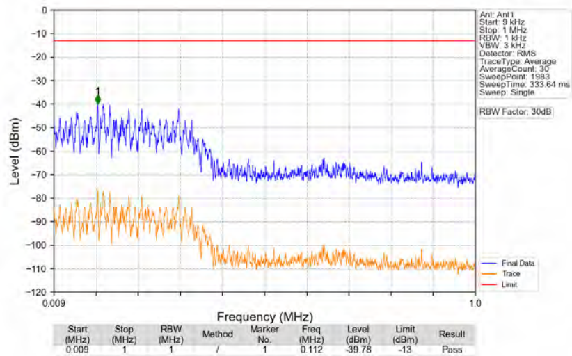
n77d_30kHz_SISO_NTNV_60MHz_DFT-s-OFDM_QPSK_3519.99MHz_Edge_1RB_Right
