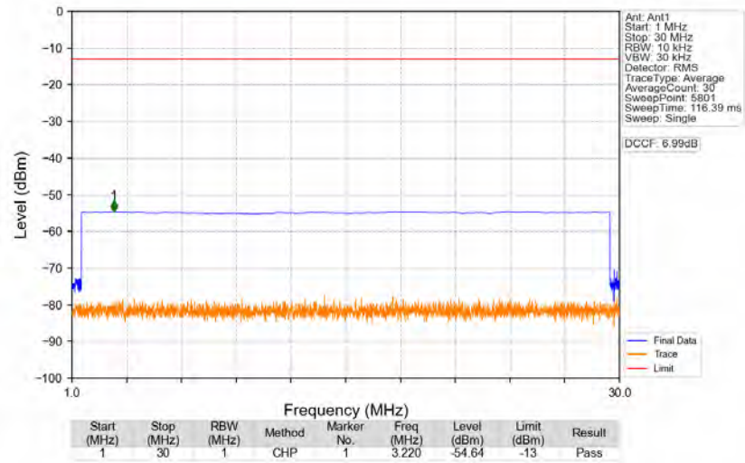
n77d_30kHz_SISO_NTNV_60MHz_CP-OFDM_QPSK_3500.01MHz_Edge_1RB_Left
