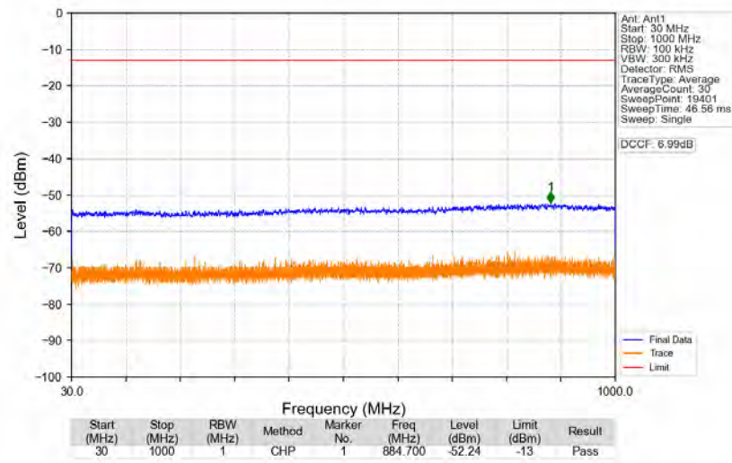
n77d_30kHz_SISO_NTNV_40MHz_CP-OFDM_QPSK_3500.01MHz_Edge_1RB_Left
