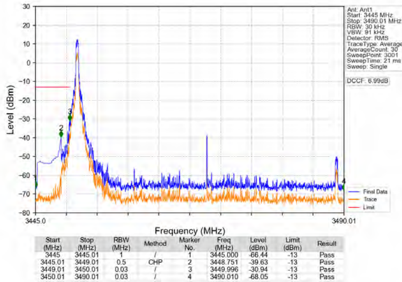
n77d_30kHz_SISO_NTNV_40MHz_CP-OFDM_QPSK_3470.01MHz_Edge_1RB_Left
