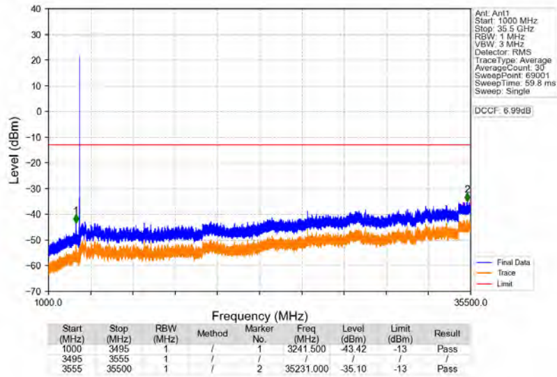
n77d_30kHz_SISO_NTNV_50MHz_DFT-s-OFDM_QPSK_3525MHz_Edge_1RB_Right
