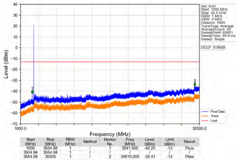
n77d_30kHz_SISO_NTNV_40MHz_DFT-s-OFDM_QPSK_3529.98MHz_Edge_1RB_Right
