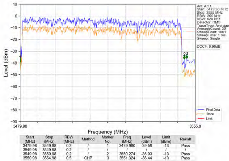
n77d_30kHz_SISO_NTNV_70MHz_CP-OFDM_QPSK_3514.98MHz_Outer_Full
