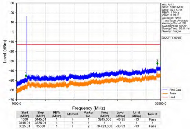
n77d_30kHz_SISO_NTNV_70MHz_CP-OFDM_QPSK_3485.01MHz_Edge_1RB_Left
