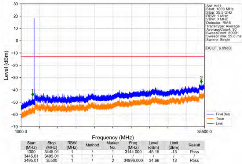
n77d_30kHz_SISO_NTNV_40MHz_DFT-s-OFDM_QPSK_3470.01MHz_Edge_1RB_Left
