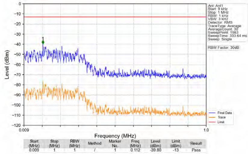
n77d_30kHz_SISO_NTNV_70MHz_DFT-s-OFDM_QPSK_3500.01MHz_Edge_1RB_Left
