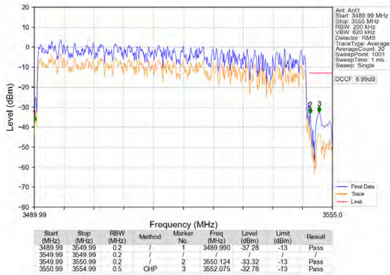
n77d_30kHz_SISO_NTNV_60MHz_DFT-s-OFDM_QPSK_3519.99MHz_Outer_Full
