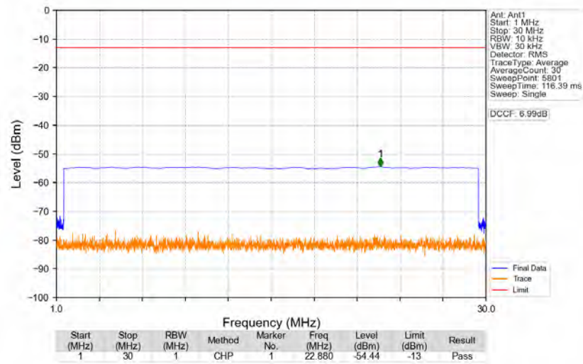
n77d_30kHz_SISO_NTNV_70MHz_CP-OFDM_QPSK_3485.01MHz_Edge_1RB_Left
