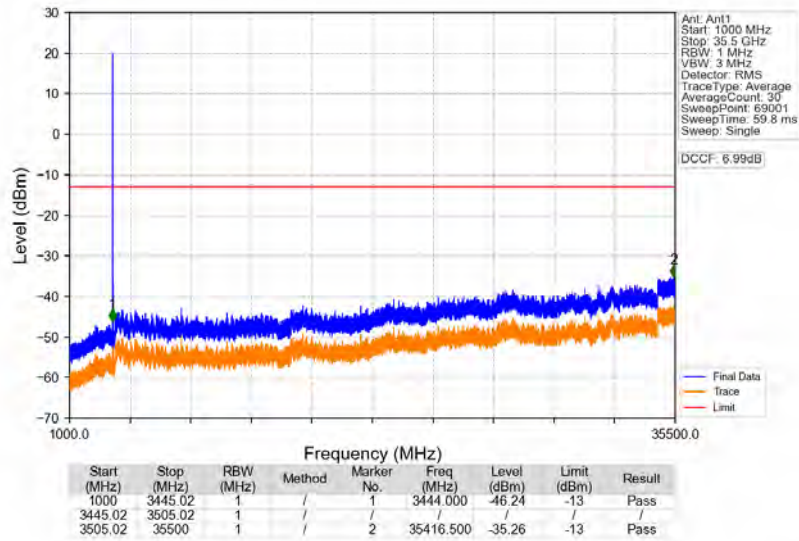
n77d_30kHz_SISO_NTNV_50MHz_DFT-s-OFDM_QPSK_3475.02MHz_Edge_1RB_Left
