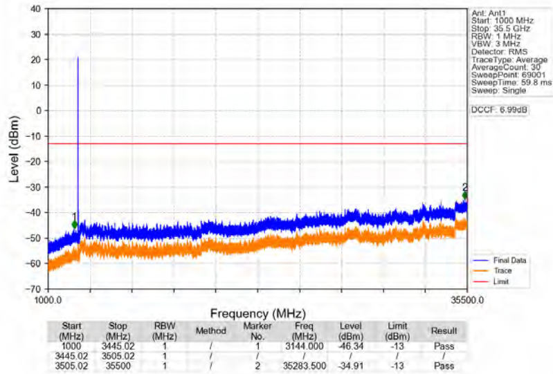
n77d_30kHz_SISO_NTNV_50MHz_DFT-s-OFDM PI/2 BPSK 3475.02MHz_Edge_1RB_Left
