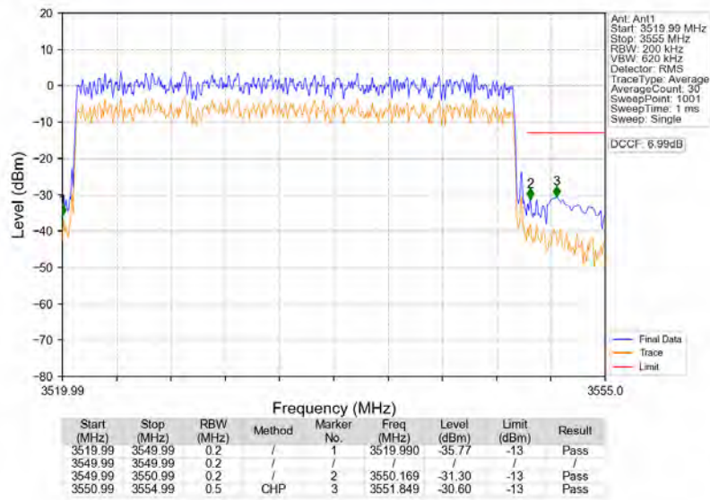
n77d_30kHz_SISO_NTNV_30MHz_CP-OFDM_QPSK_3534.99MHz_Outer_Full
