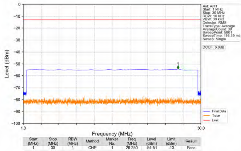
n77d_30kHz_SISO_NTNV_60MHz_DFT-s-OFDM_QPSK_3519.99MHz_Edge_1RB_Right
