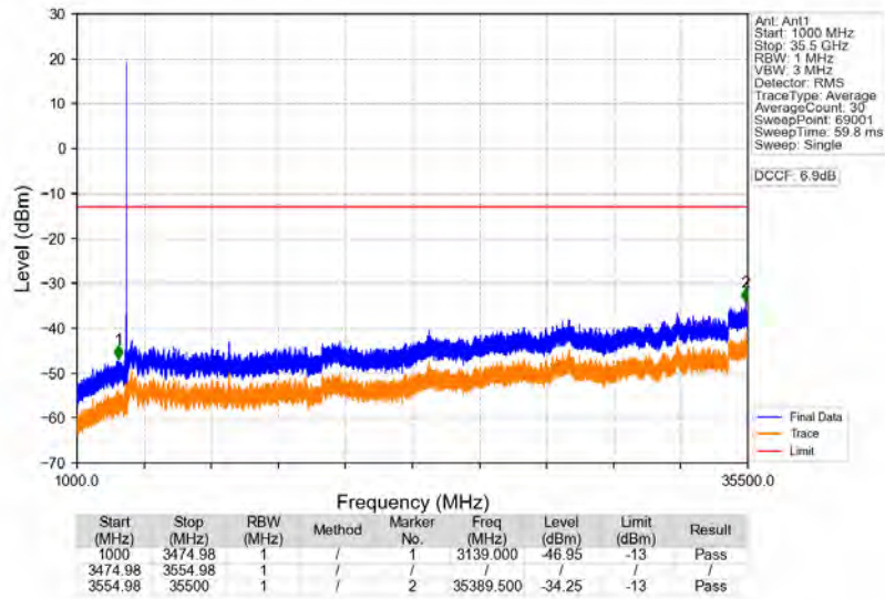
n77d_30kHz_SISO_NTNV_70MHz_CP-OFDM_QPSK_3514.98MHz_Edge_1RB_Right
