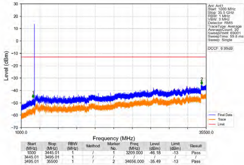
n77d_30kHz_SISO_NTNV_40MHz_CP-OFDM_QPSK_3470.01MHz_Edge_1RB_Left
