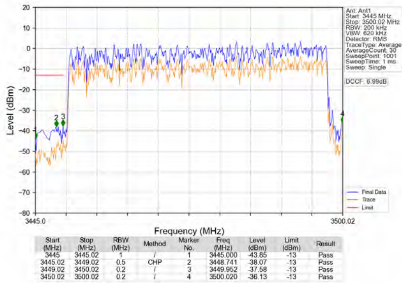
n77d_30kHz_SISO_NTNV_50MHz_DFT-s-OFDM PI/2 BPSK 3475.02MHz_Outer_Full
