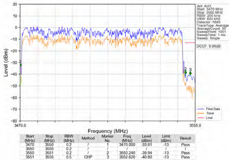
n77d_30kHz_SISO_NTNV_80MHz_DFT-s-OFDM_PI/2_BPSK_3510MHz_Outer_Full
