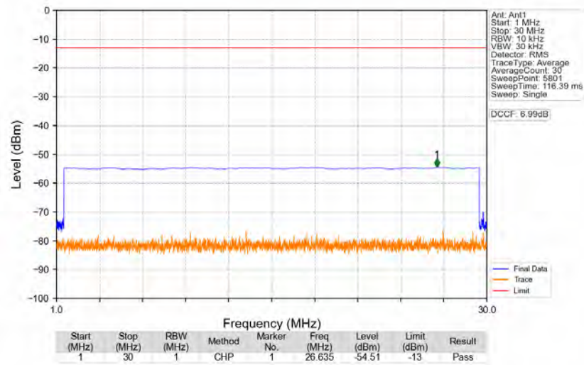
n77d_30kHz_SISO_NTNV_40MHz_DFT-s-OFDM_QPSK_3529.98MHz_Edge_1RB_Right
