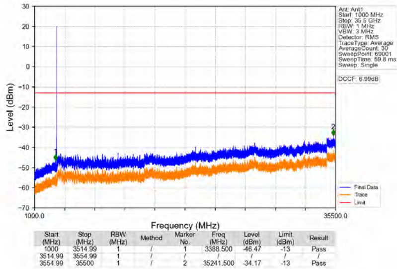
n77d_30kHz_SISO_NTNV_30MHz_CP-OFDM_QPSK_3534.99MHz_Edge_1RB_Right
