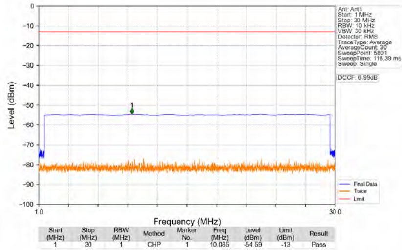
n77d_30kHz_SISO_NTNV_50MHz_CP-OFDM_QPSK_3525MHz_Edge_1RB_Right
