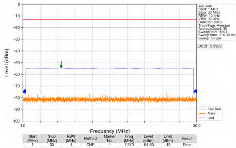
n77d_30kHz_SISO_NTNV_60MHz_CP-OFDM_QPSK_3480MHz_Edge_1RB_Left
