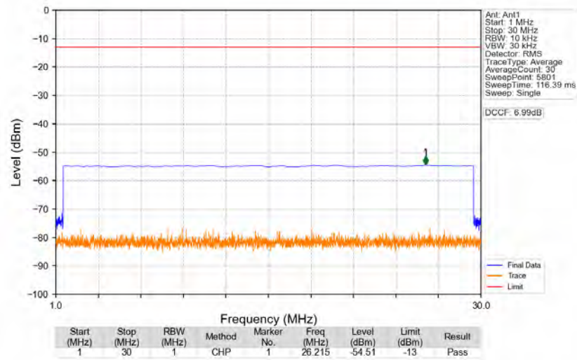
n77d_30kHz_SISO_NTNV_60MHz_DFT-s-OFDM_QPSK_3500.01MHz_Edge_1RB_Left
