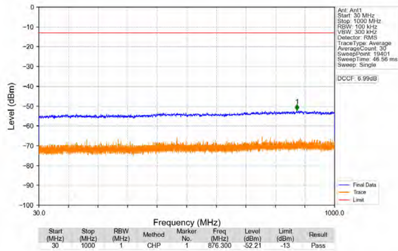
n77d_30kHz_SISO_NTNV_60MHz_DFT-s-OFDM_QPSK_3480MHz_Edge_1RB_Left
