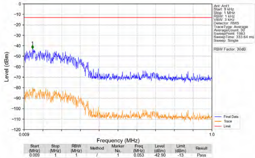
n77d_30kHz_SISO_NTNV_70MHz_CP-OFDM_QPSK_3514.98MHz_Edge_1RB_Right
