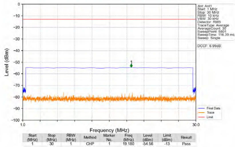
n77d_30kHz_SISO_NTNV_40MHz_DFT-s-OFDM_QPSK_3470.01MHz_Edge_1RB_Left
