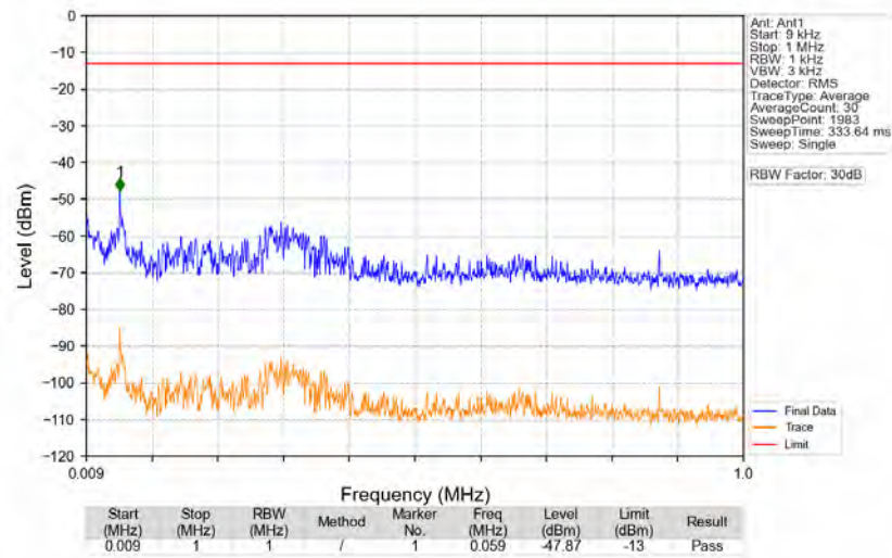
n77d_30kHz_SISO_NTNV_40MHz_CP-OFDM_QPSK_3500.01MHz_Edge_1RB_Left
