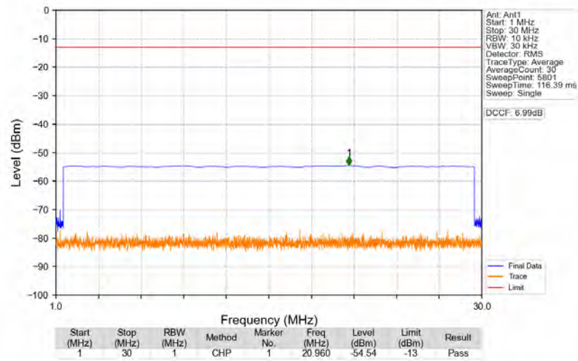
n77d_30kHz_SISO_NTNV_60MHz_DFT-s-OFDM_QPSK_3480MHz_Edge_1RB_Left
