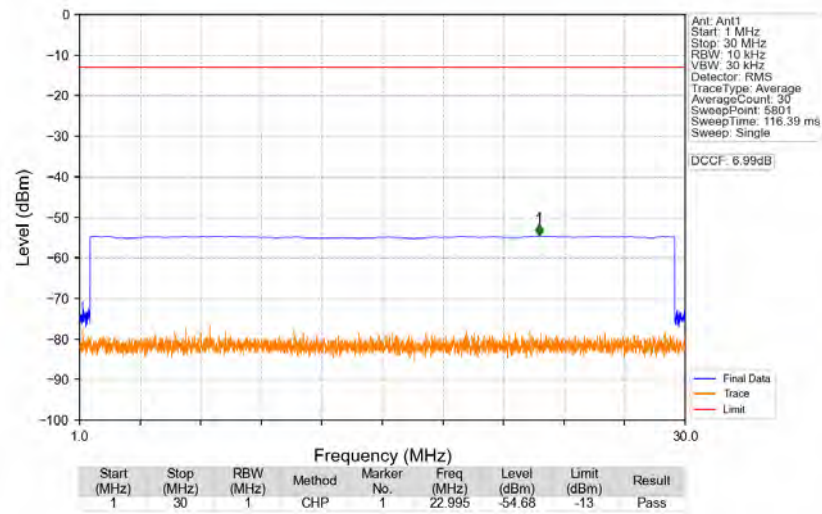
n77d_30kHz_SISO_NTNV_70MHz_DFT-s-OFDM_QPSK_3514.98MHz_Edge_1RB_Right
