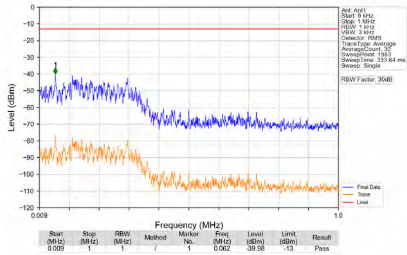
n77d_30kHz_SISO_NTNV_50MHz_DFT-s-OFDM_QPSK_3500.01MHz_Edge_1RB_Left
