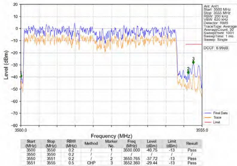
n77d_30kHz_SISO_NTNV_50MHz_DFT-s-OFDM_PI/2_BPSK_3525MHz_Outer_Full
