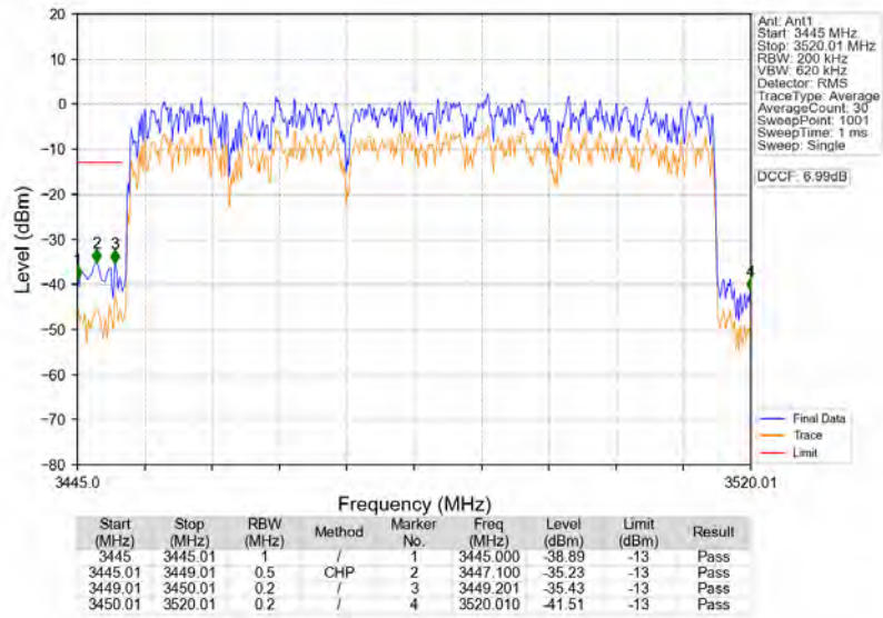
n77d_30kHz_SISO_NTNV_70MHz_DFT-s-OFDM_PI/2_BPSK_3485.01MHz_Outer_Full
