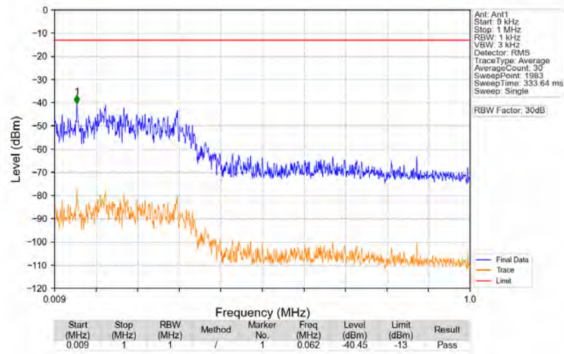
n77d_30kHz_SISO_NTNV_40MHz_DFT-s-OFDM_QPSK_3500.01MHz_Edge_1RB_Left
