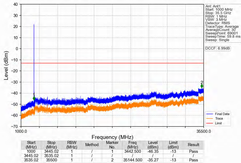
n77d_30kHz_SISO_NTNV_80MHz_DFT-s-OFDM_PI/2_BPSK_3490.02MHz_Edge_1RB_Left
