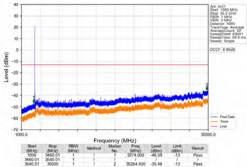
n77d_30kHz_SISO_NTNV_70MHz_CP-OFDM_QPSK_3500.01MHz_Edge_1RB_Left
