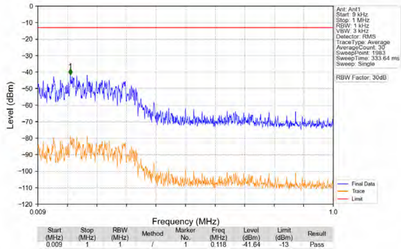
n77d_30kHz_SISO_NTNV_50MHz_DFT-s-OFDM_QPSK_3525MHz_Edge_1RB_Right
