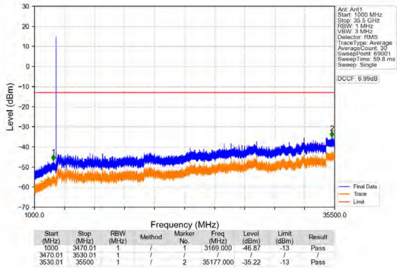
n77d_30kHz_SISO_NTNV_50MHz_DFT-s-OFDM_QPSK_3500.01MHz_Edge_1RB_Left
