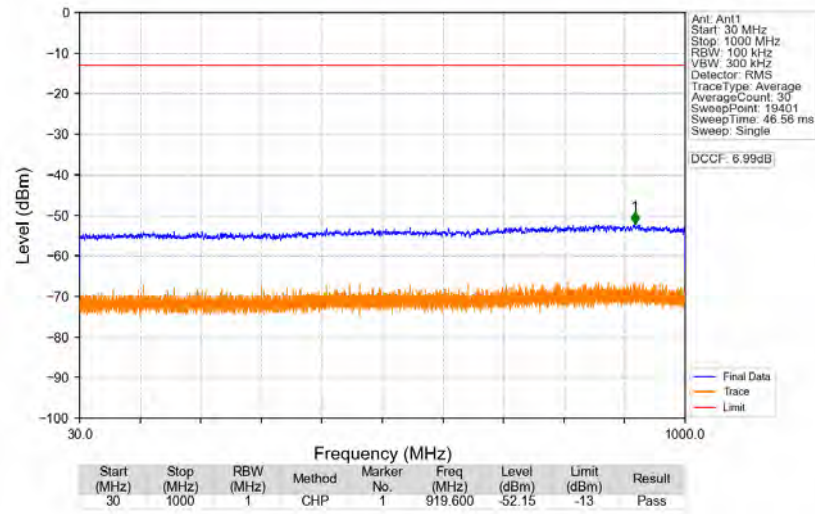
n77d_30kHz_SISO_NTNV_50MHz_CP-OFDM_QPSK_3500.01MHz_Edge_1RB_Left
