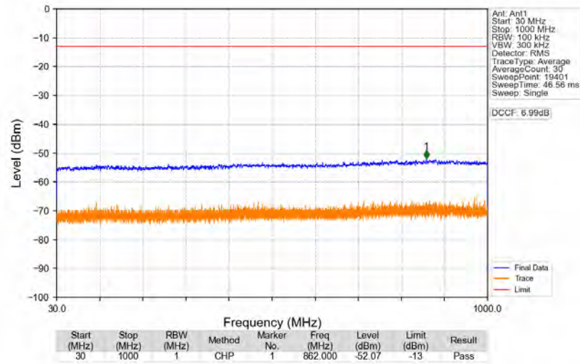
n77d_30kHz_SISO_NTNV_50MHz_DFT-s-OFDM_QPSK_3525MHz_Edge_1RB_Right
