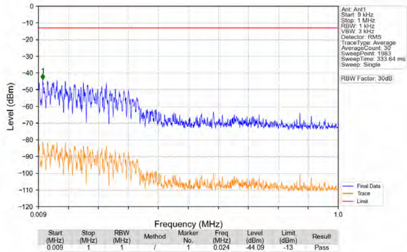
n77d_30kHz_SISO_NTNV_40MHz_CP-OFDM_QPSK_3529.98MHz_Edge_1RB_Right
