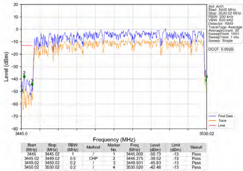
n77d_30kHz_SISO_NTNV_80MHz_DFT-s-OFDM_QPSK_3490.02MHz_Outer_Full
