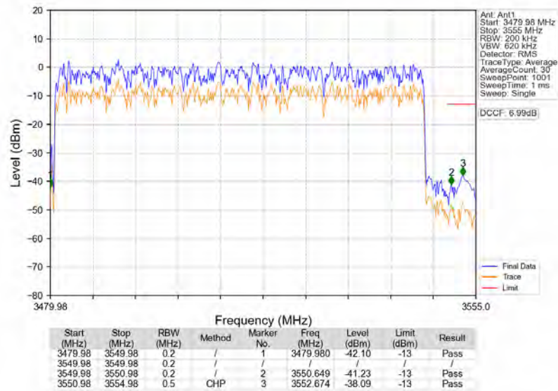
n77d_30kHz_SISO_NTNV_70MHz_DFT-s-OFDM_PI/2_BPSK_3514.98MHz_Outer_Full
