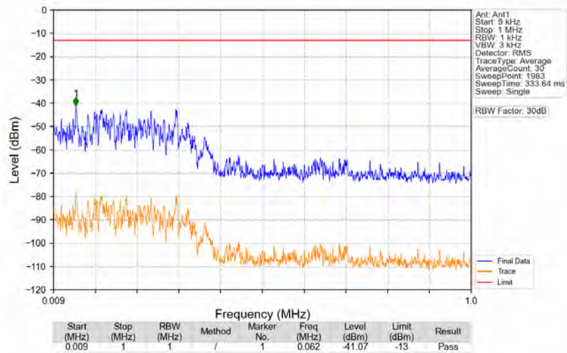
n77d_30kHz_SISO_NTNV_60MHz_DFT-s-OFDM_QPSK_3480MHz_Edge_1RB_Left
