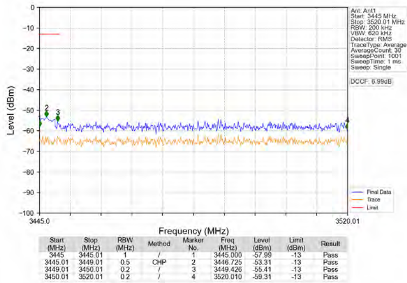
n77d_30kHz_SISO_NTNV_70MHz_DFT-s-OFDM_QPSK_3485.01MHz_Outer_Full
