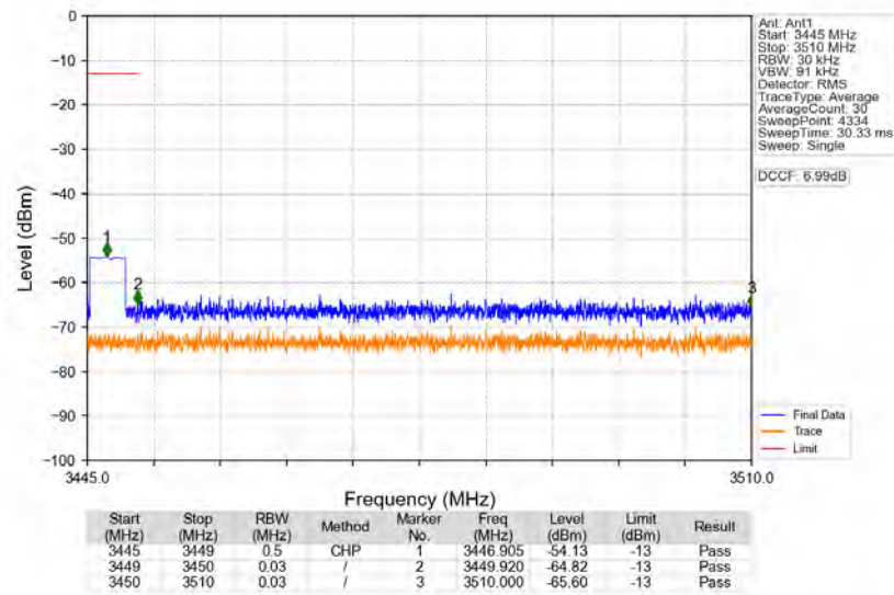
n77d_30kHz_SISO_NTNV_60MHz_CP-OFDM_QPSK_3480MHz_Edge_1RB_Left
