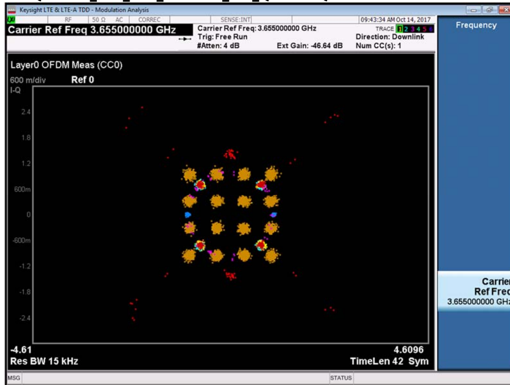
Figure 4.2.2 Modulation Measurements FW2QMBOM1_2x2_10M_3655MHz_Tx2_QPSK+16QAM
