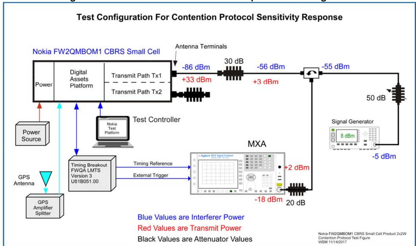
Figure 4.7. Part 90Z Contention Protocol Response Test Configuration
