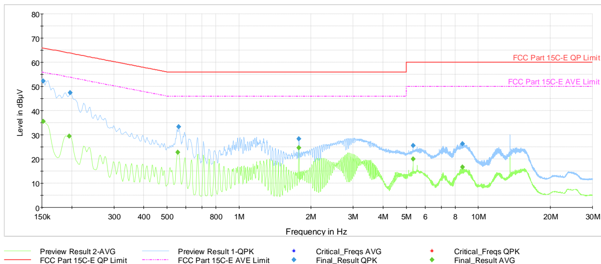
Plot 7-14. AC Line-Conducted Plot (L1, Reader A 848kbps, with Laptop and Magnetic Charger)
