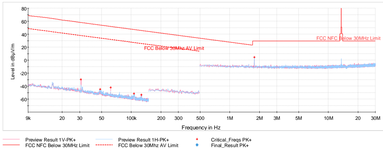
Plot 7-9. Radiated Spurious Emissions 9kHz – 30MHz (Reader A 848kbps, with AC/DC Adapter and Magnetic Charger)
