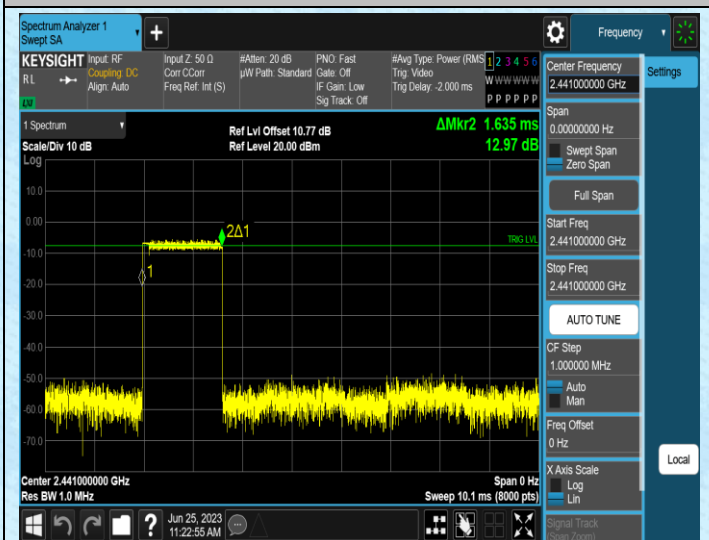
3DH3-Ant1-Hop
