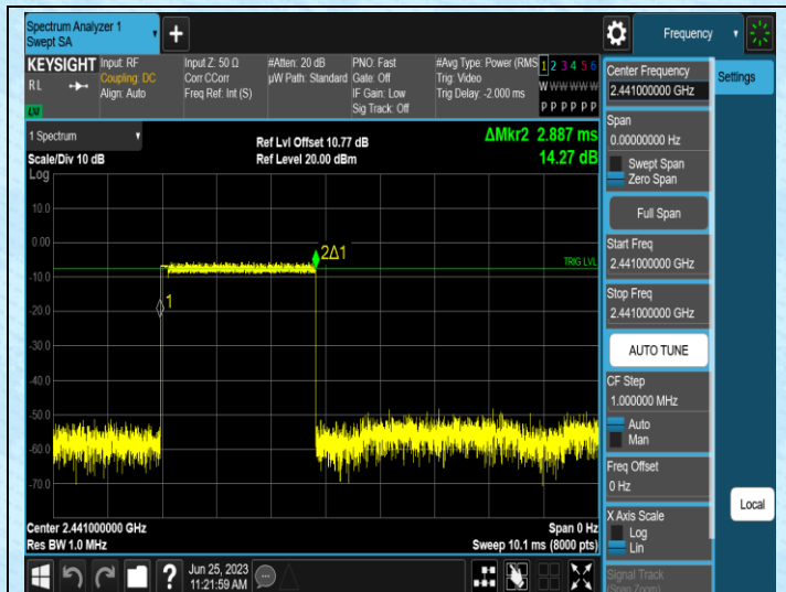
3DH5-Ant1-Hop
