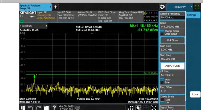
Band41-10MHz-QPSK-41540-1RB#49-0.009~0.15-PASS
