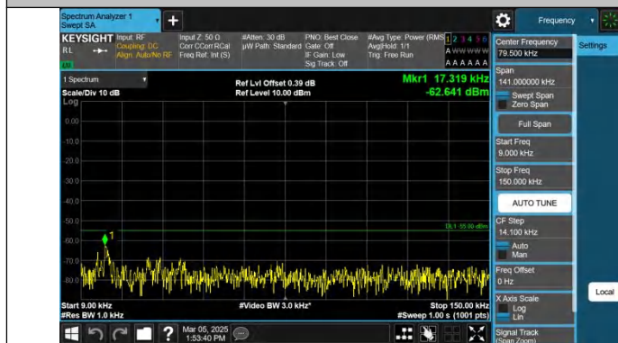
Band41-10MHz-QPSK-41540-1RB#0-0.009~0.15-PASS
