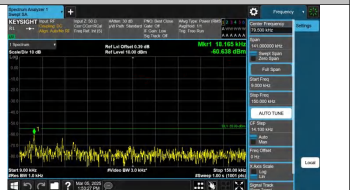
Band41-10MHz-QPSK-40620-1RB#49-0.009~0.15-PASS
