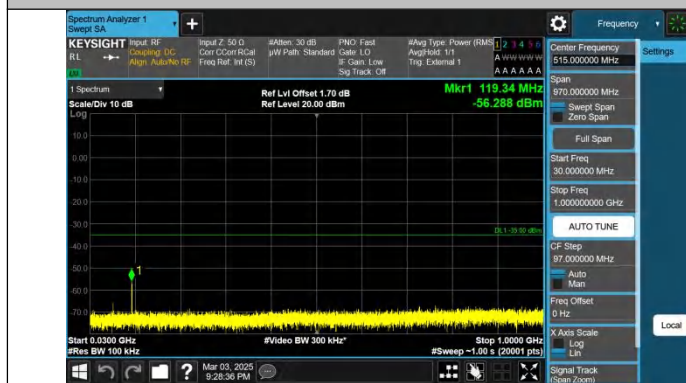
Band41-10MHz-QPSK-41540-1RB#0-30~1000-PASS
