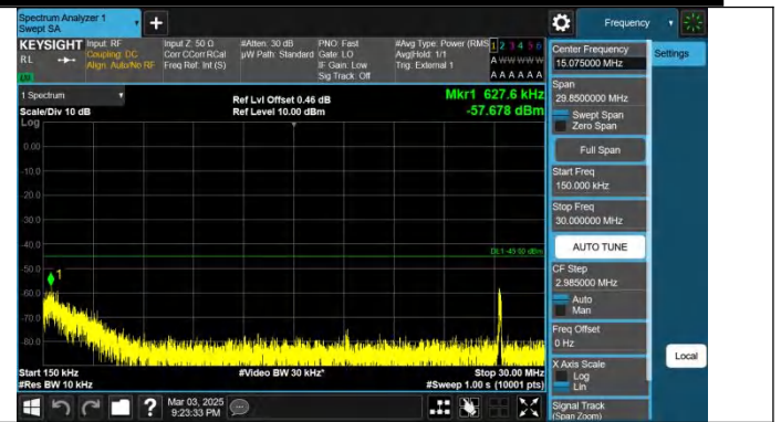
Band41-10MHz-QPSK-40620-1RB#0-0.15~30-PASS
