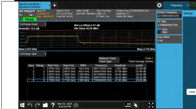
Band41-15MHz-QPSK-41515-75RB#0-PASS
