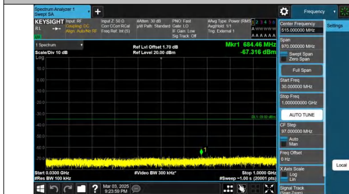
Band41-10MHz-QPSK-40620-1RB#0-30~1000-PASS
