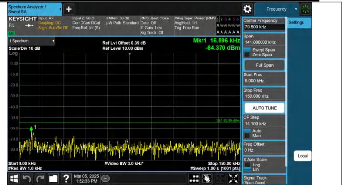
Band41-5MHz-QPSK-41565-1RB#24-0.009~0.15-PASS
