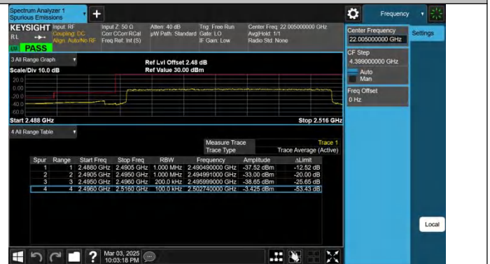
Band41-20MHz-QPSK-39750-100RB#0-PASS
