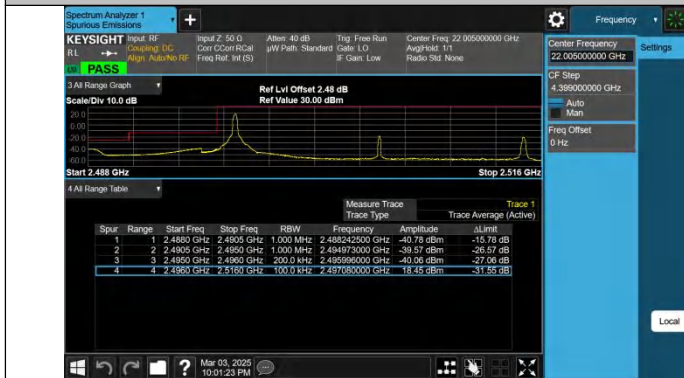
Band41-20MHz-QPSK-39750-1RB#0-PASS
