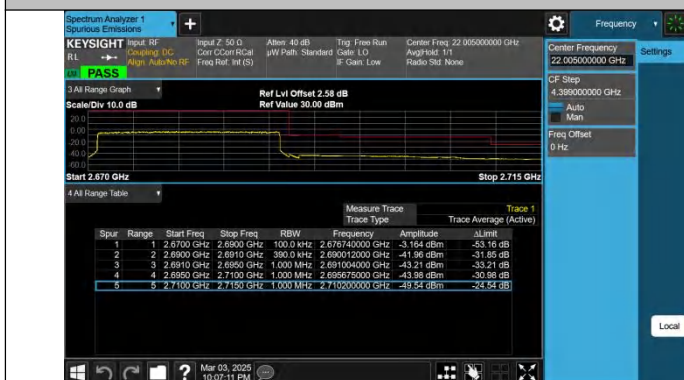
Band41-20MHz-QPSK-41490-100RB#0-PASS
