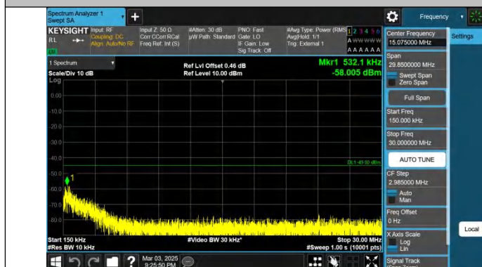
Band41-10MHz-QPSK-40620-1RB#49-0.15~30-PASS
