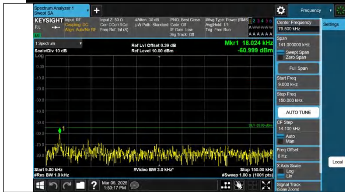
Band41-10MHz-QPSK-40620-1RB#0-0.009~0.15-PASS
