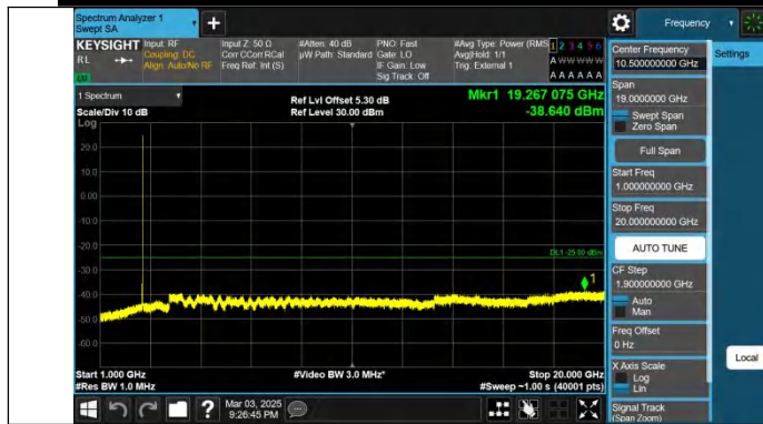
Band41-10MHz-QPSK-40620-1RB#49-1000~20000-PASS
