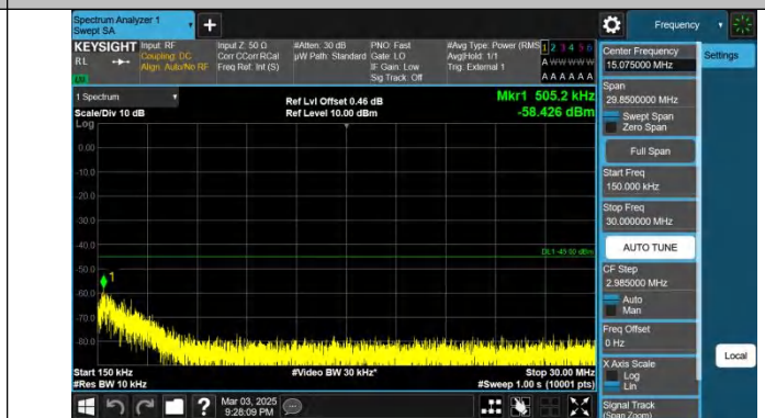
Band41-10MHz-QPSK-41540-1RB#0-0.15~30-PASS
